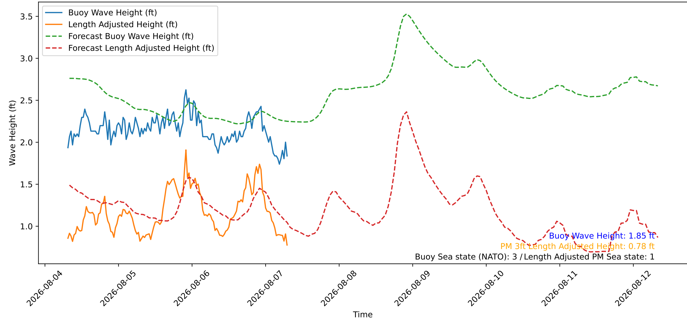
Wave Heights over Time for Green Beach at 2026-08-07 07:41:09
