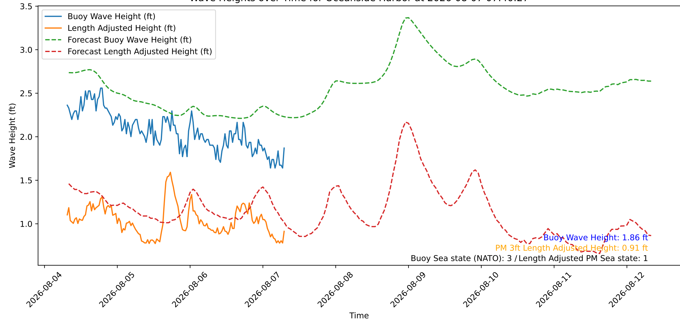
Wave Heights over Time for Oceanside Harbor at 2026-08-07 07:40:27
