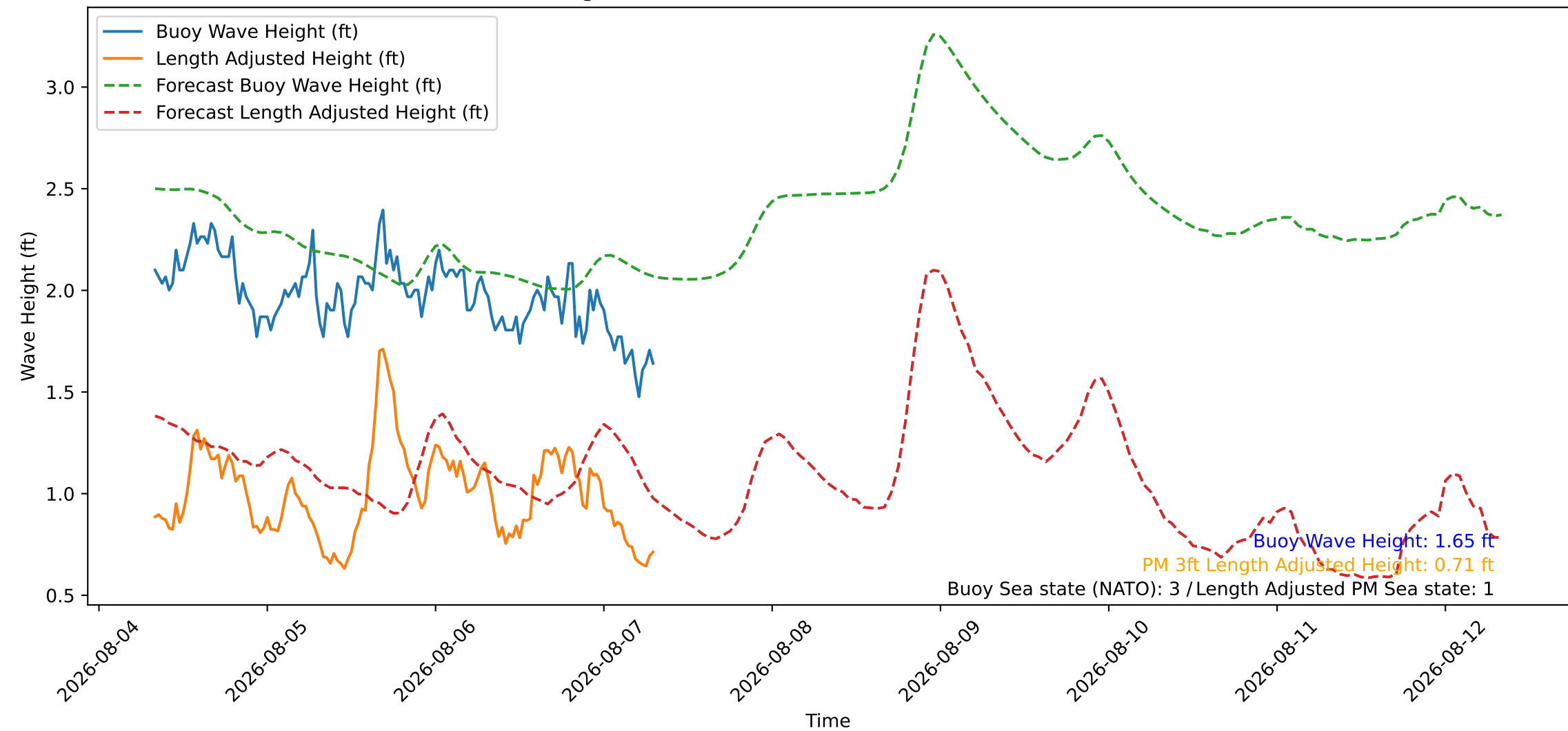
Wave Heights over Time for Red Beach at 2026-08-07 07:40:46
