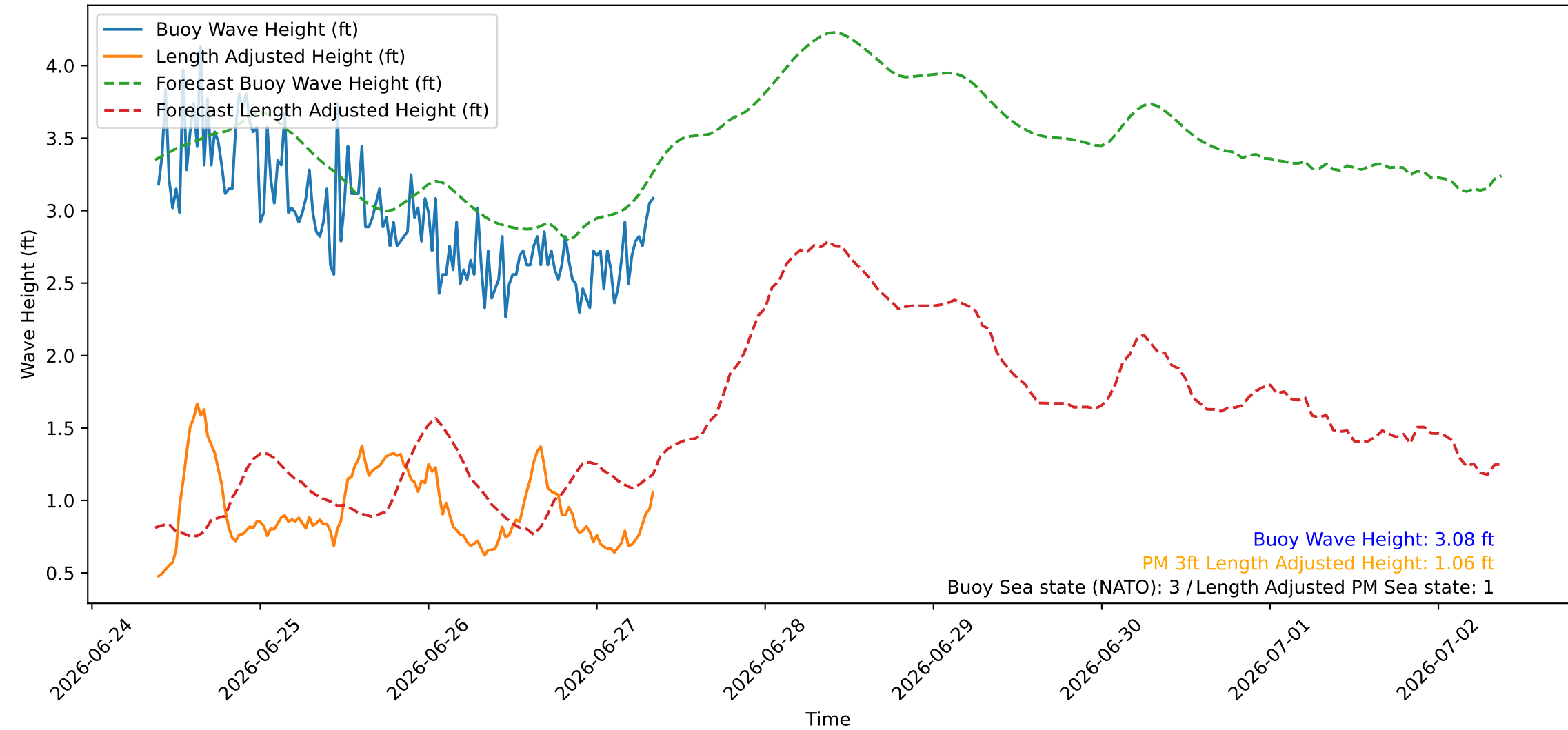
Wave Heights over Time for Red Beach at 2026-06-27 09:00:45
