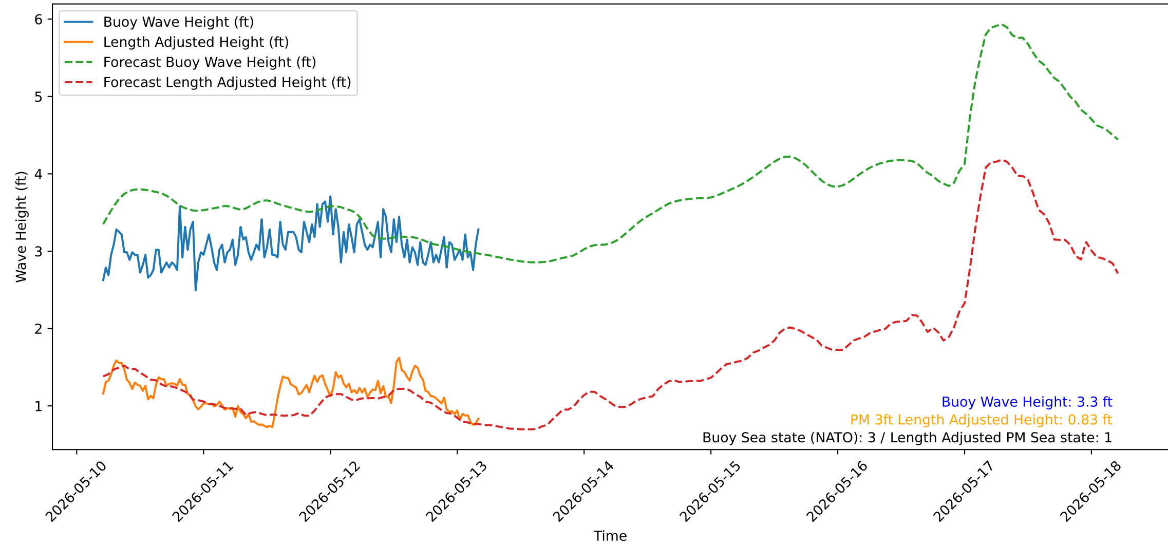
Wave Heights over Time for Oceanside Harbor at 2026-05-13 04:50:31
