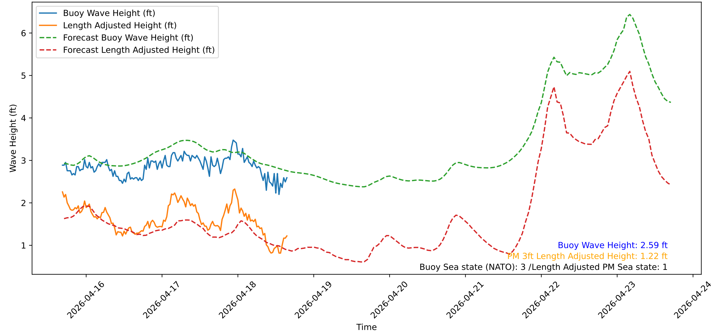
Wave Heights over Time for Green Beach at 2026-04-18 16:31:12
