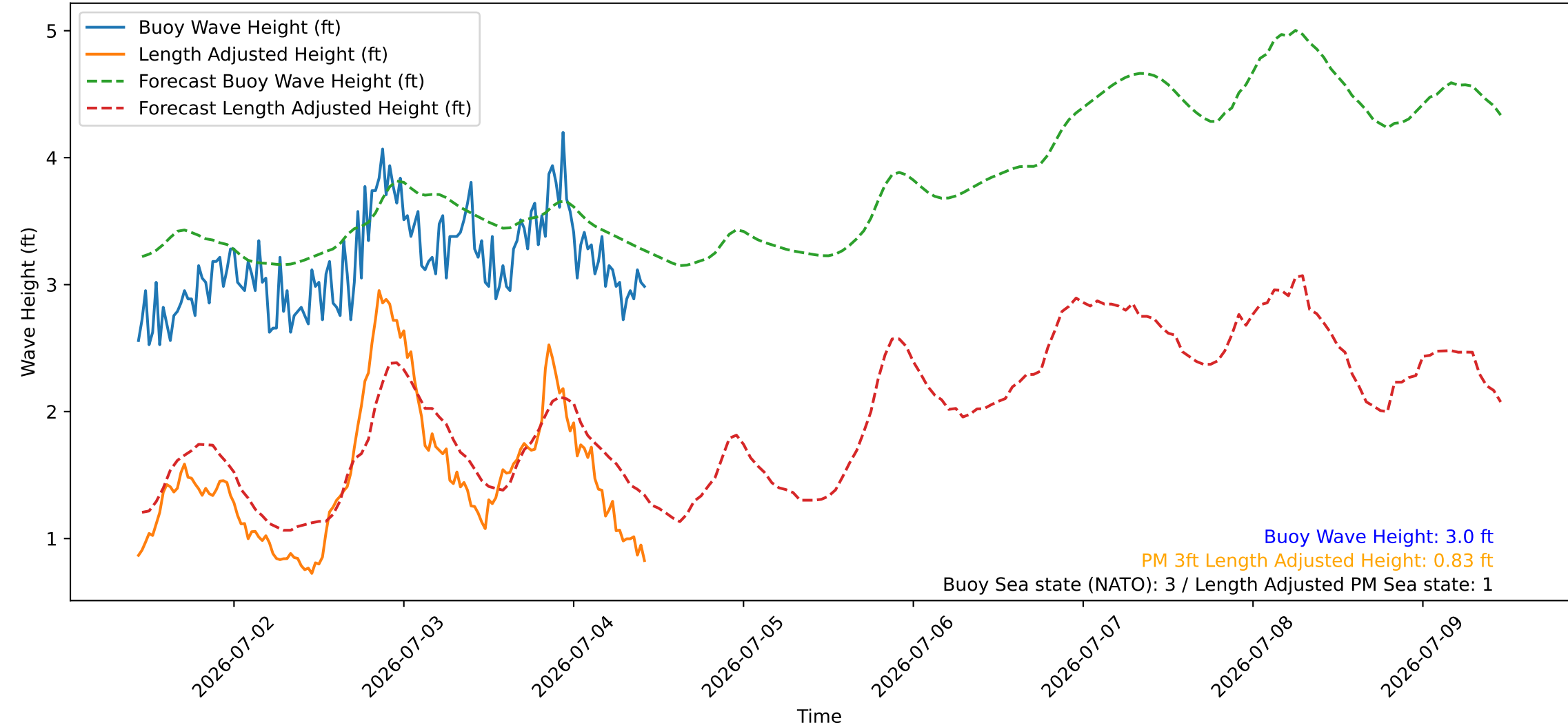
Wave Heights over Time for Green Beach at 2026-07-04 10:41:08
