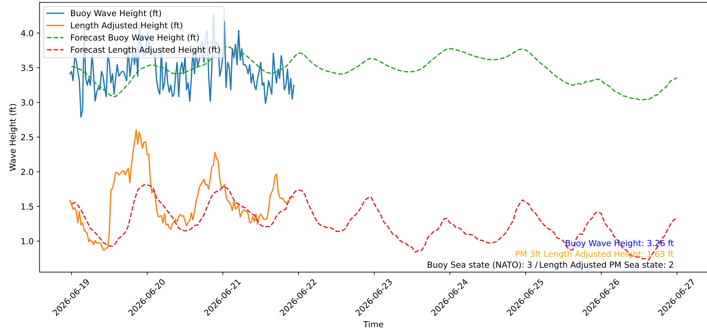
Wave Heights over Time for Oceanside Harbor at 2026-06-21 23:30:26
