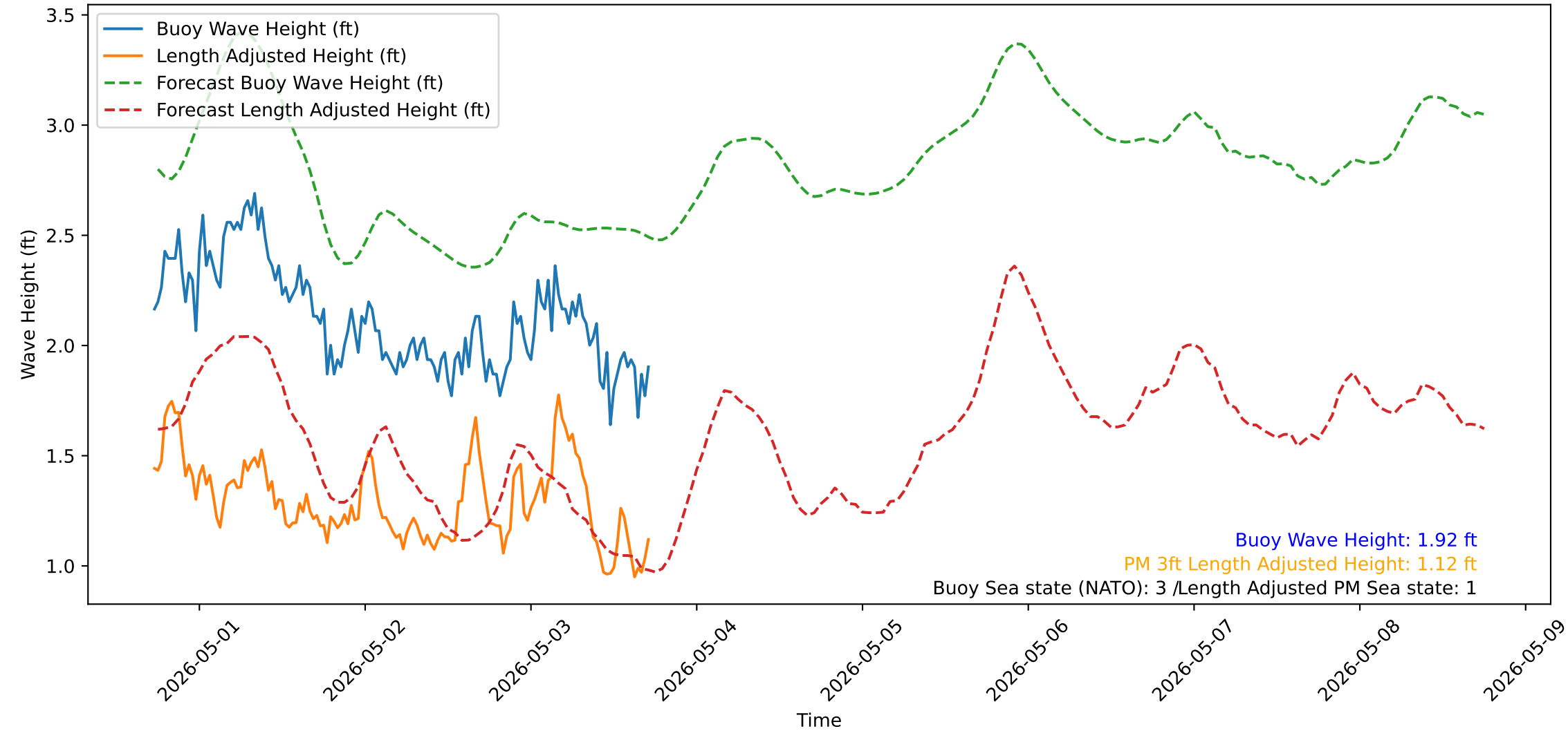
Wave Heights over Time for Oceanside Harbor at 2026-05-03 17:30:31
