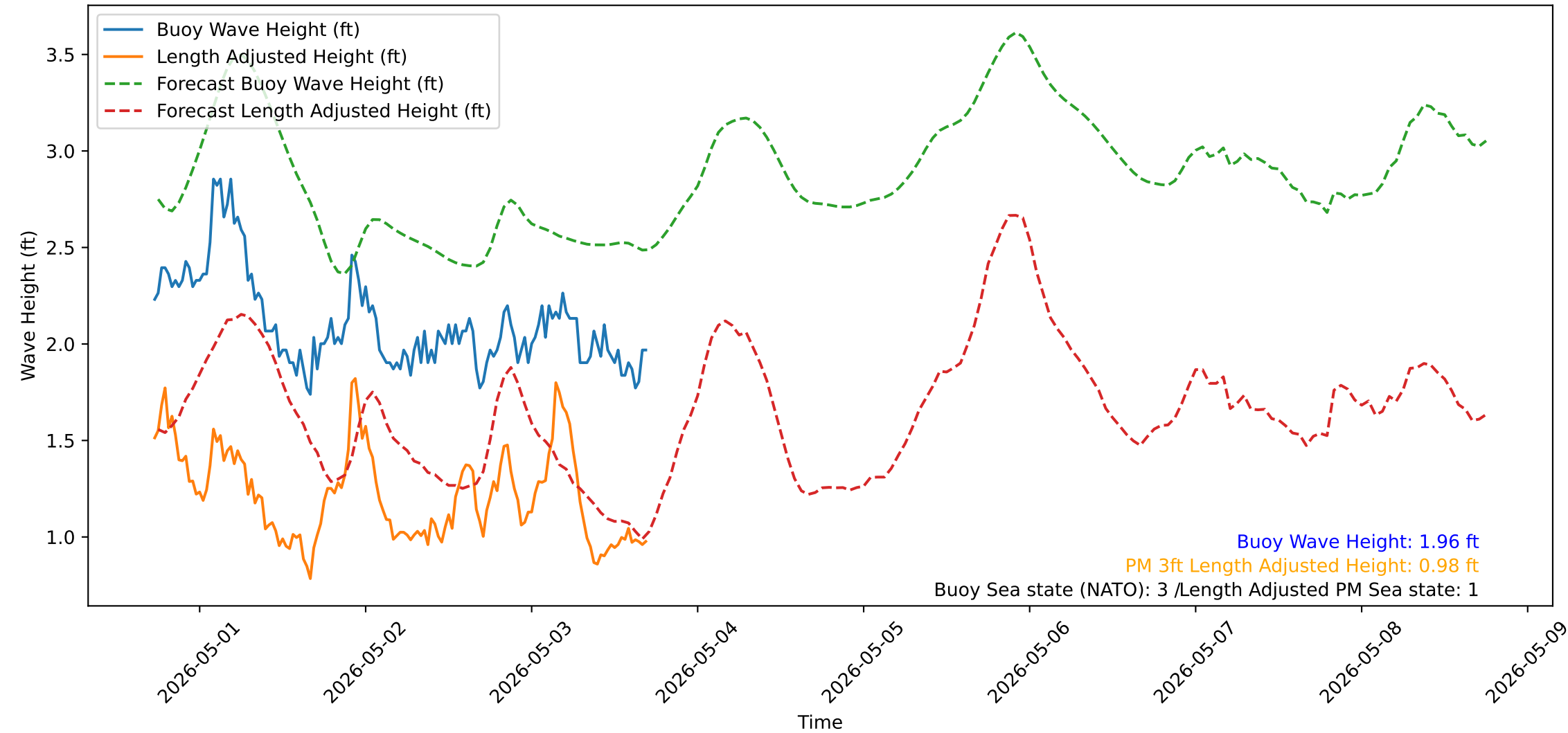
Wave Heights over Time for Green Beach at 2026-05-03 17:31:12
