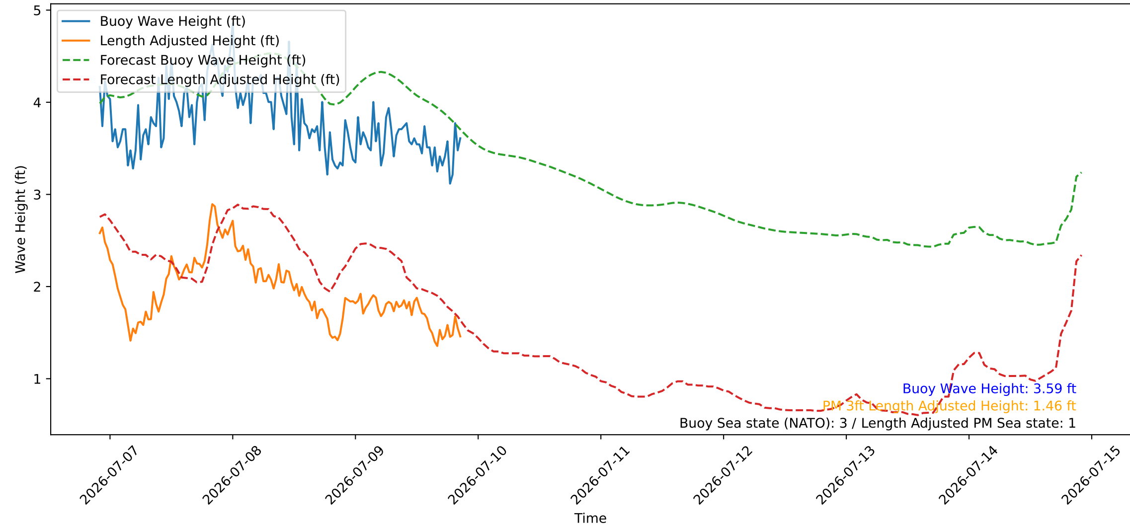
Wave Heights over Time for Red Beach at 2026-07-09 21:30:45
