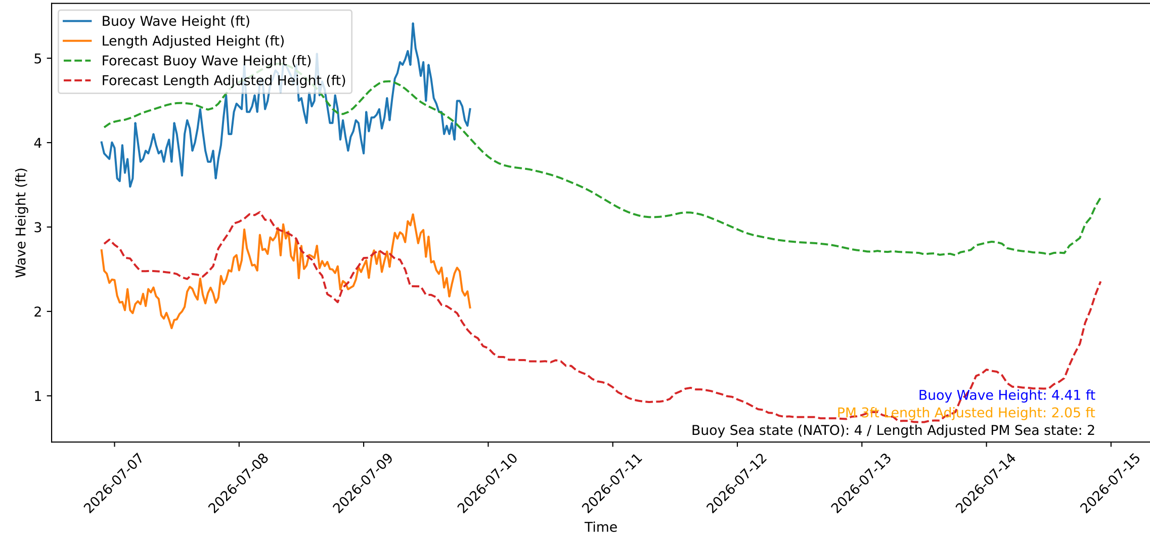
Wave Heights over Time for Oceanside Harbor at 2026-07-09 21:30:26
