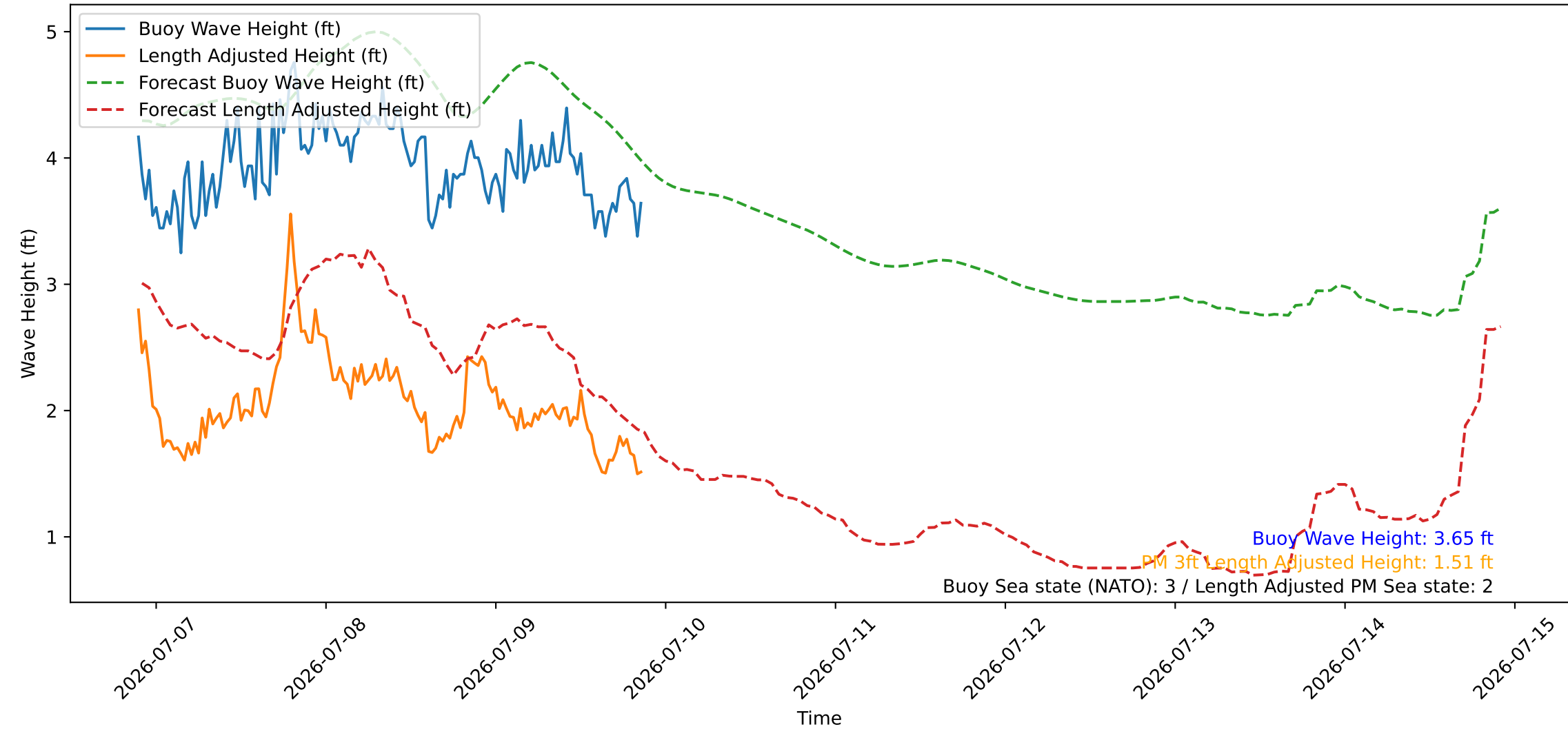
Wave Heights over Time for Green Beach at 2026-07-09 21:31:08
