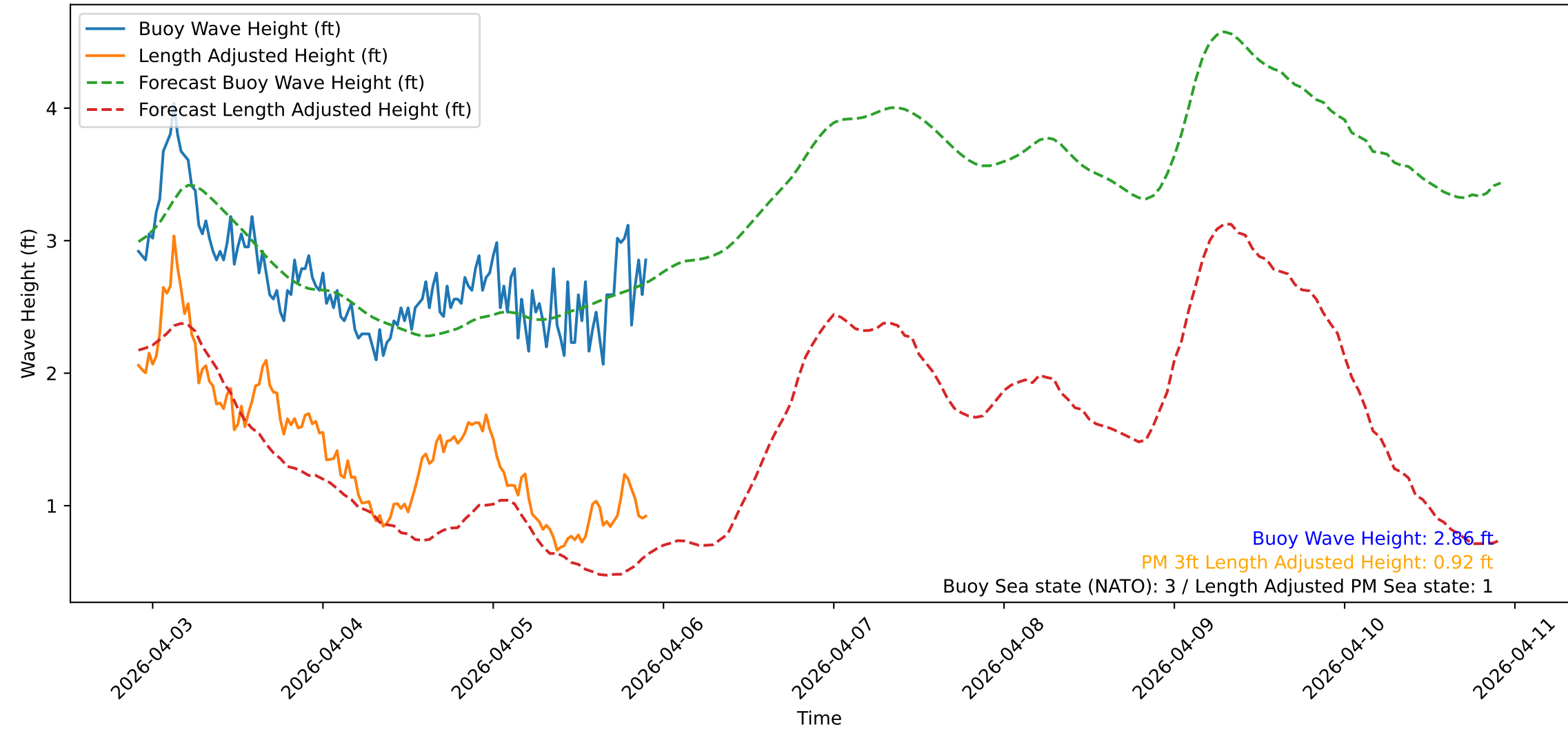
Wave Heights over Time for Oceanside Harbor at 2026-04-05 22:10:34
