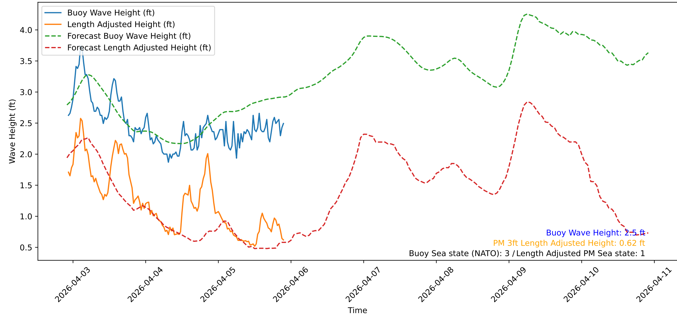
Wave Heights over Time for Red Beach at 2026-04-05 22:10:53
