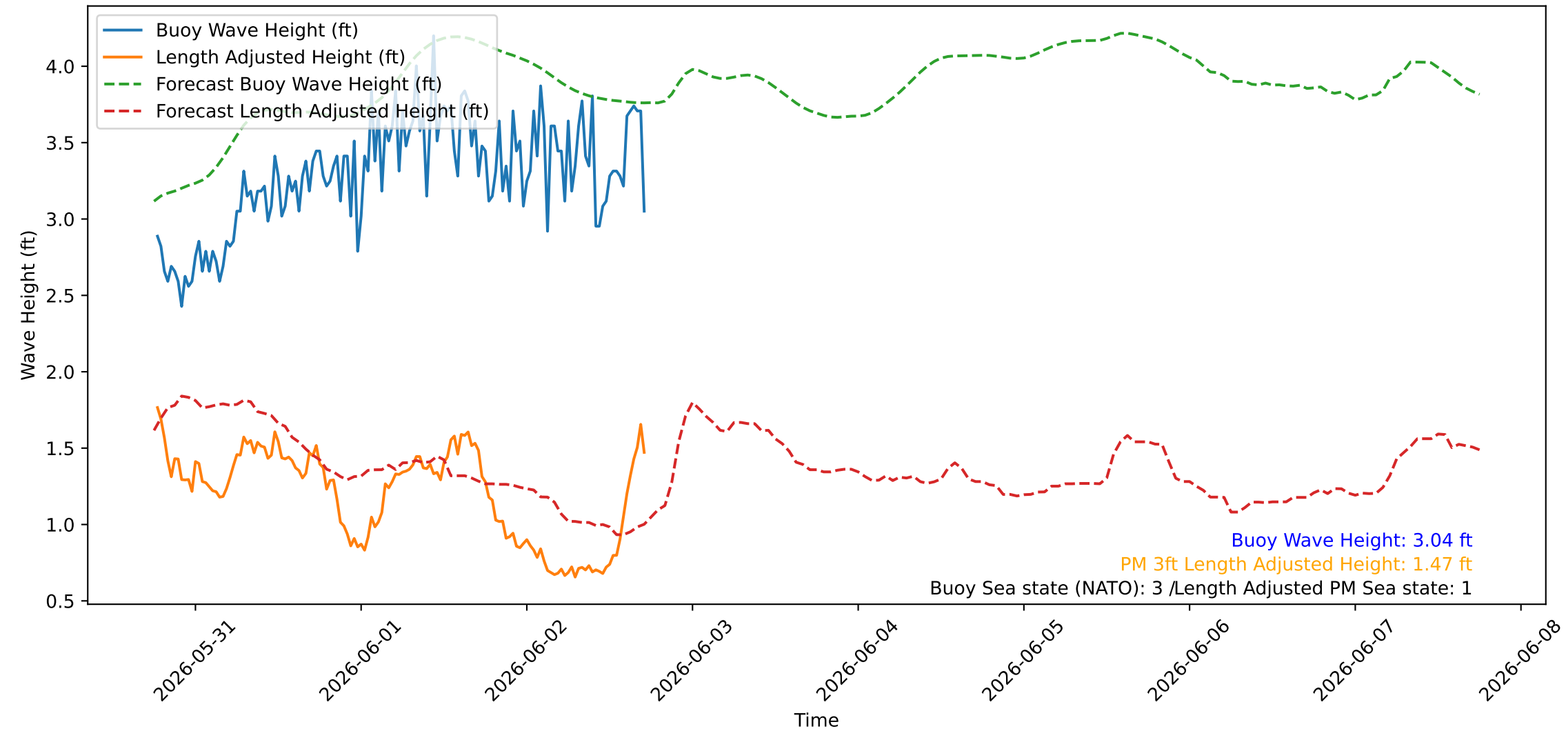
Wave Heights over Time for Red Beach at 2026-06-02 18:00:46
