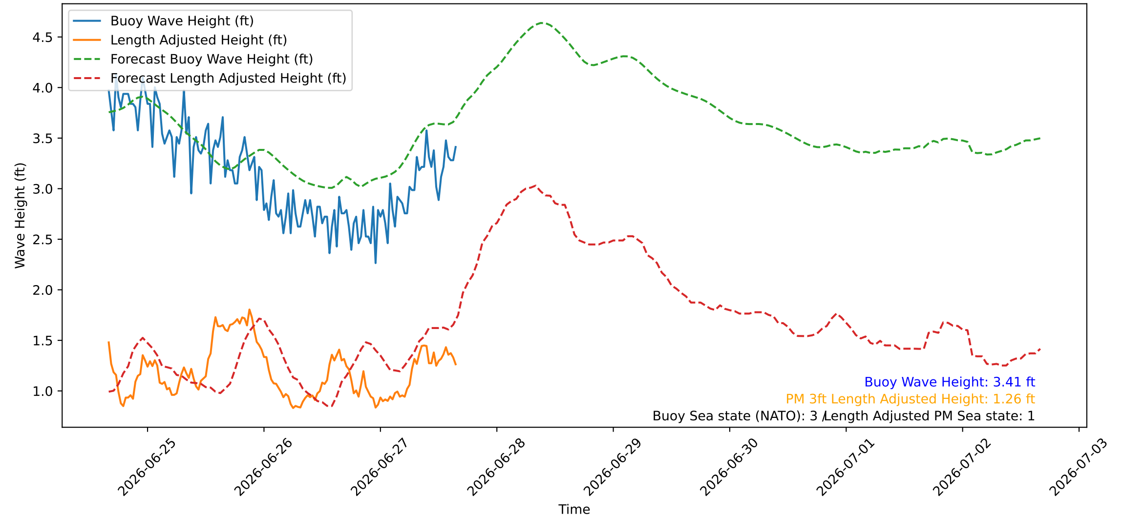
Wave Heights over Time for Green Beach at 2026-06-27 16:11:08
