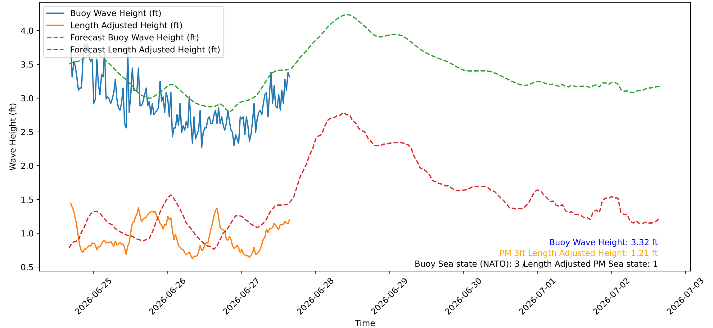
Wave Heights over Time for Red Beach at 2026-06-27 16:10:46
