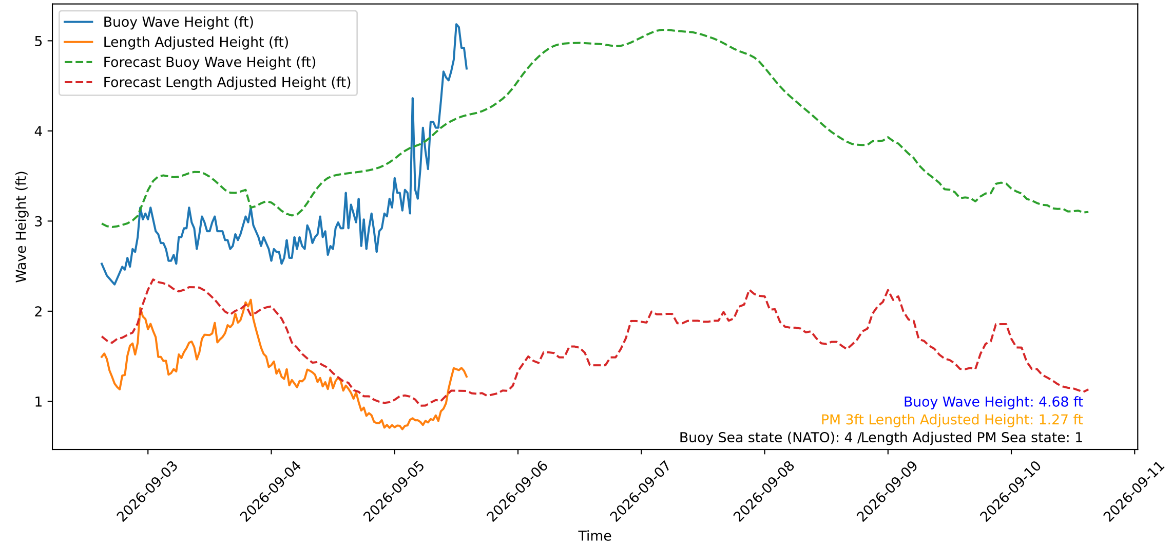
Wave Heights over Time for Red Beach at 2026-09-05 14:50:52
