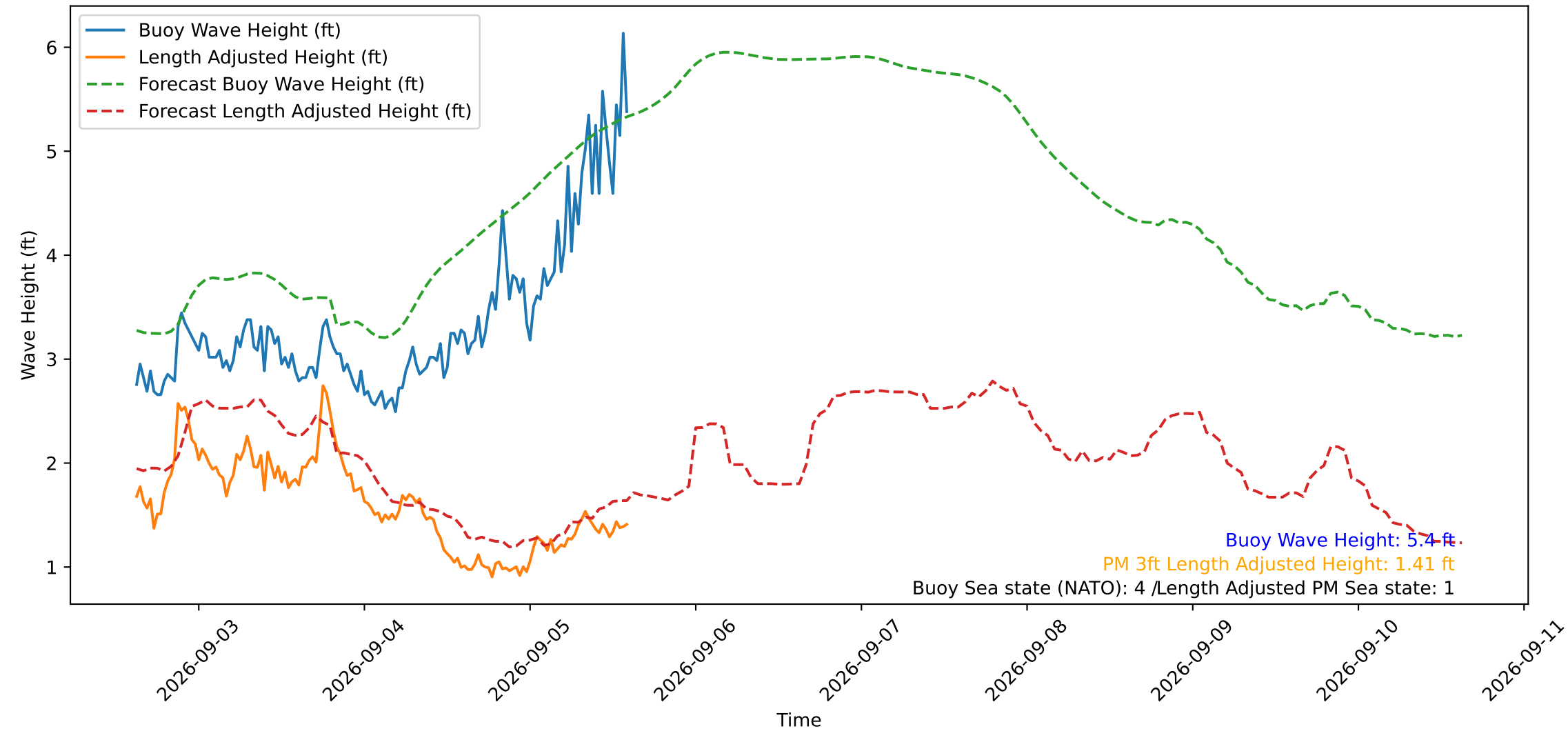
Wave Heights over Time for Green Beach at 2026-09-05 14:51:15
