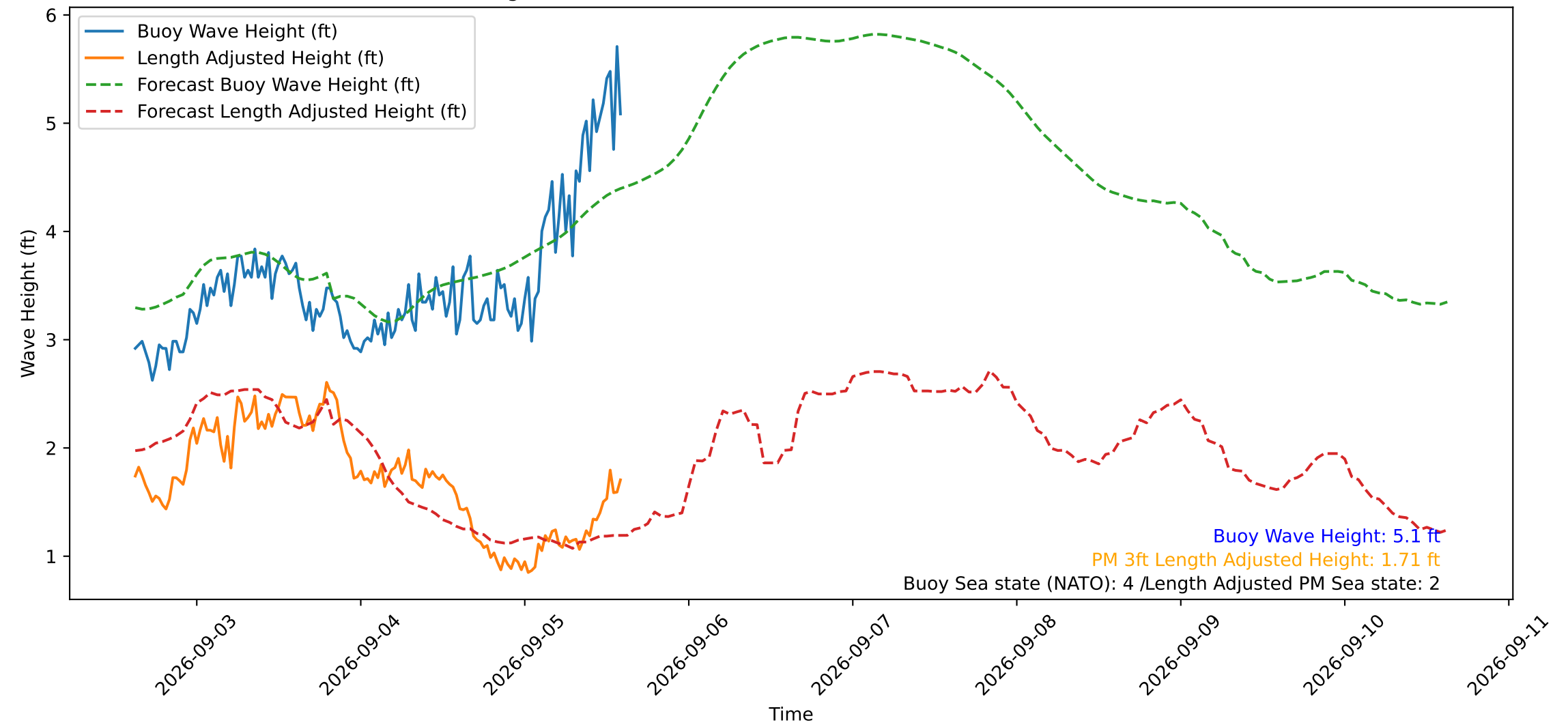
Wave Heights over Time for Oceanside Harbor at 2026-09-05 14:50:30
