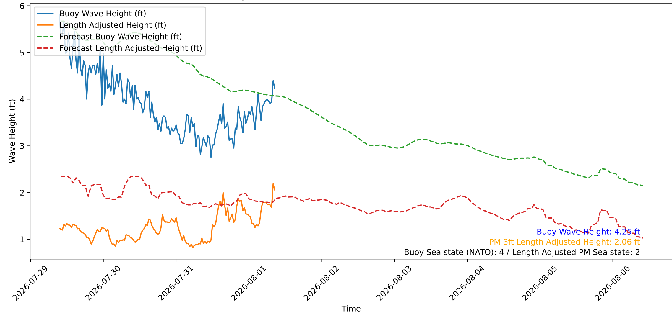
Wave Heights over Time for Green Beach at 2026-08-01 09:31:07
