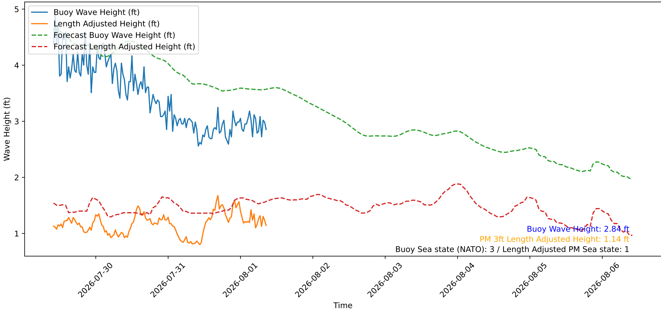
Wave Heights over Time for Red Beach at 2026-08-01 09:30:45
