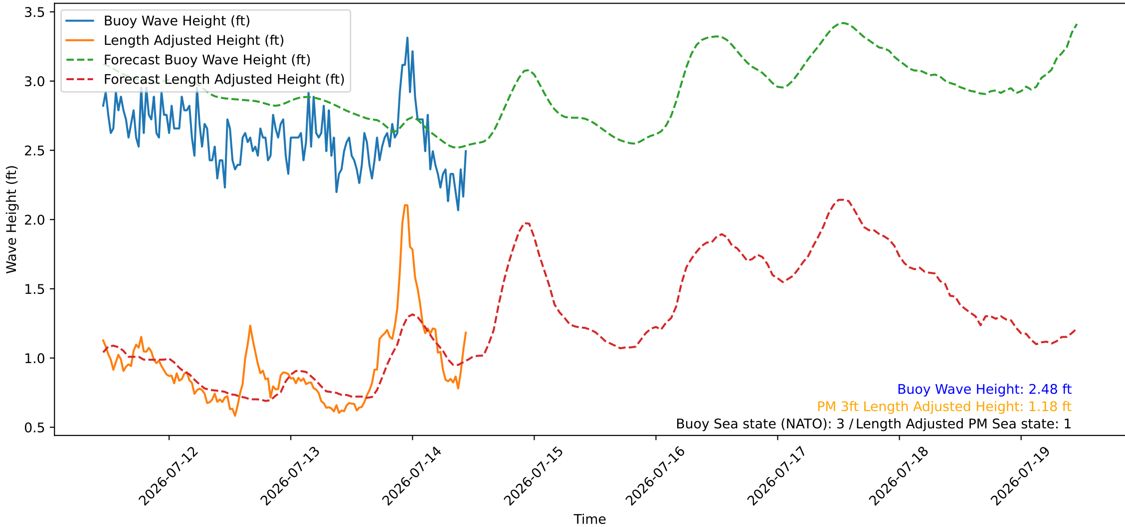
Wave Heights over Time for Green Beach at 2026-07-14 11:11:09
