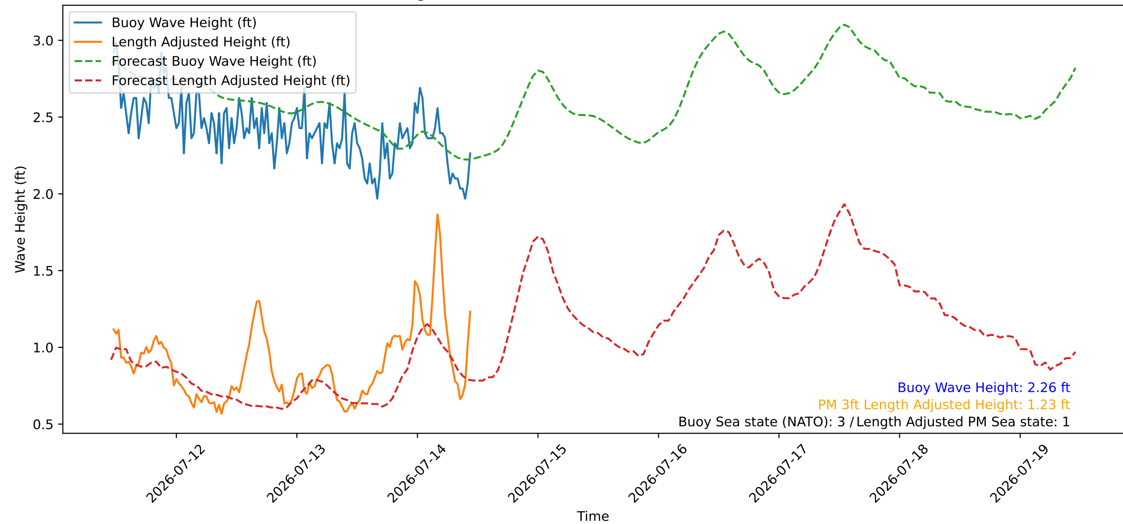
Wave Heights over Time for Red Beach at 2026-07-14 11:10:46
