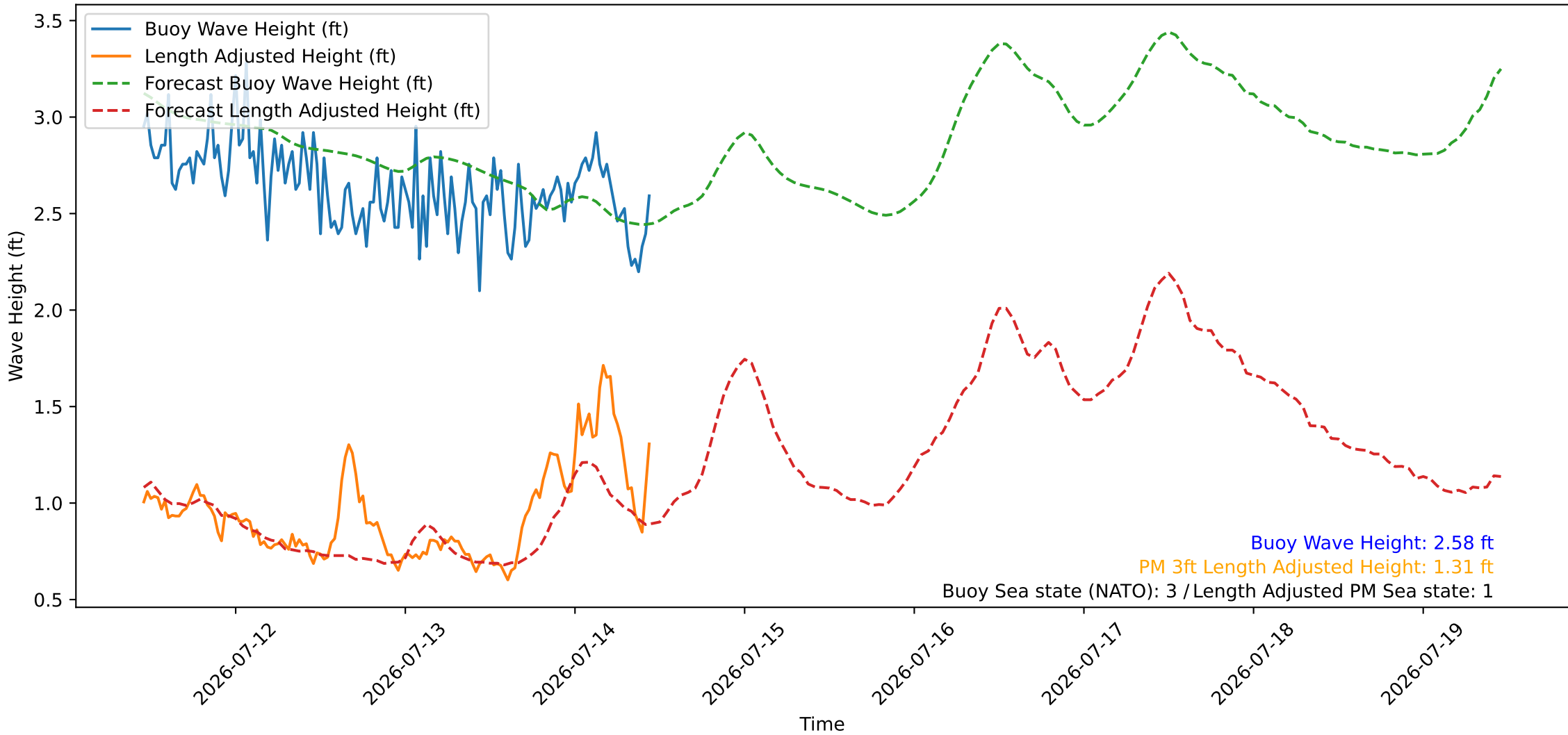
Wave Heights over Time for Oceanside Harbor at 2026-07-14 11:10:26
