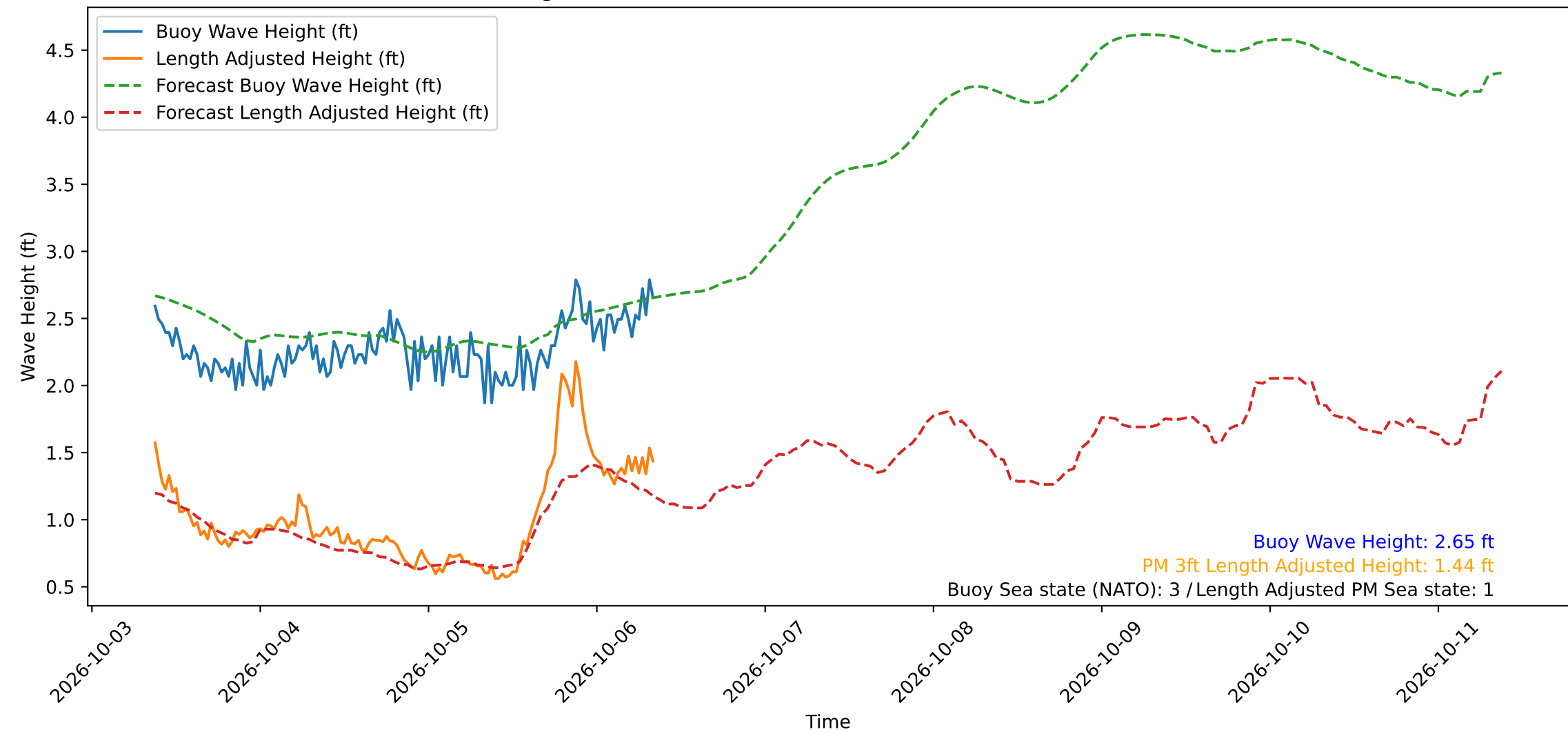
Wave Heights over Time for Oceanside Harbor at 2026-10-06 08:50:30
