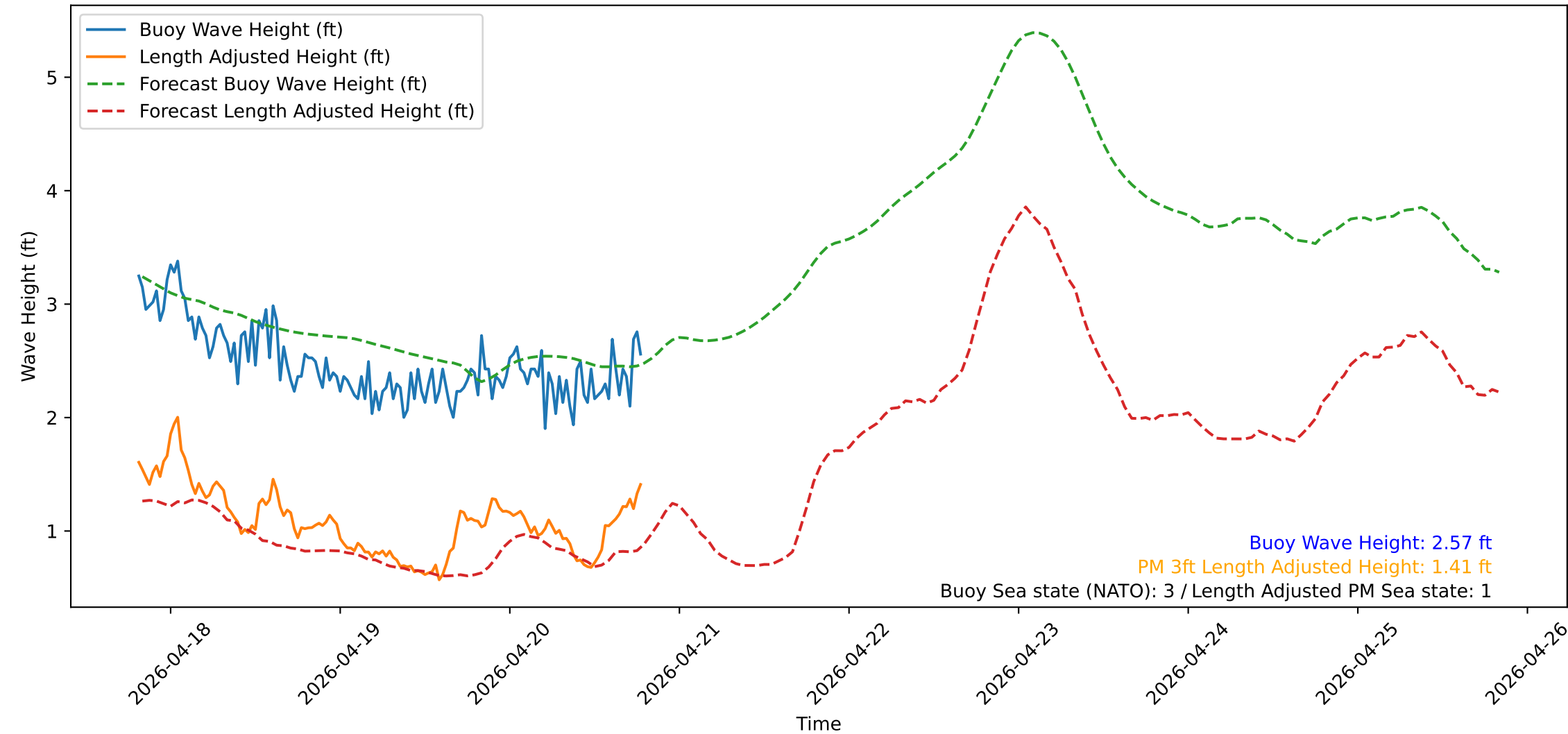
Wave Heights over Time for Oceanside Harbor at 2026-04-20 19:40:32
