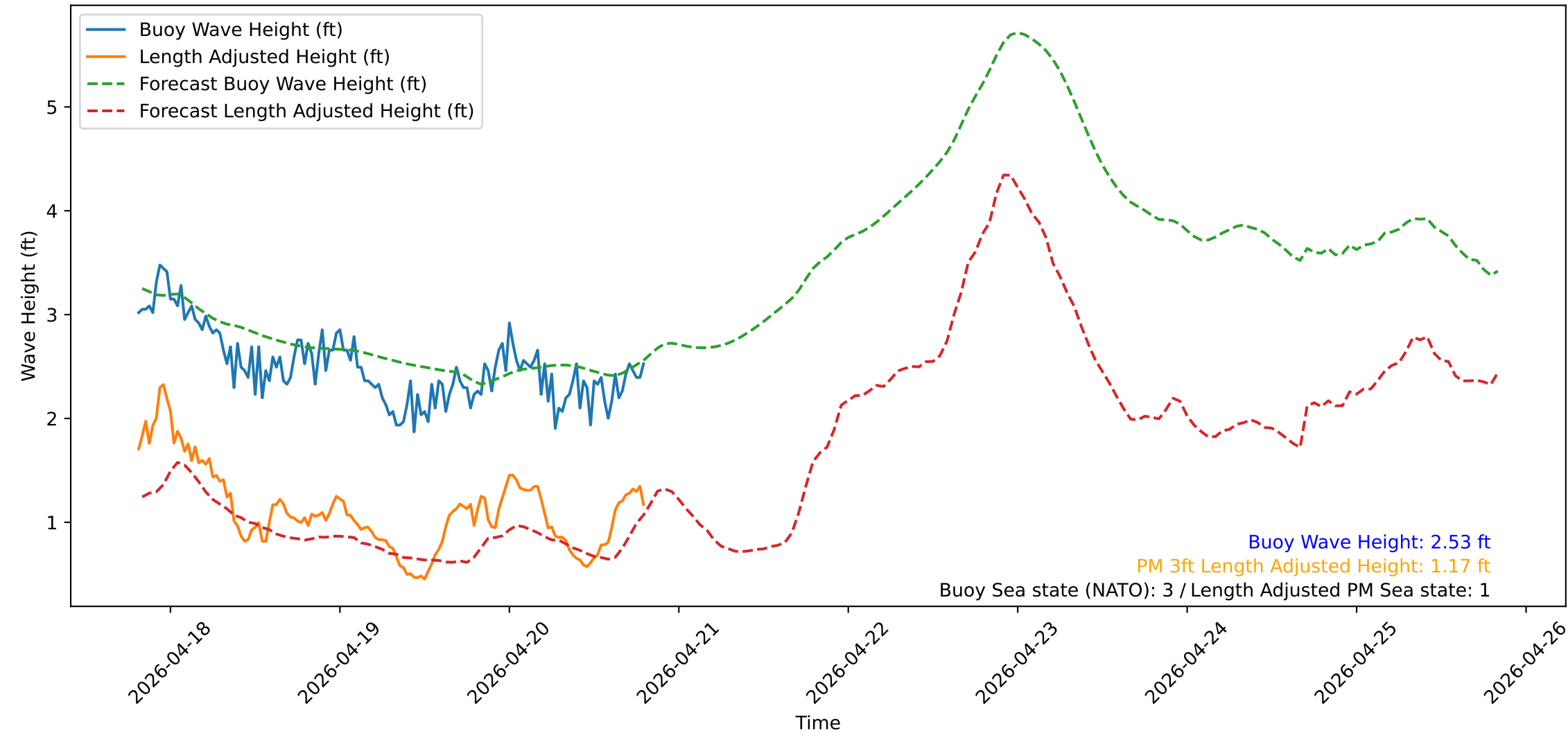
Wave Heights over Time for Green Beach at 2026-04-20 19:41:13
