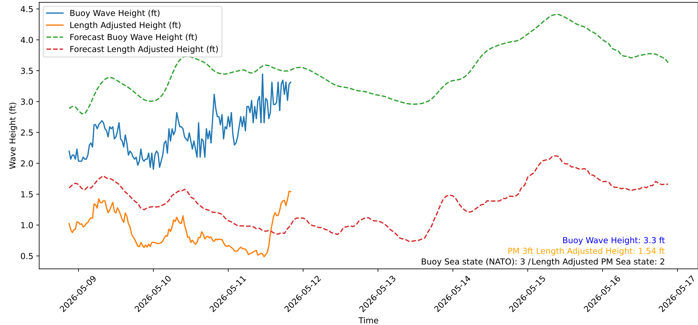
Wave Heights over Time for Green Beach at 2026-05-11 20:51:14
