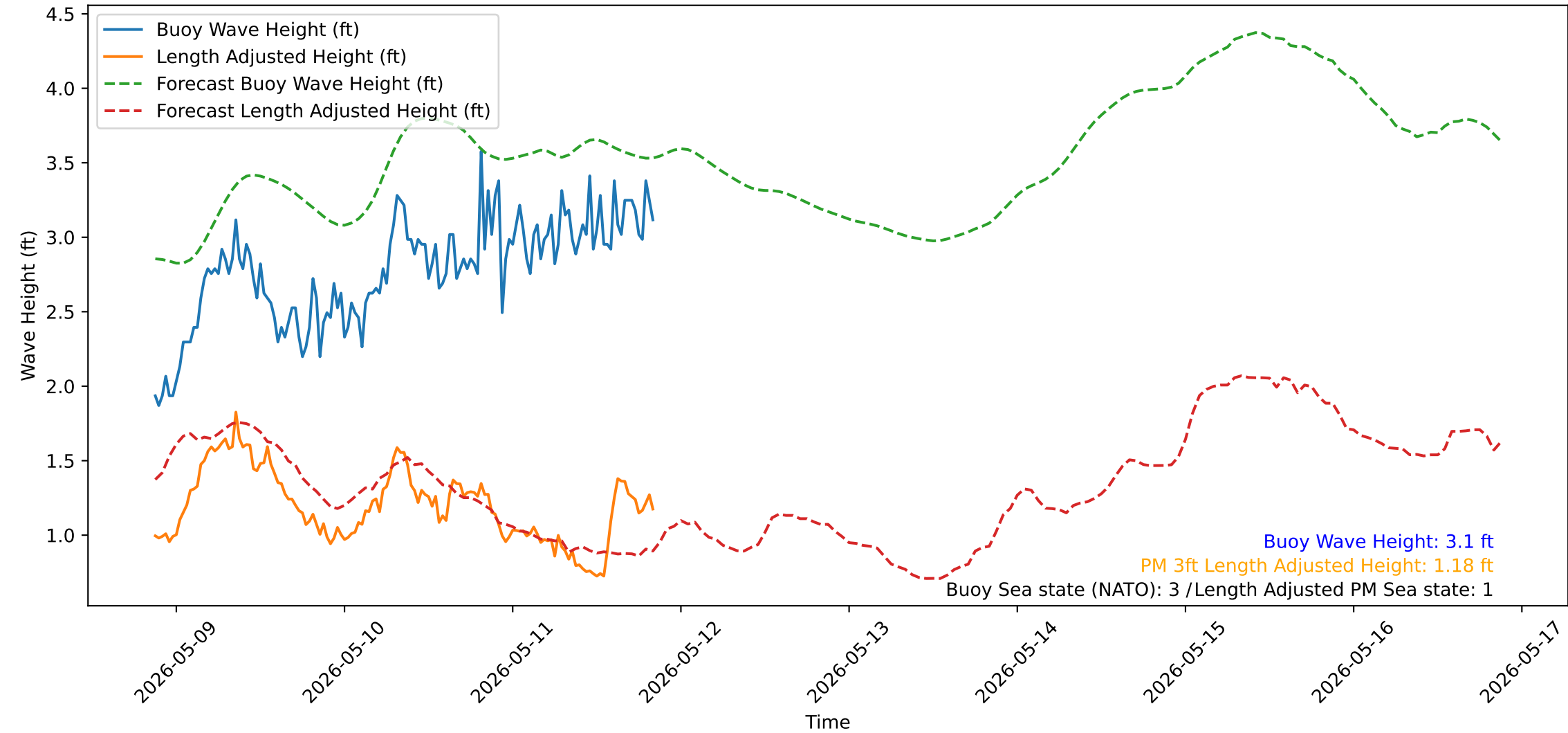
Wave Heights over Time for Oceanside Harbor at 2026-05-11 20:50:31
