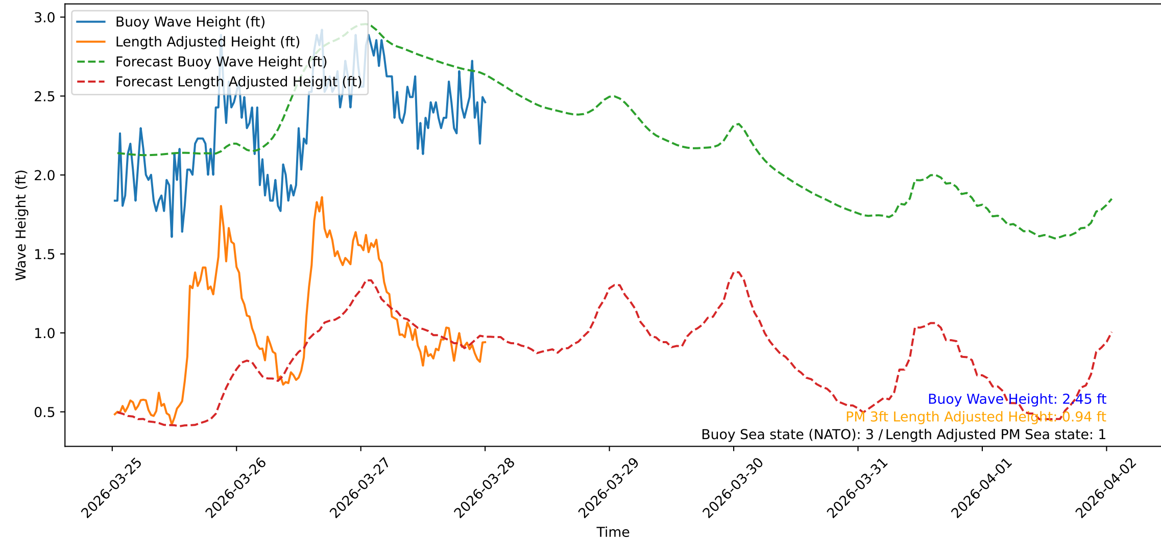
Wave Heights over Time for Oceanside Harbor at 2026-03-28 00:40:32
