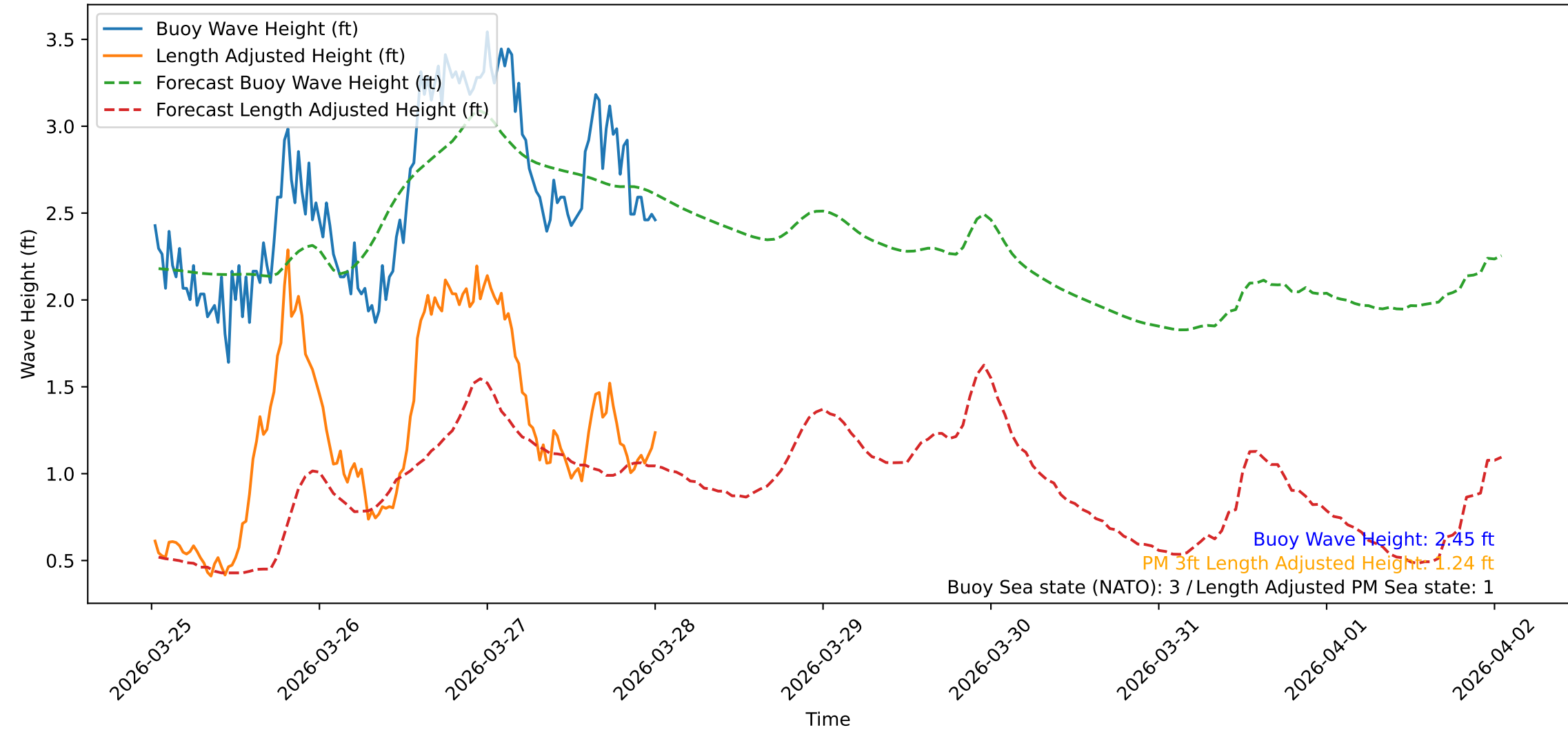
Wave Heights over Time for Green Beach at 2026-03-28 00:41:10
