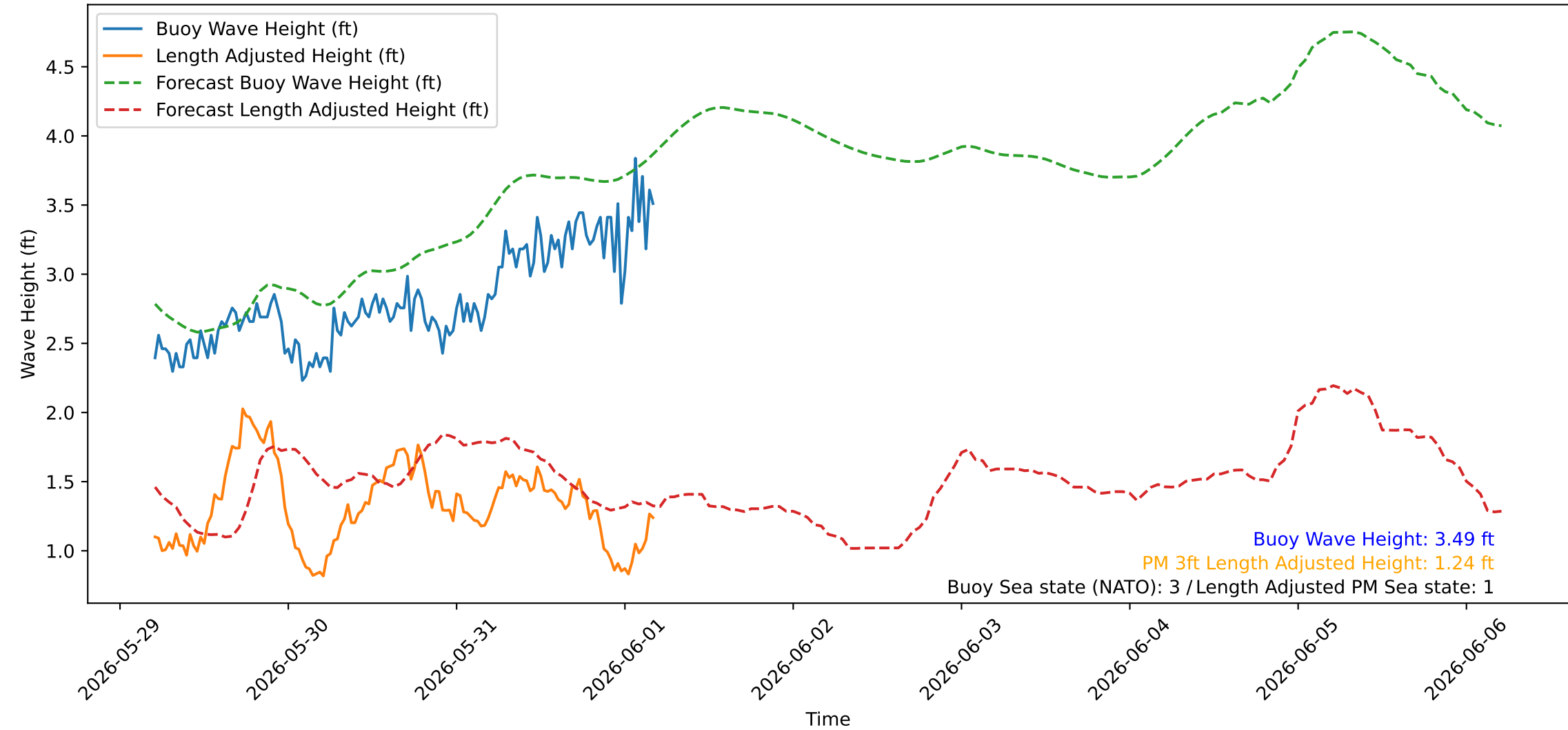
Wave Heights over Time for Red Beach at 2026-06-01 04:40:45
