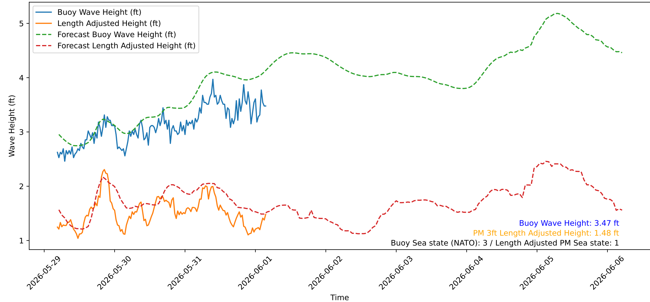
Wave Heights over Time for Green Beach at 2026-06-01 04:41:07
