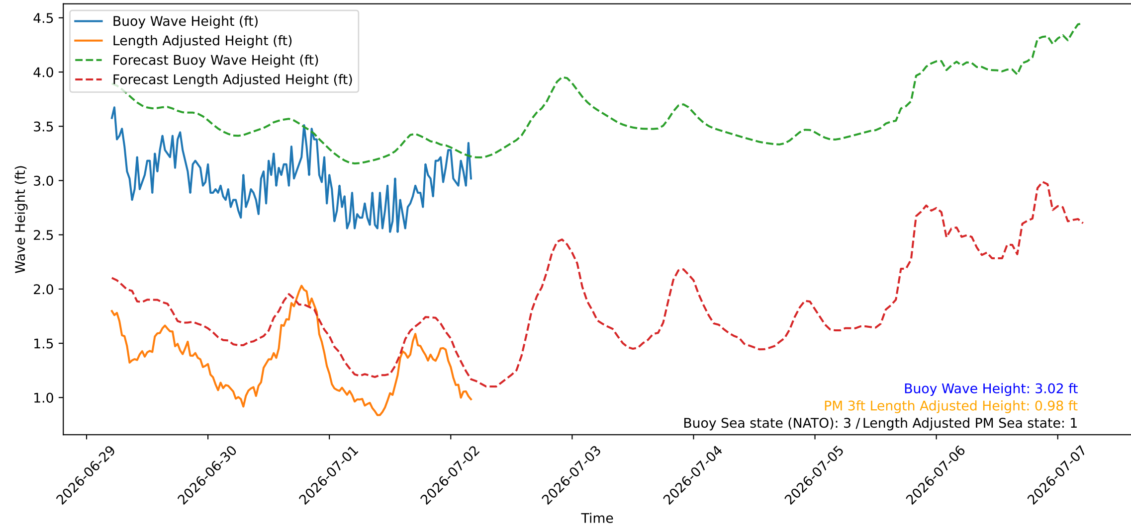
Wave Heights over Time for Green Beach at 2026-07-02 05:01:08
