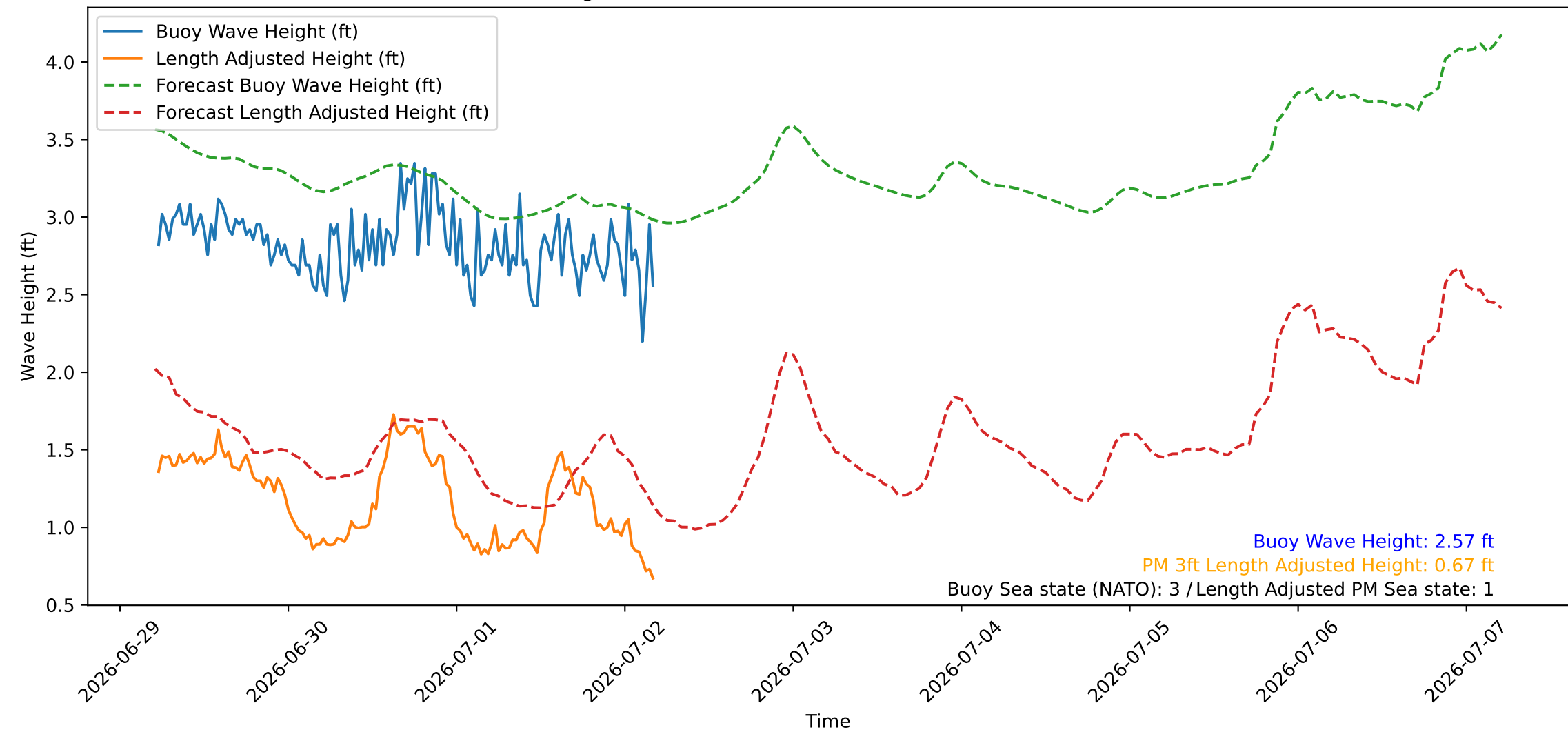
Wave Heights over Time for Red Beach at 2026-07-02 05:00:46
