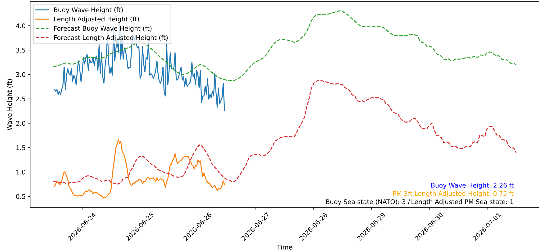
Wave Heights over Time for Red Beach at 2026-06-26 12:10:45
