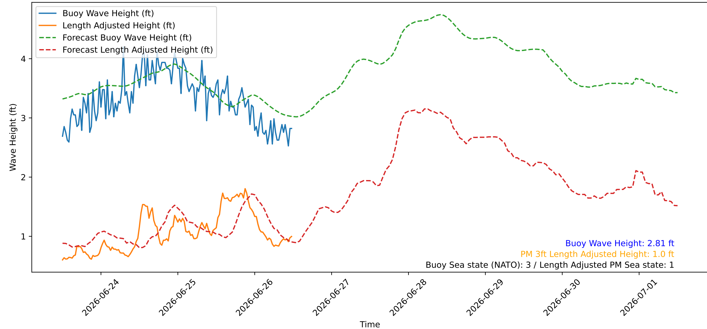
Wave Heights over Time for Green Beach at 2026-06-26 12:11:08
