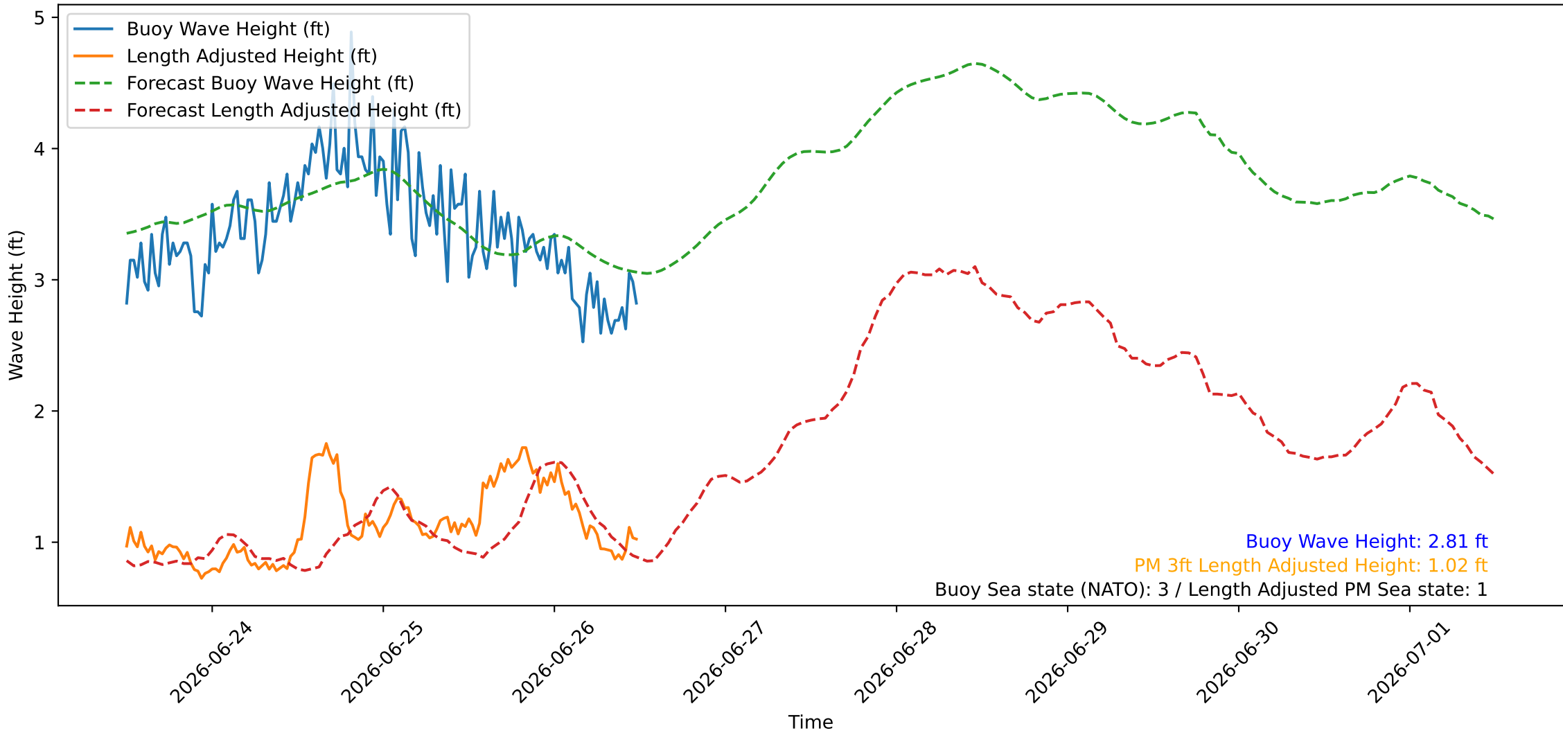
Wave Heights over Time for Oceanside Harbor at 2026-06-26 12:10:26
