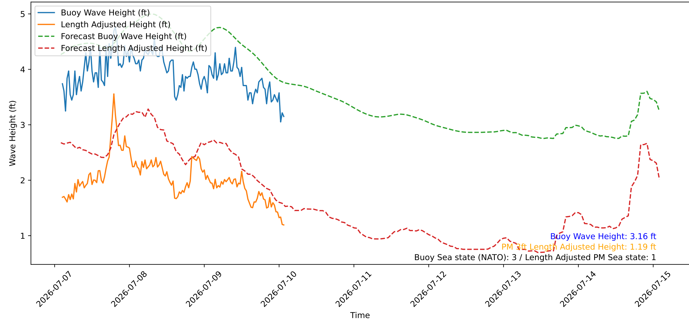
Wave Heights over Time for Green Beach at 2026-07-10 02:21:09
