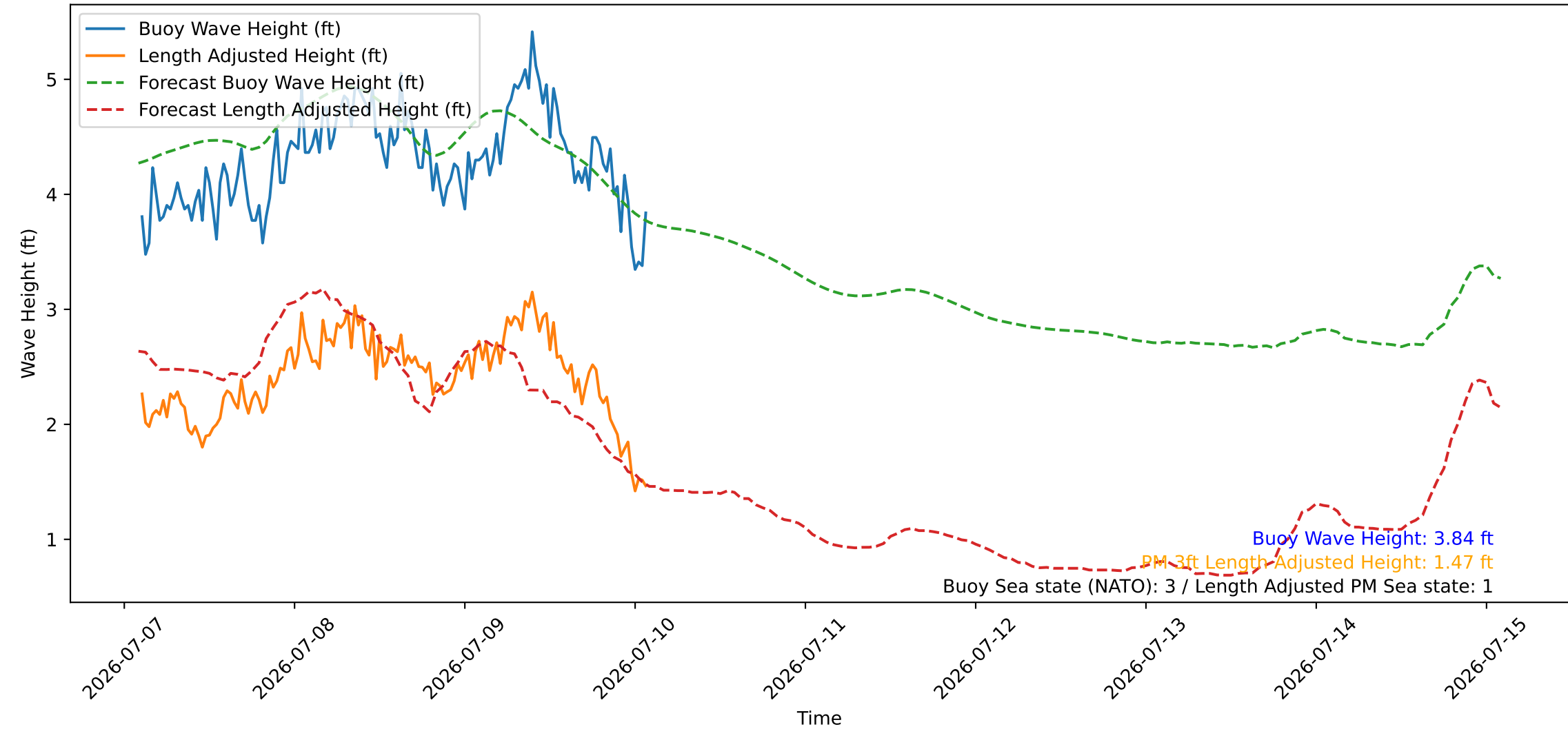
Wave Heights over Time for Oceanside Harbor at 2026-07-10 02:20:26
