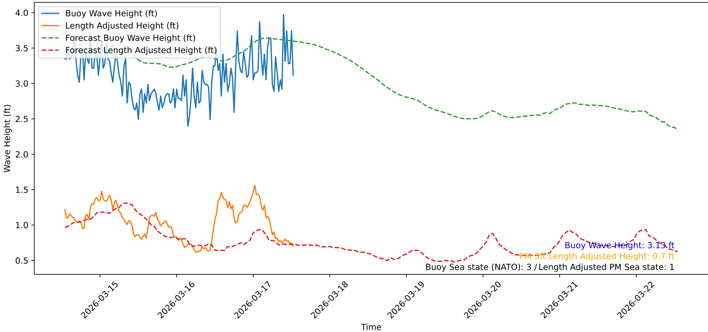
Wave Heights over Time for Oceanside Harbor at 2026-03-17 13:10:42
