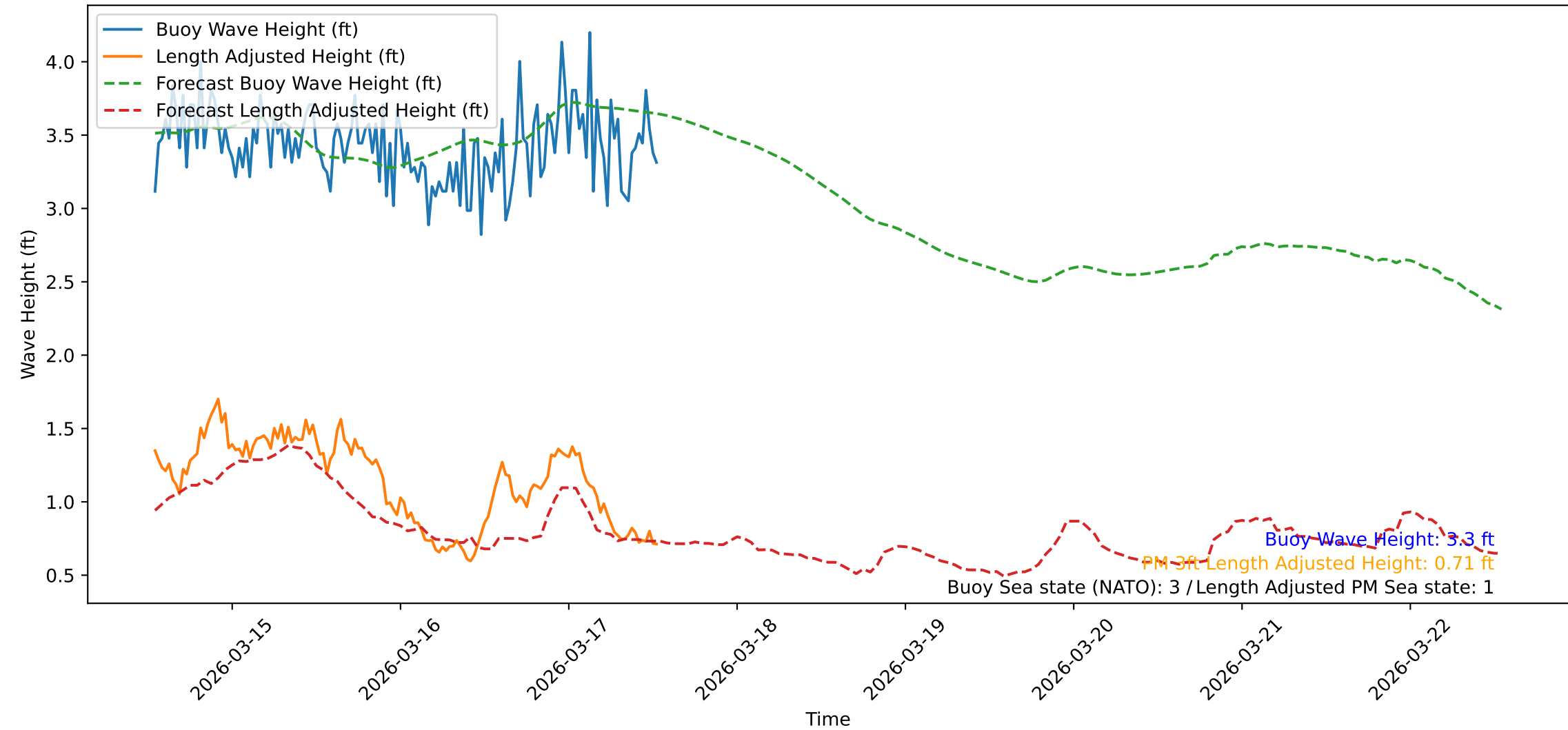
Wave Heights over Time for Green Beach at 2026-03-17 13:11:40
