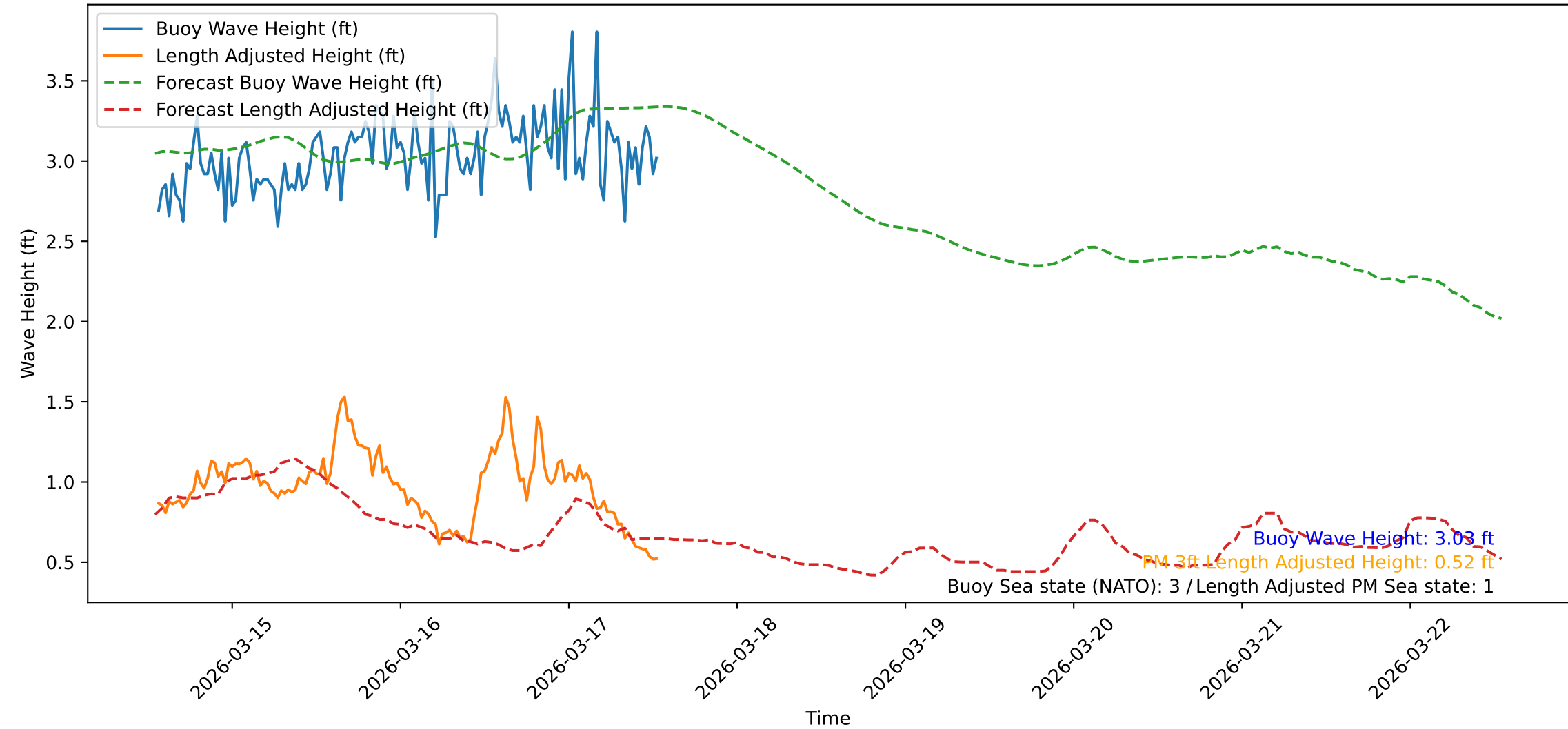
Wave Heights over Time for Red Beach at 2026-03-17 13:11:04
