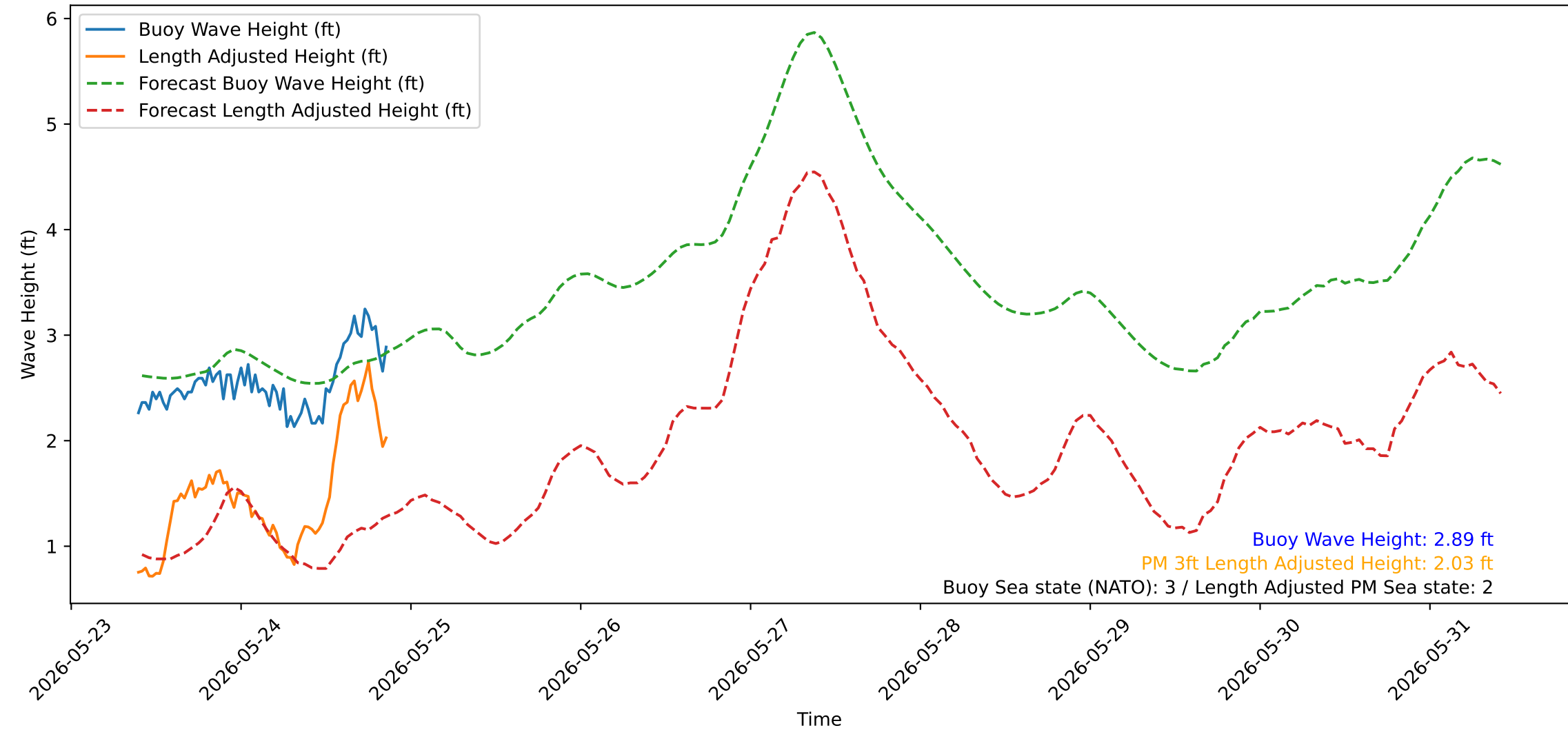
Wave Heights over Time for Oceanside Harbor at 2026-05-26 09:40:28
