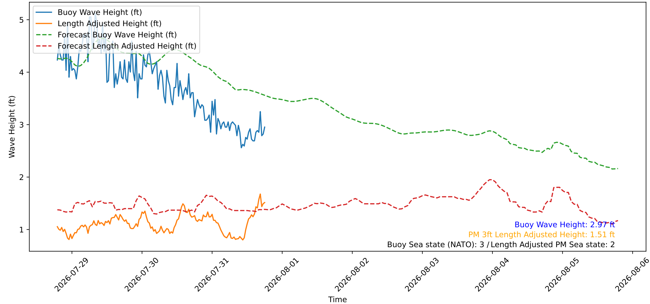
Wave Heights over Time for Red Beach at 2026-07-31 18:50:47
