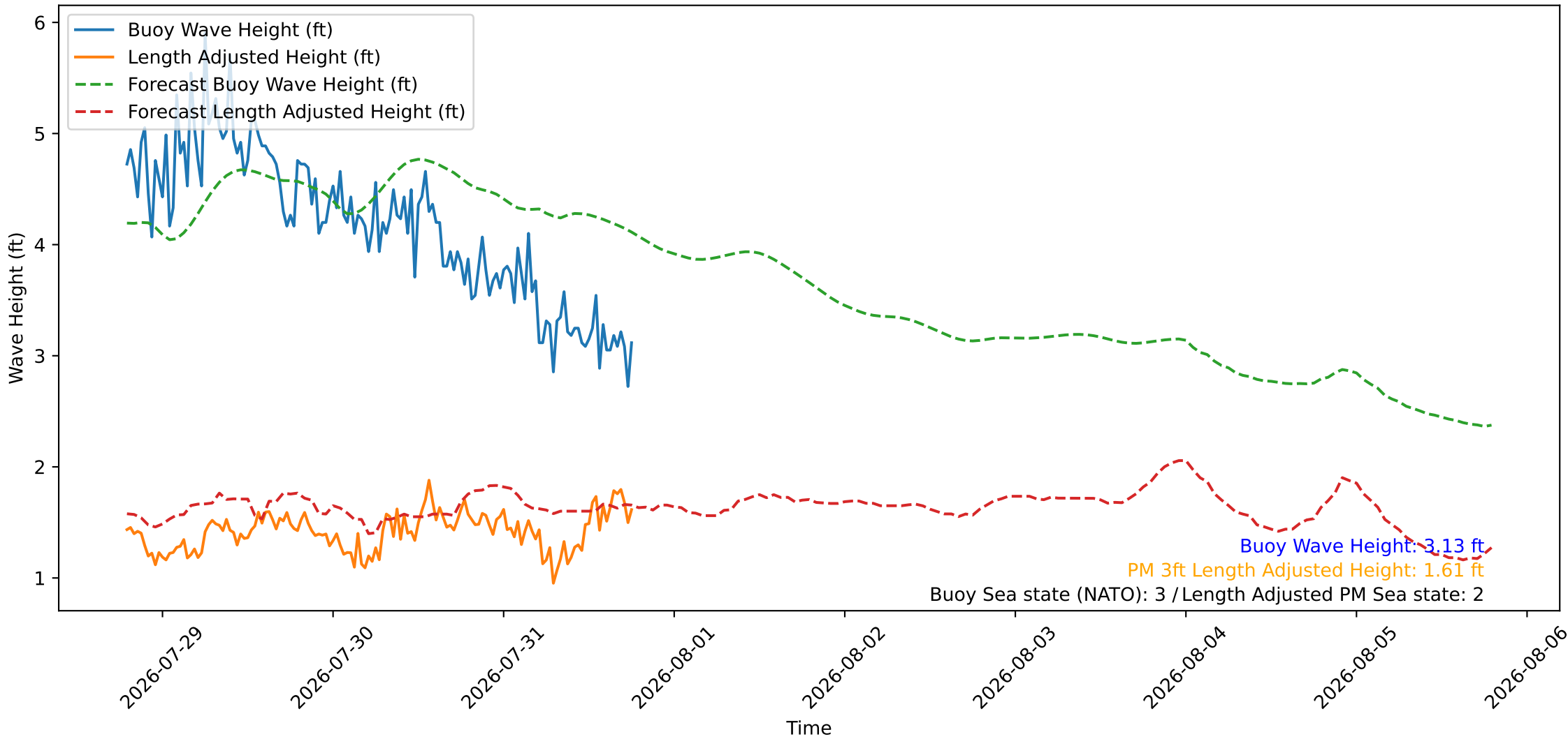
Wave Heights over Time for Oceanside Harbor at 2026-07-31 18:50:27
