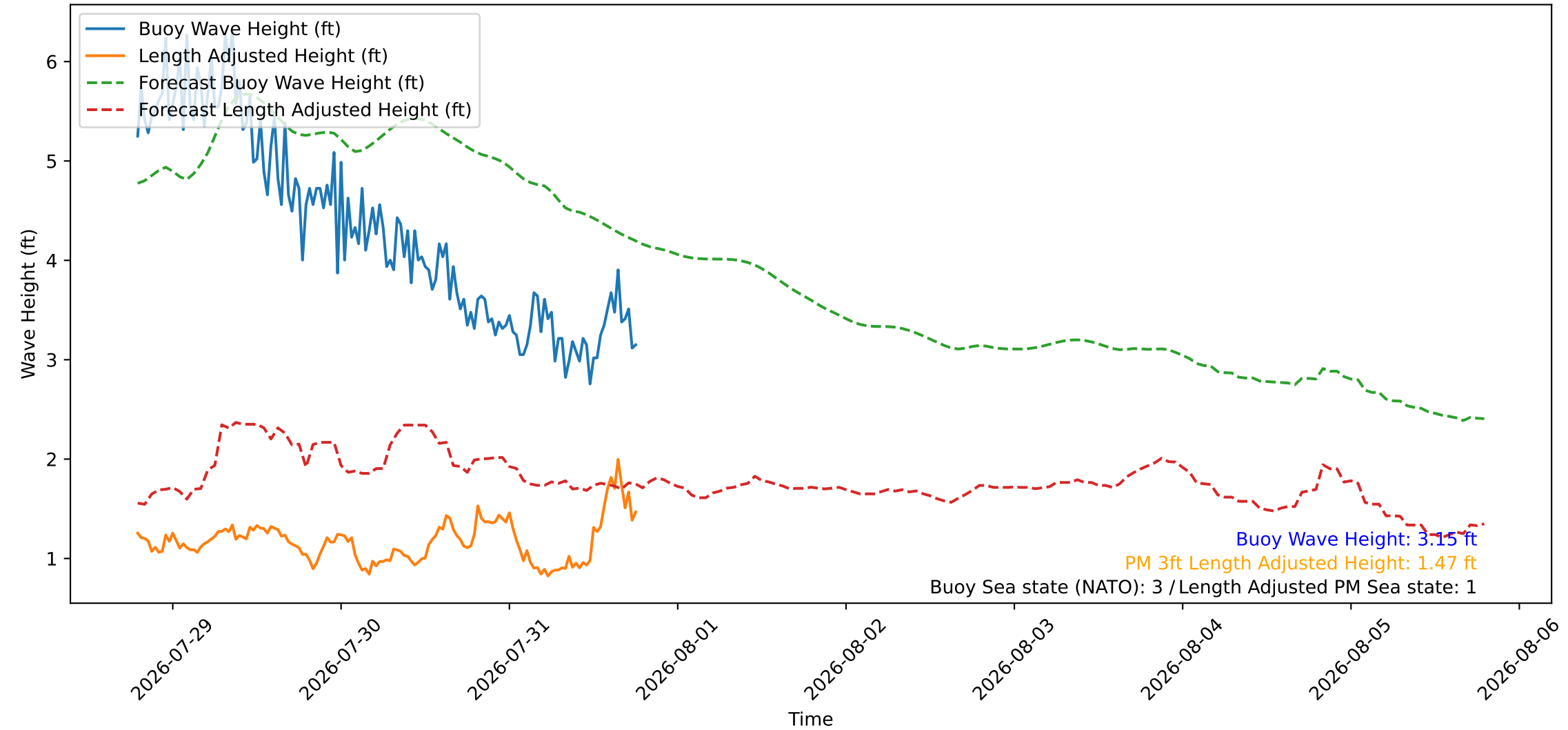
Wave Heights over Time for Green Beach at 2026-07-31 18:51:10
