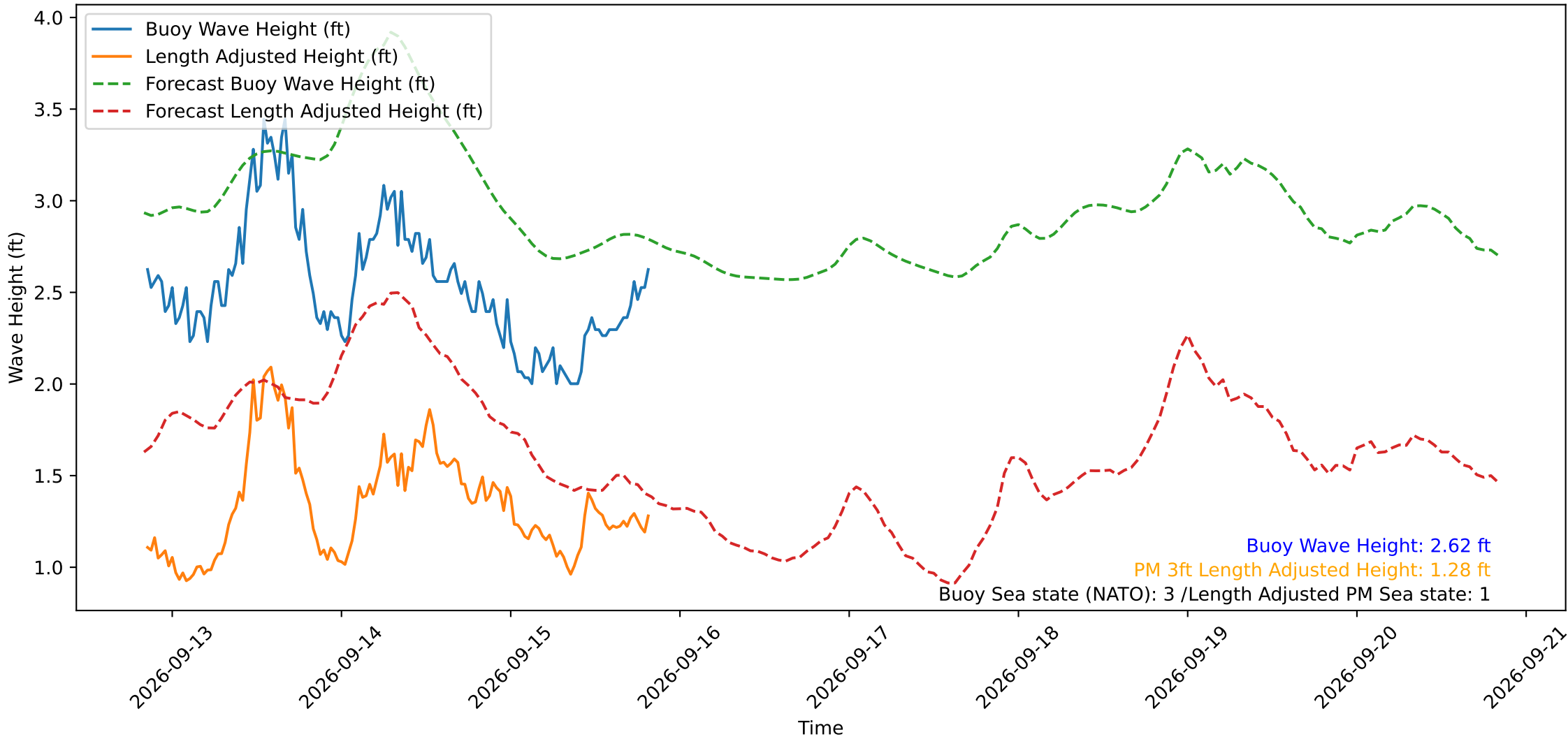
Wave Heights over Time for Red Beach at 2026-09-15 20:10:49
