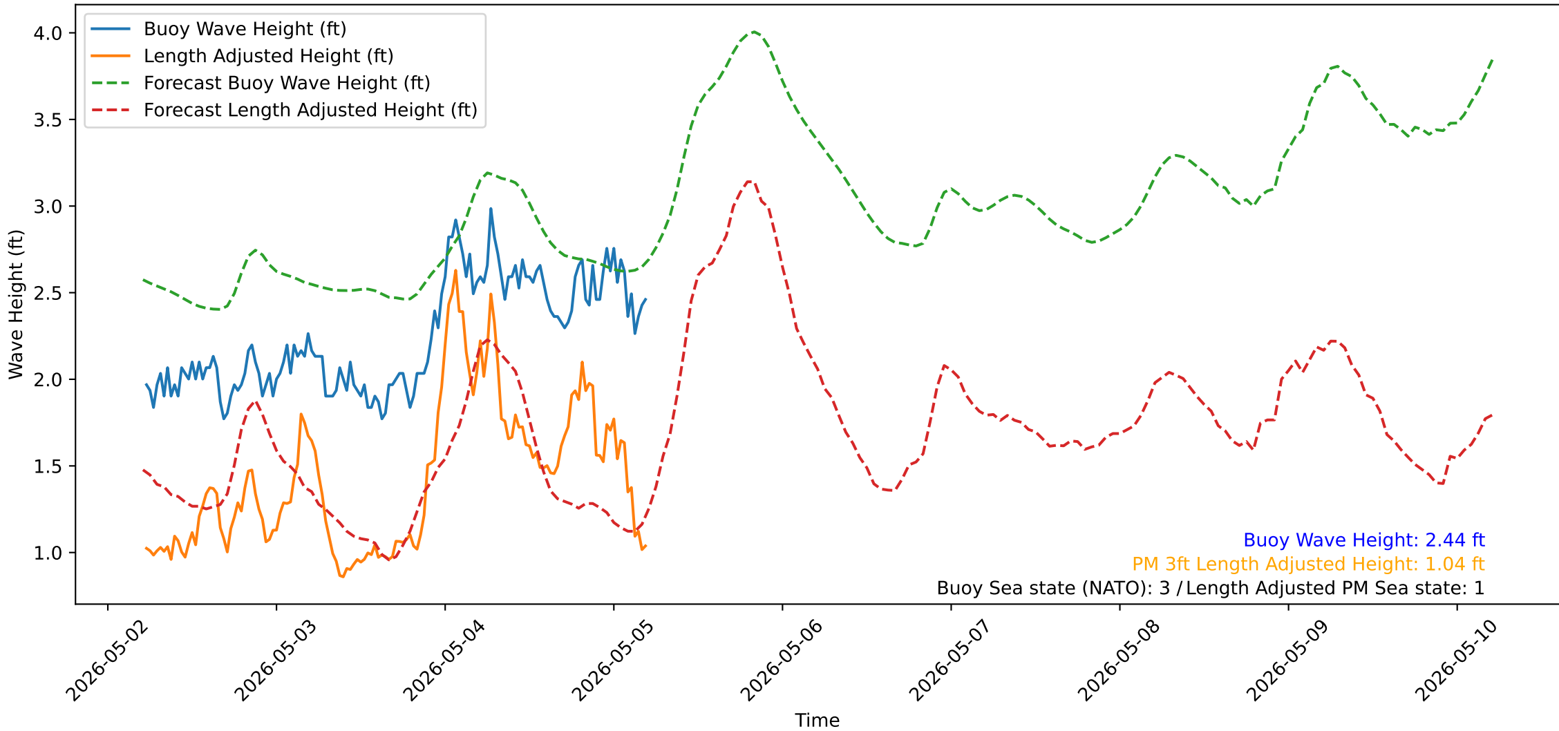
Wave Heights over Time for Green Beach at 2026-05-05 05:21:13
