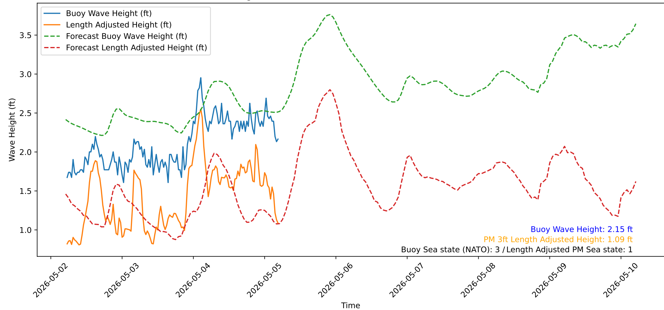
Wave Heights over Time for Red Beach at 2026-05-05 05:20:51
