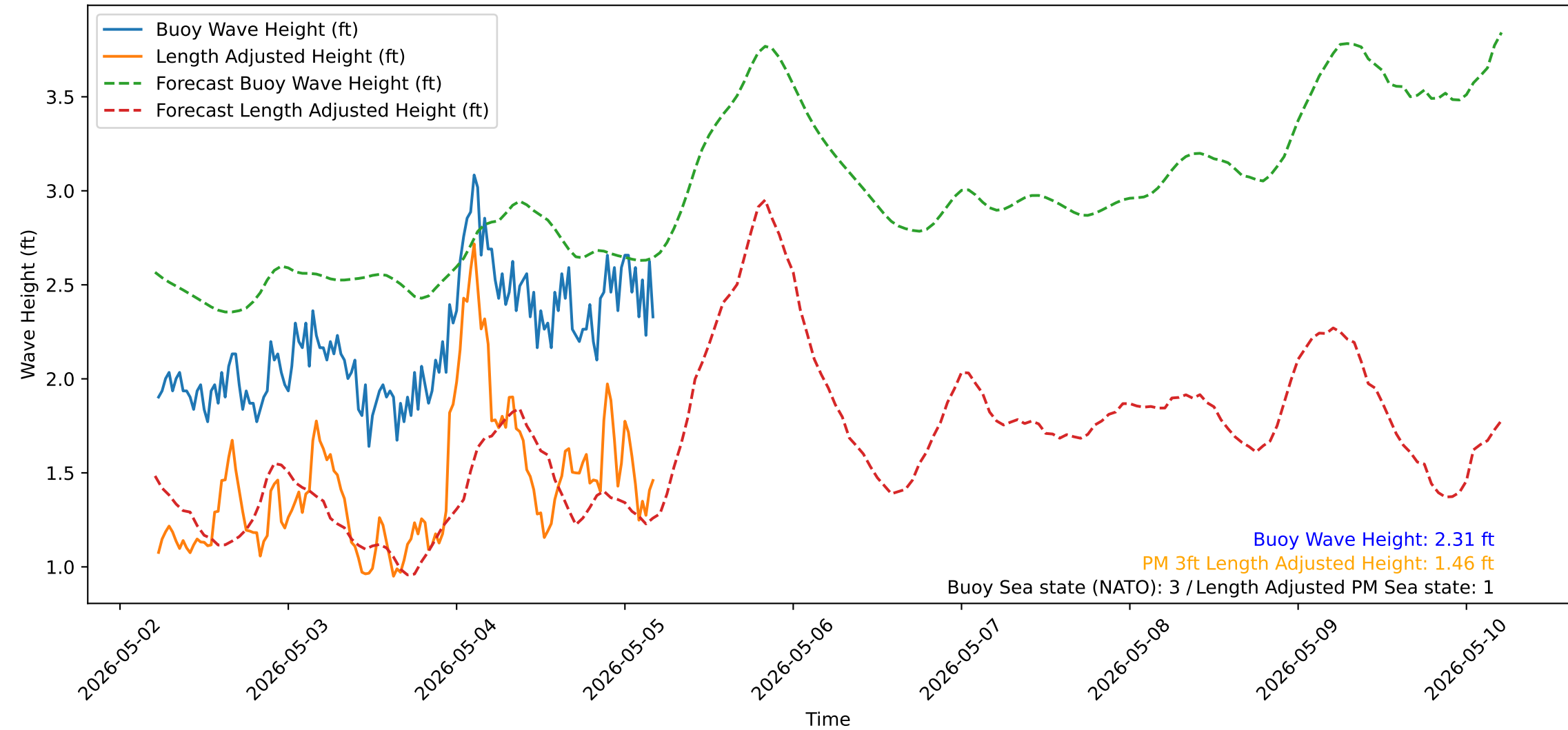
Wave Heights over Time for Oceanside Harbor at 2026-05-05 05:20:31
