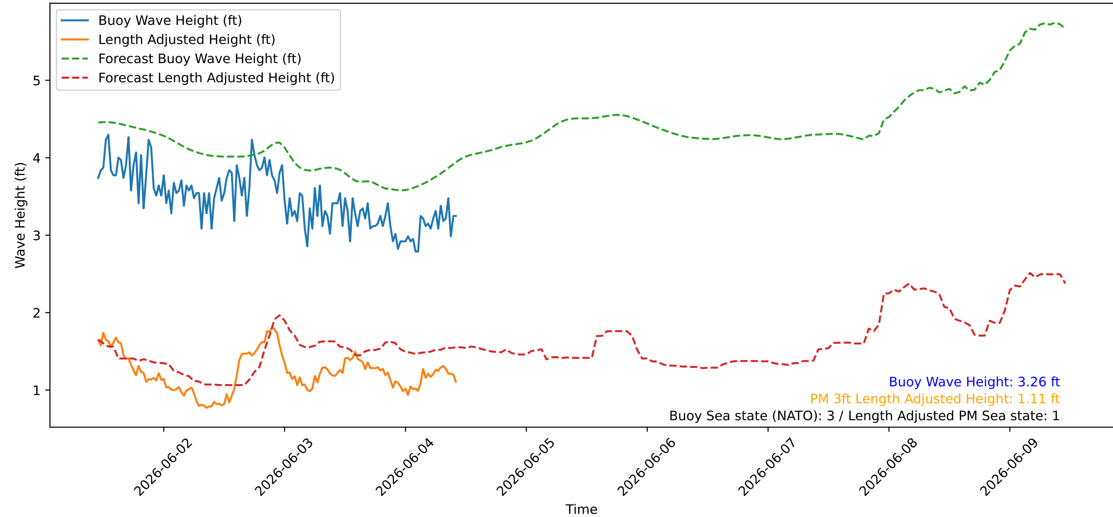
Wave Heights over Time for Green Beach at 2026-06-04 11:01:07
