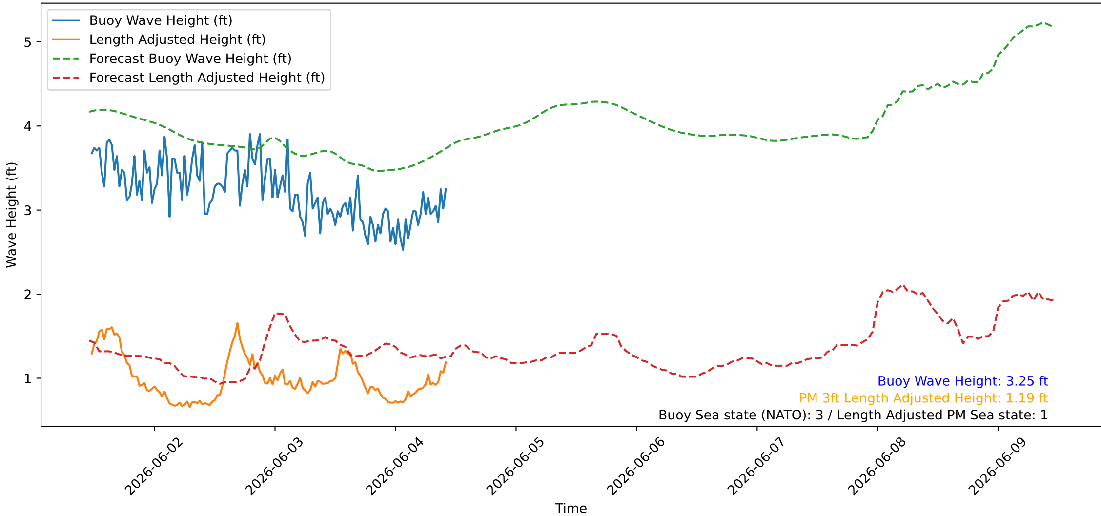
Wave Heights over Time for Red Beach at 2026-06-04 11:00:45
