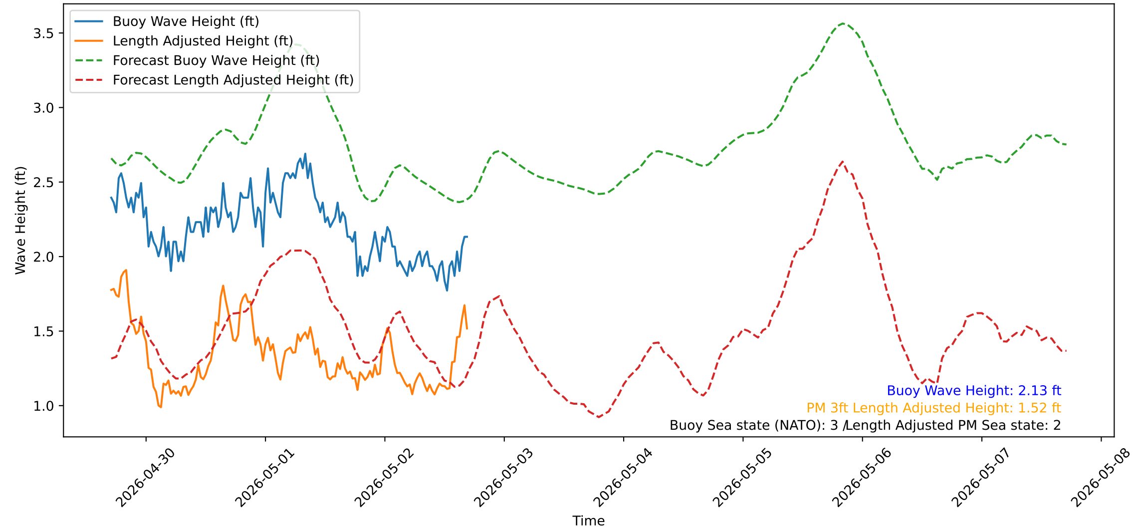
Wave Heights over Time for Oceanside Harbor at 2026-05-02 17:10:31
