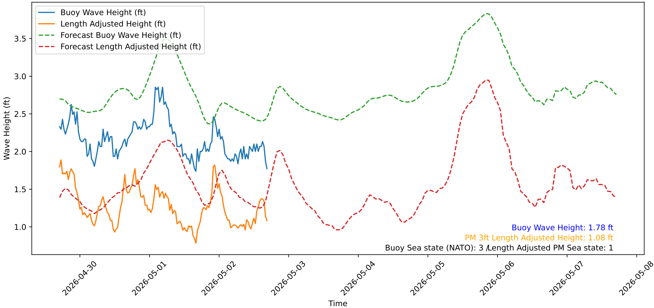
Wave Heights over Time for Green Beach at 2026-05-02 17:11:12
