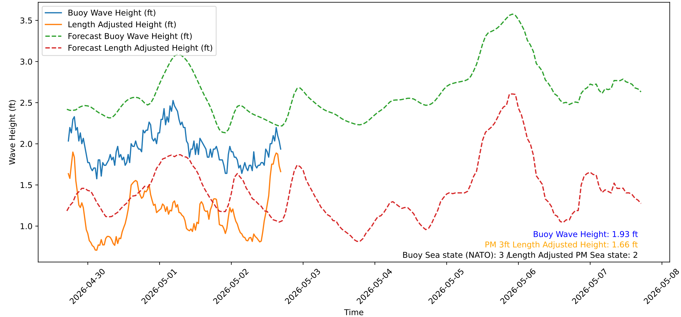
Wave Heights over Time for Red Beach at 2026-05-02 17:10:50
