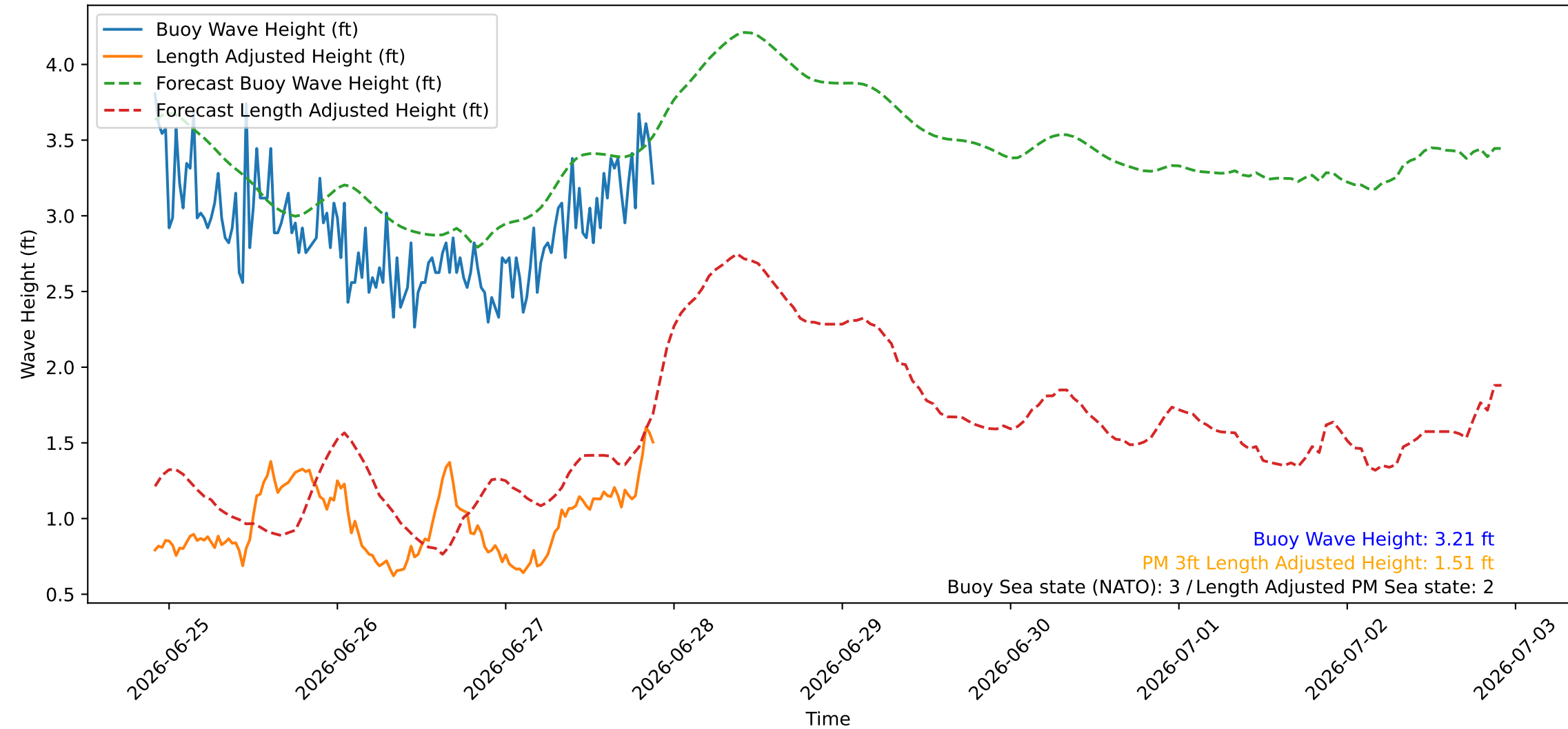
Wave Heights over Time for Red Beach at 2026-06-27 21:50:47
