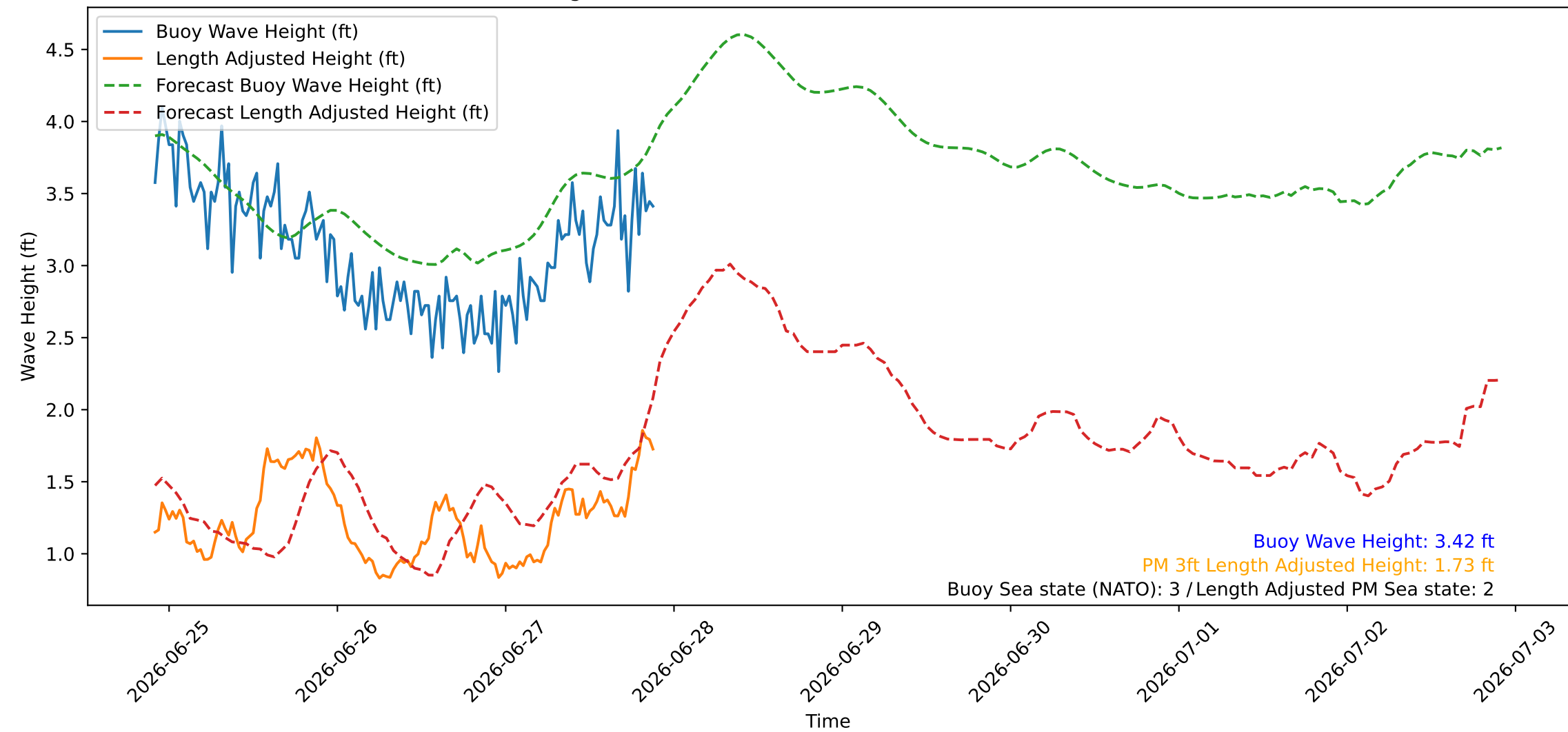
Wave Heights over Time for Green Beach at 2026-06-27 21:51:10
