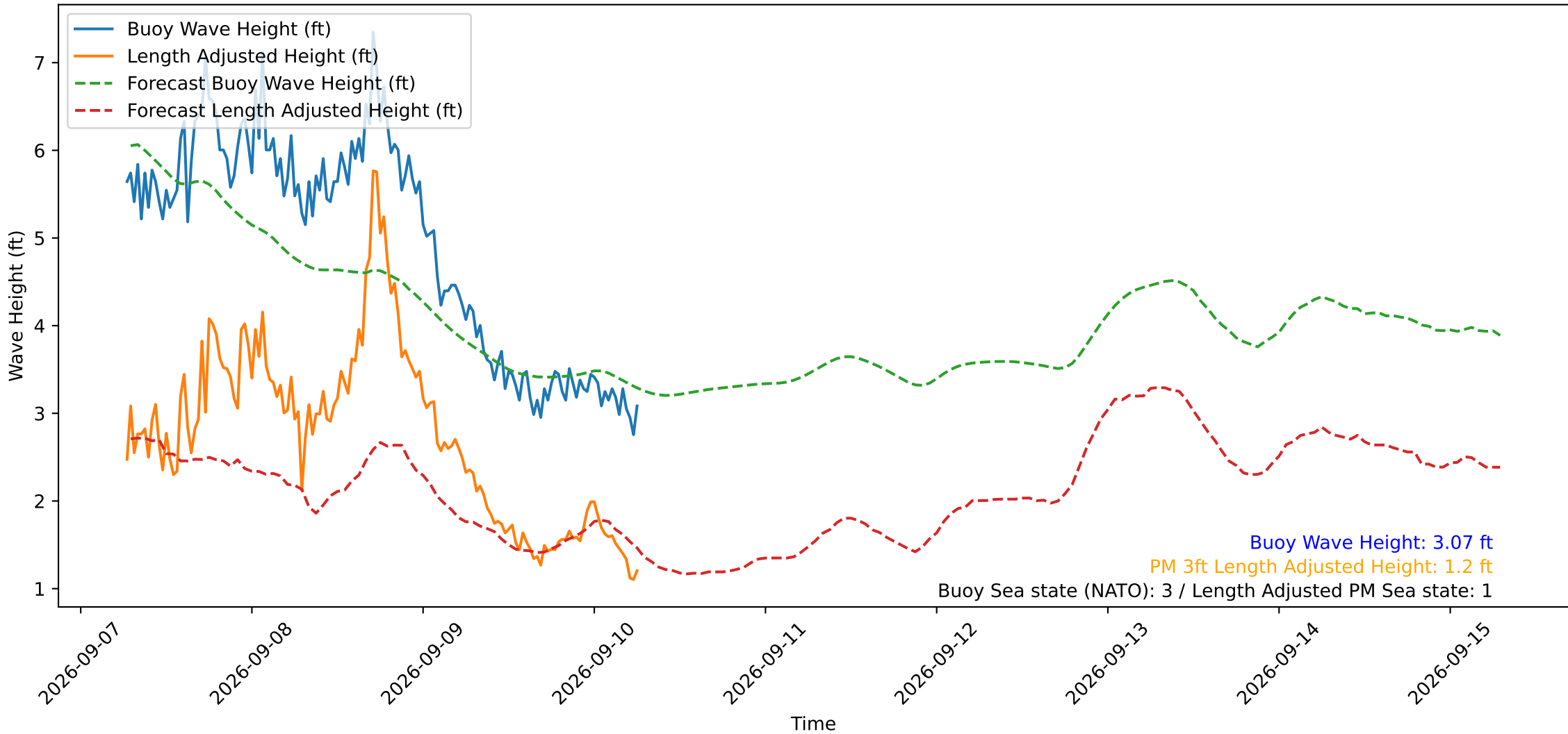
Wave Heights over Time for Oceanside Harbor at 2026-09-10 06:40:30
