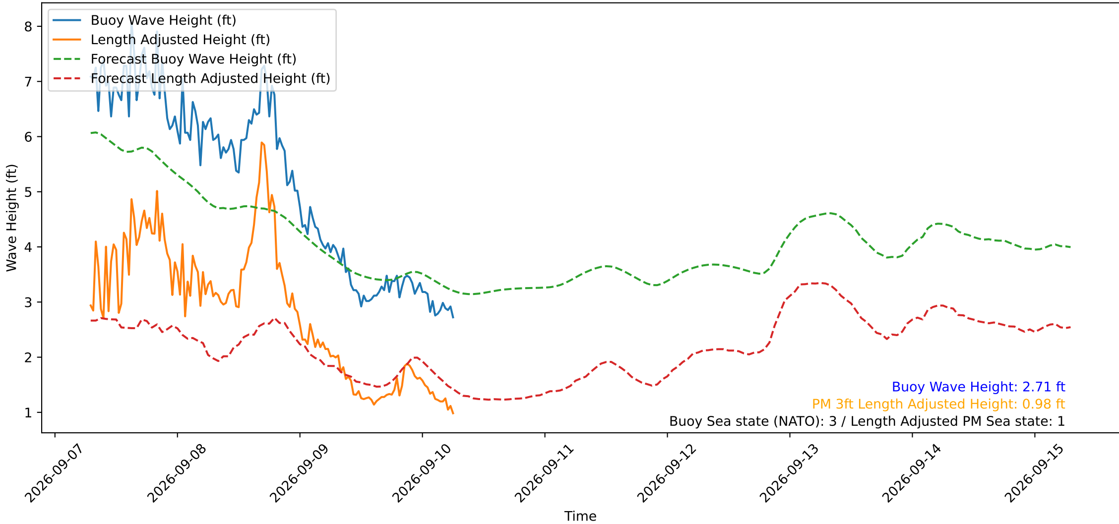
Wave Heights over Time for Green Beach at 2026-09-10 06:41:12
