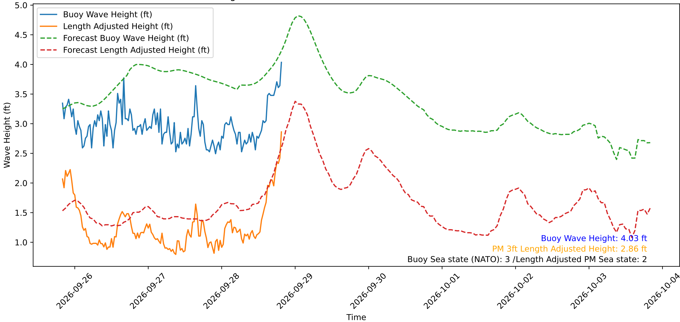
Wave Heights over Time for Oceanside Harbor at 2026-09-28 20:10:29
