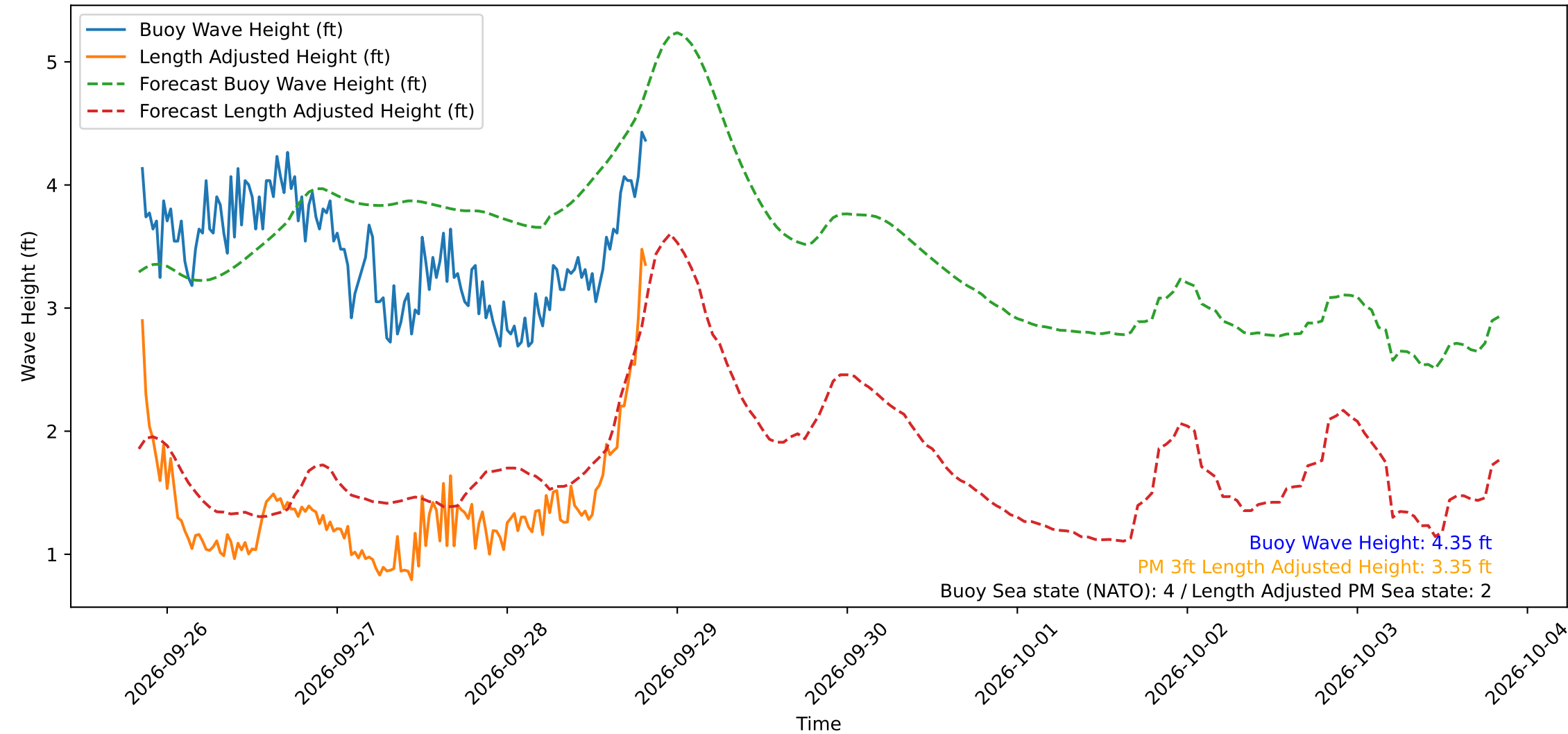
Wave Heights over Time for Green Beach at 2026-09-28 20:11:11
