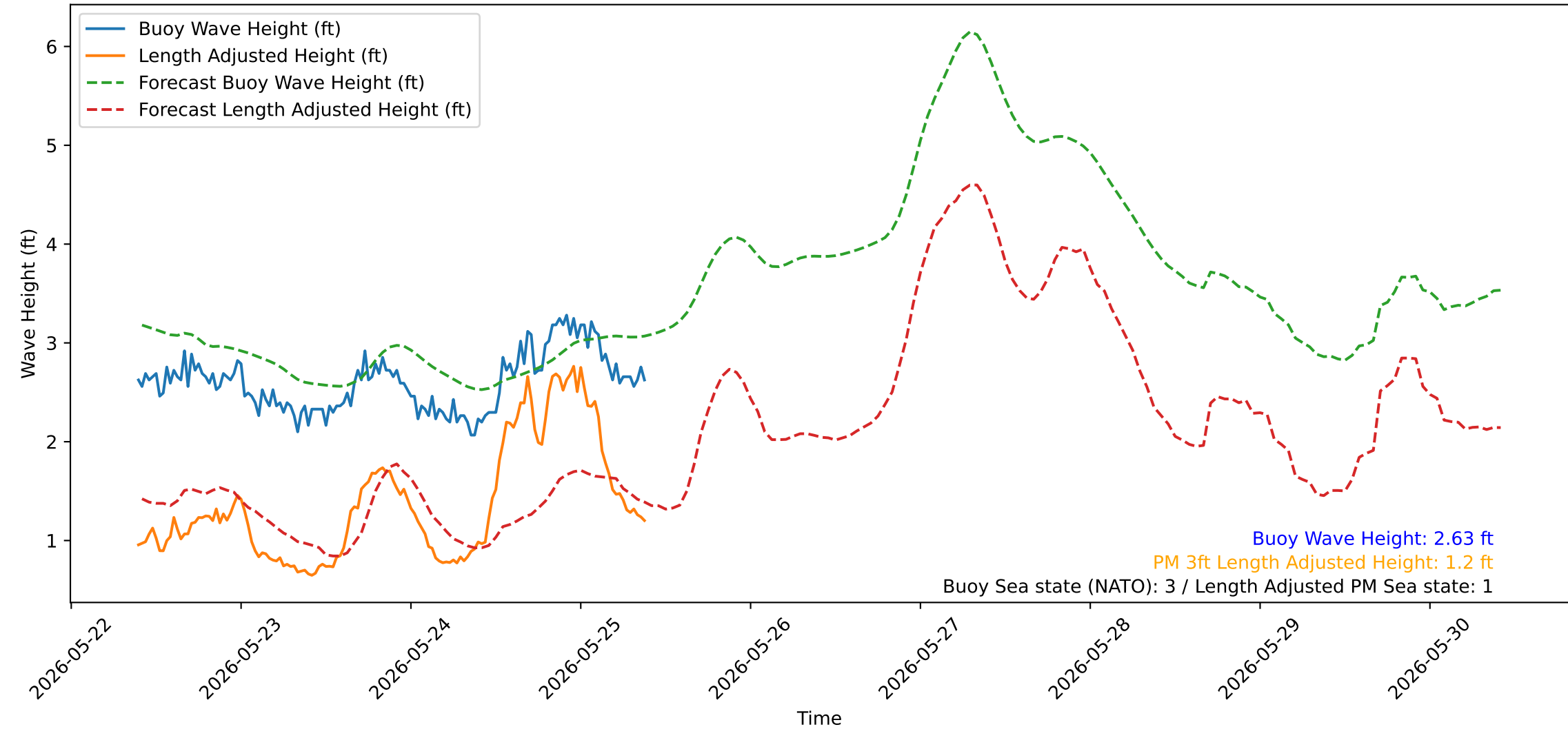
Wave Heights over Time for Green Beach at 2026-05-25 09:41:11
