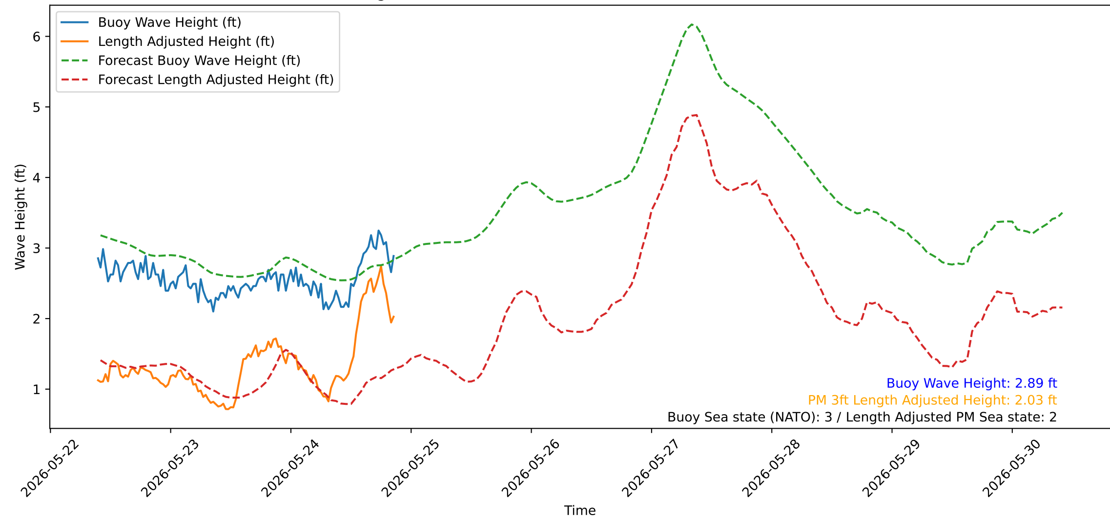
Wave Heights over Time for Oceanside Harbor at 2026-05-25 09:40:29
