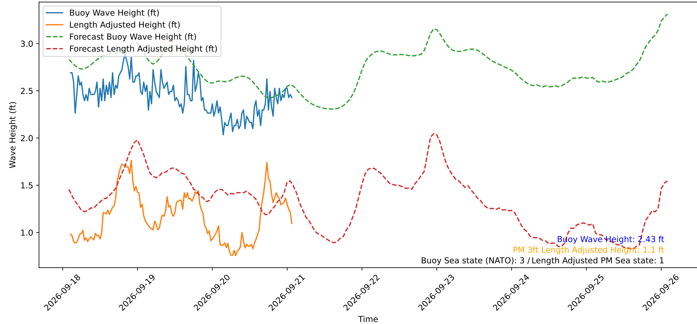
Wave Heights over Time for Red Beach at 2026-09-21 02:10:49
