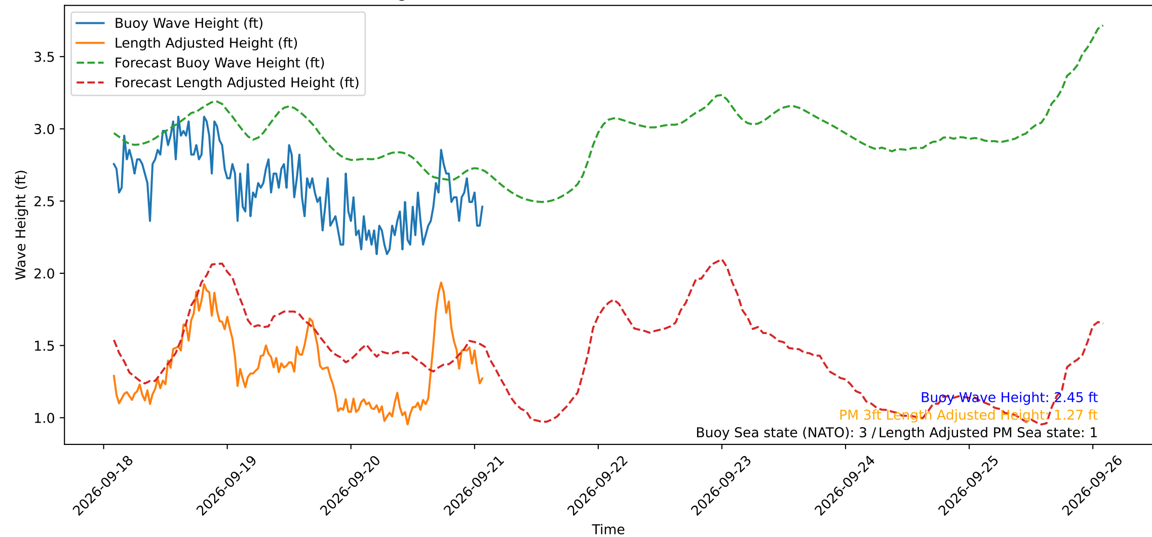
Wave Heights over Time for Oceanside Harbor at 2026-09-21 02:10:29
