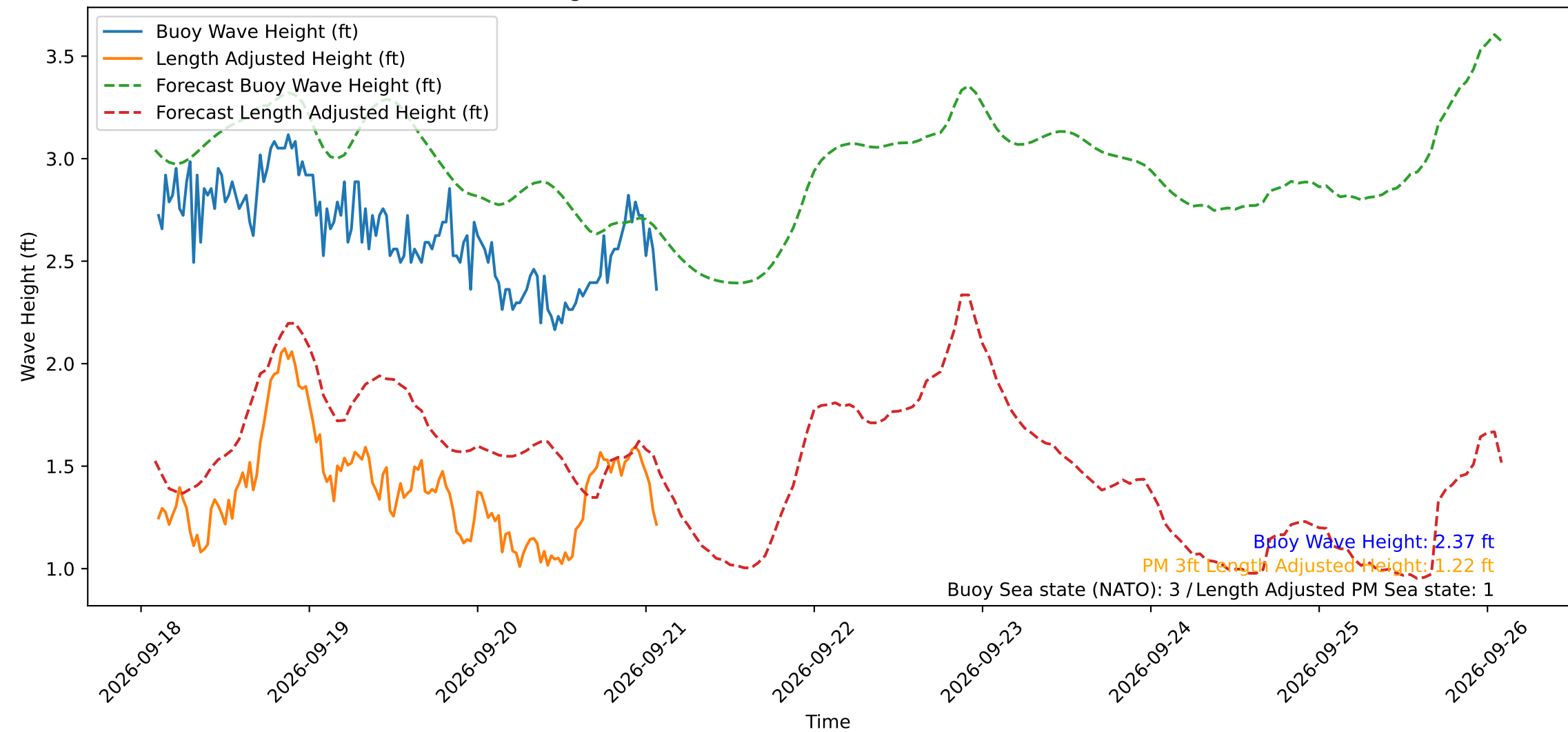
Wave Heights over Time for Green Beach at 2026-09-21 02:11:11
