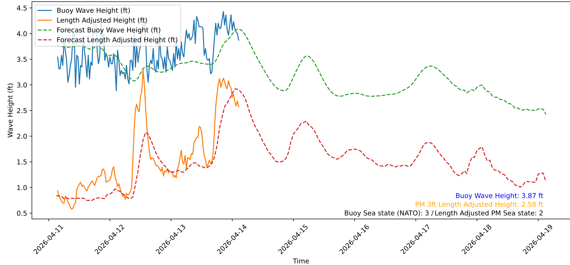
Wave Heights over Time for Red Beach at 2026-04-14 03:20:51
