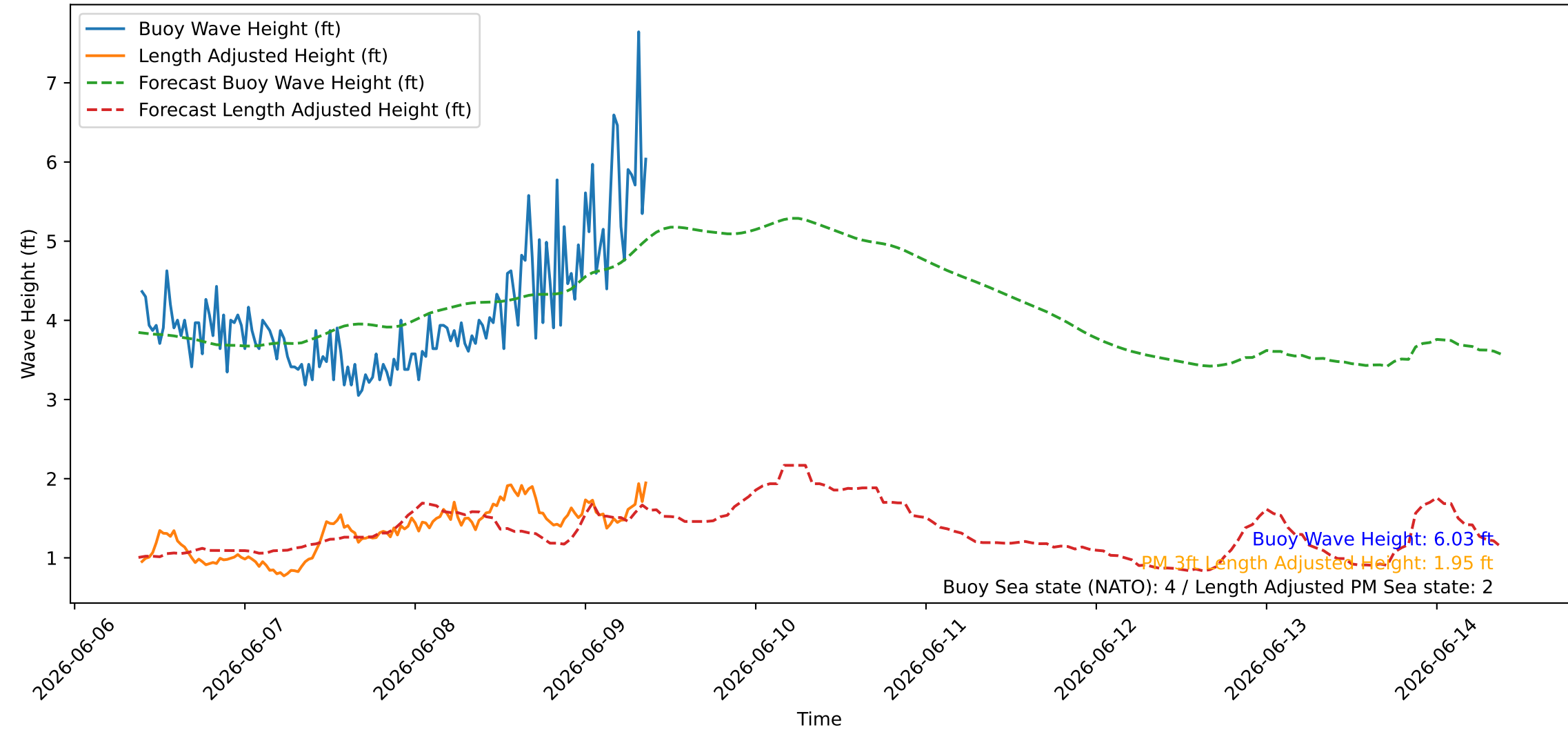
Wave Heights over Time for Red Beach at 2026-06-09 09:10:45
