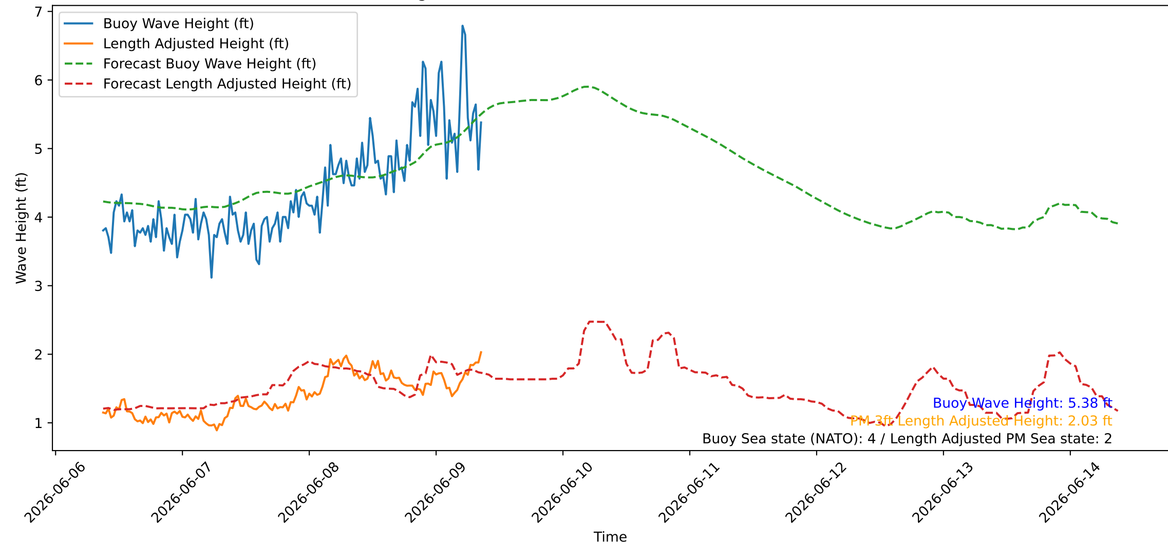
Wave Heights over Time for Green Beach at 2026-06-09 09:11:08
