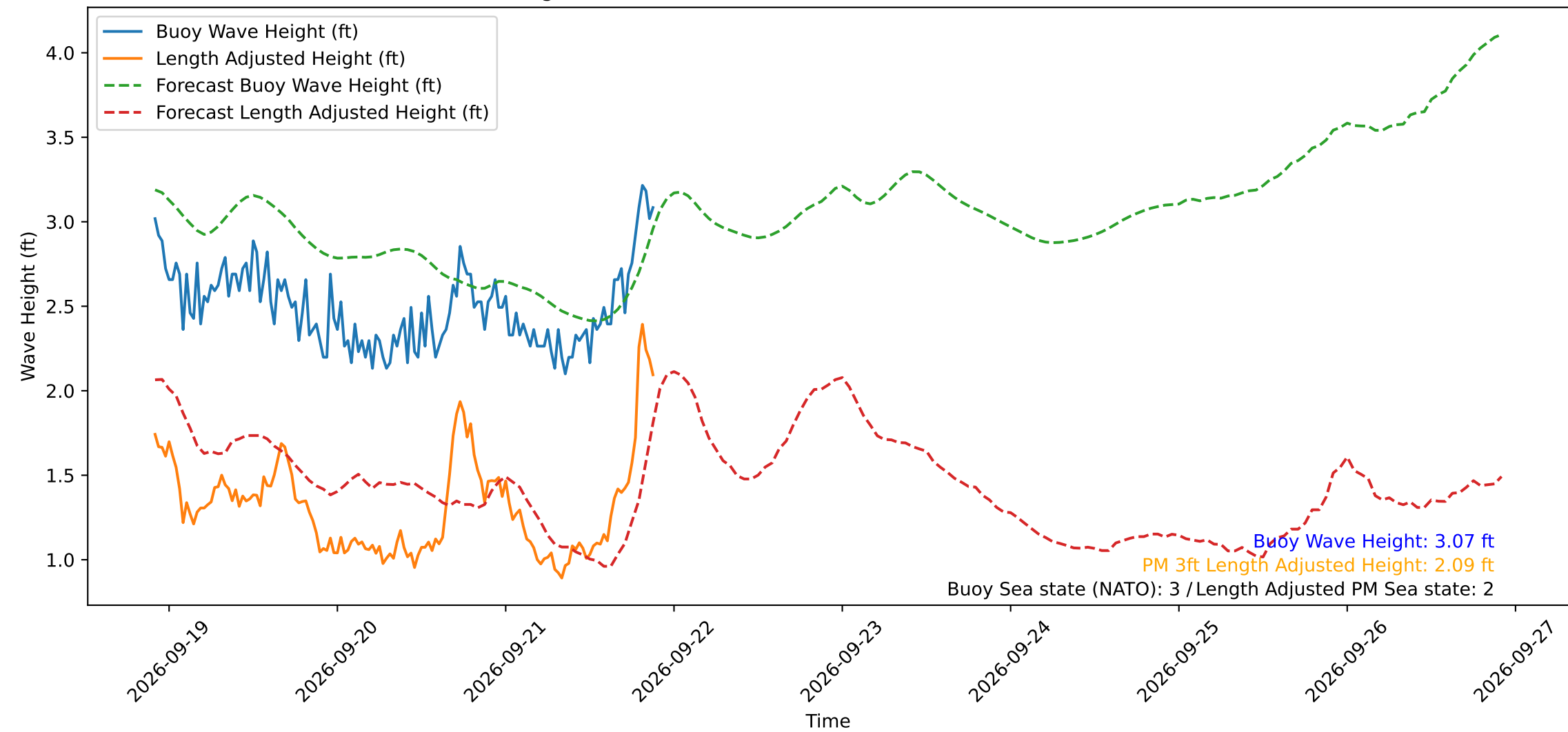
Wave Heights over Time for Oceanside Harbor at 2026-09-21 21:50:30
