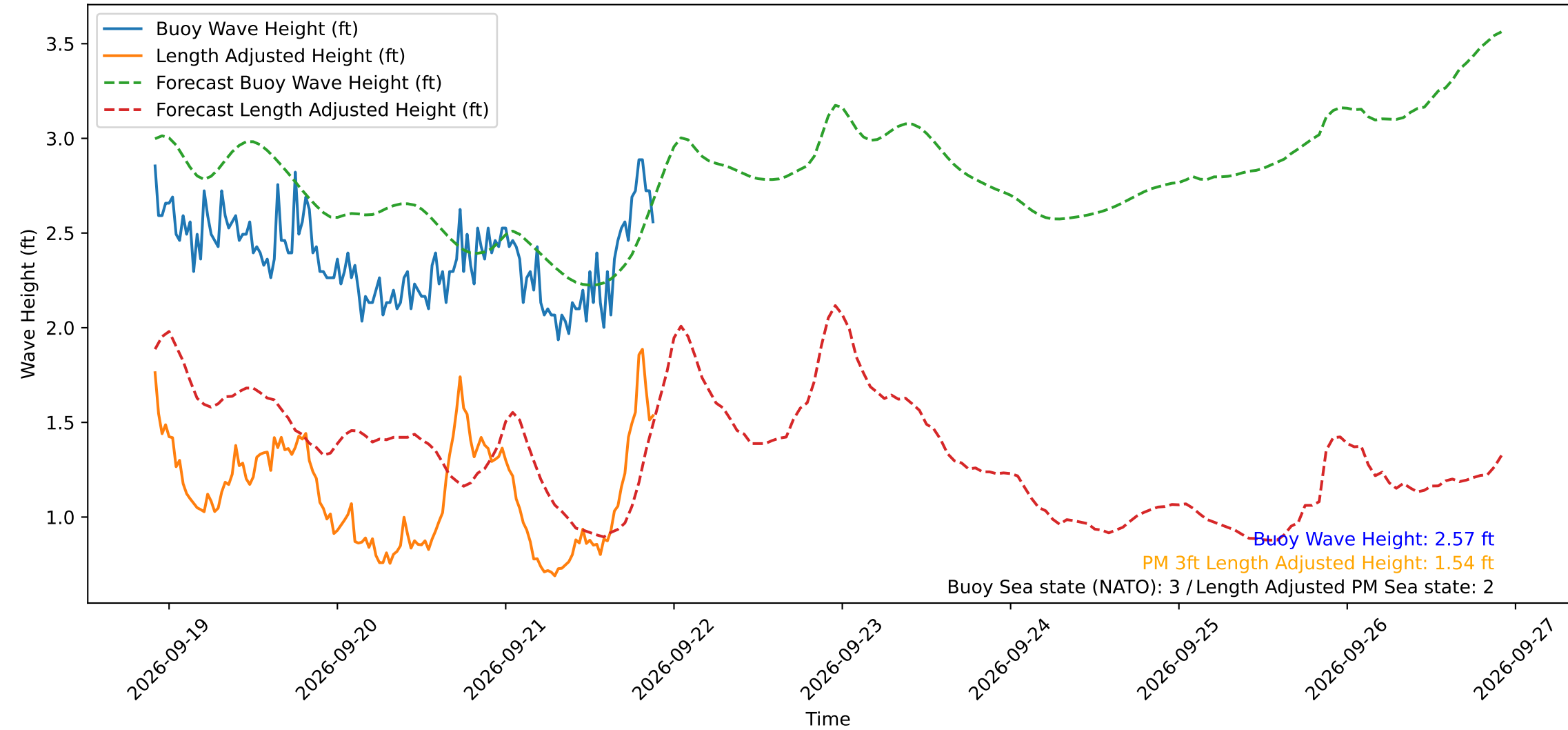
Wave Heights over Time for Red Beach at 2026-09-21 21:50:51
