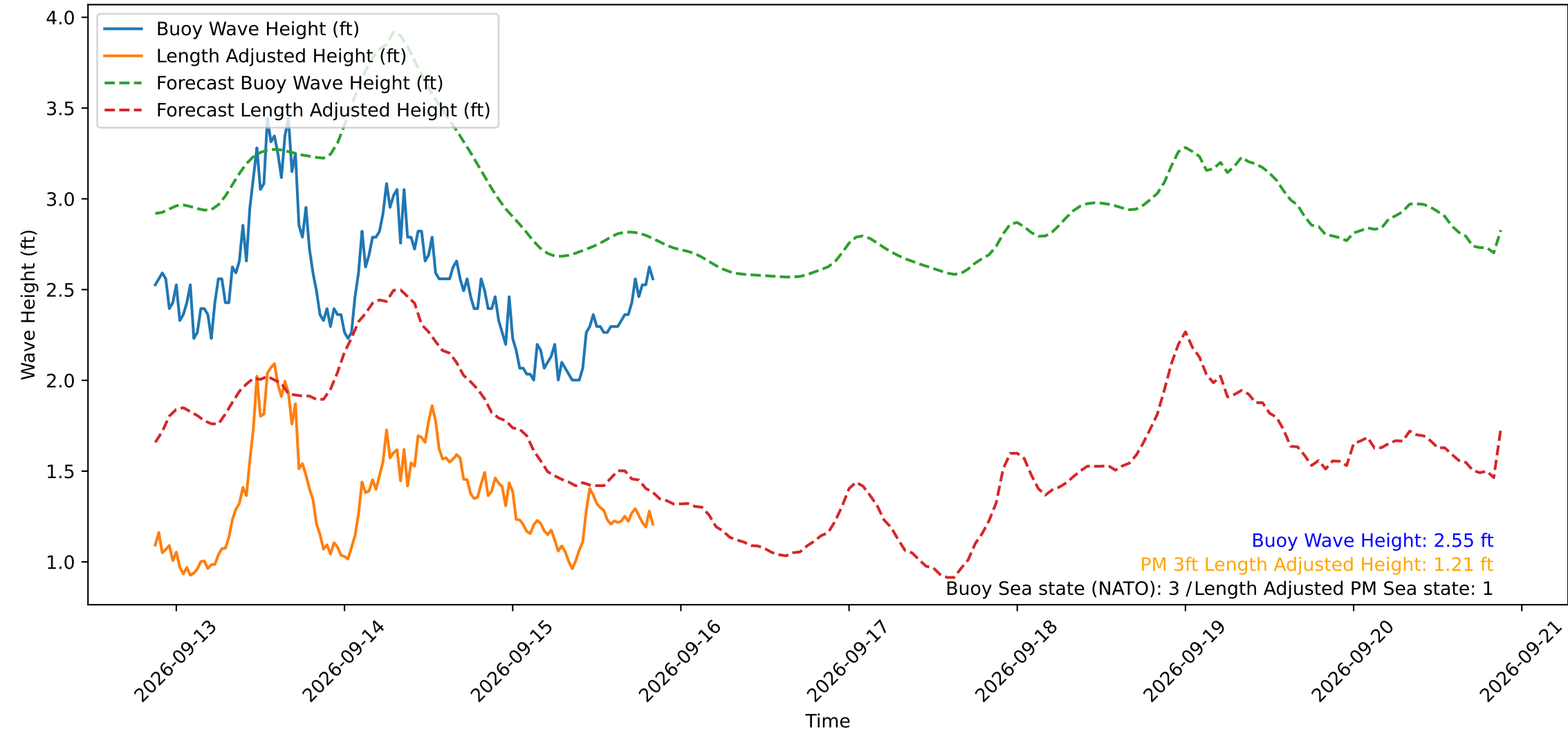
Wave Heights over Time for Red Beach at 2026-09-15 20:40:50
