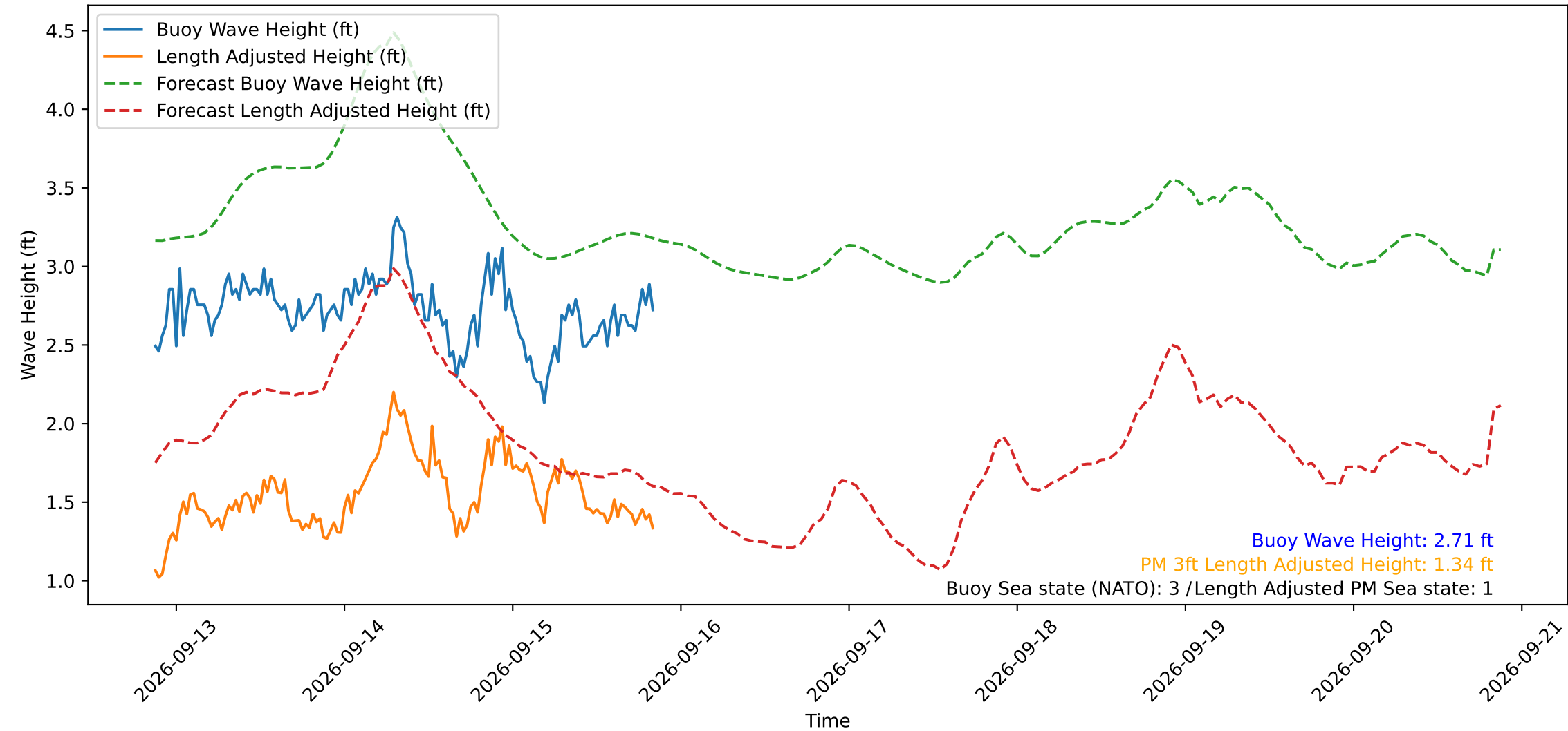
Wave Heights over Time for Green Beach at 2026-09-15 20:41:13
