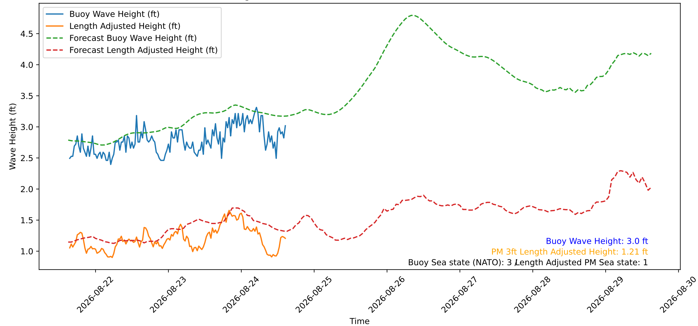
Wave Heights over Time for Green Beach at 2026-08-24 15:11:11
