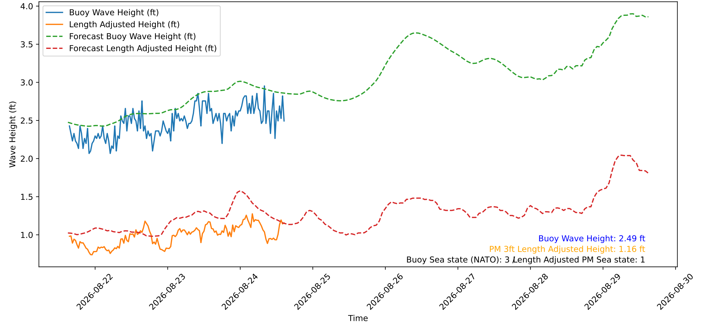
Wave Heights over Time for Red Beach at 2026-08-24 15:10:48
