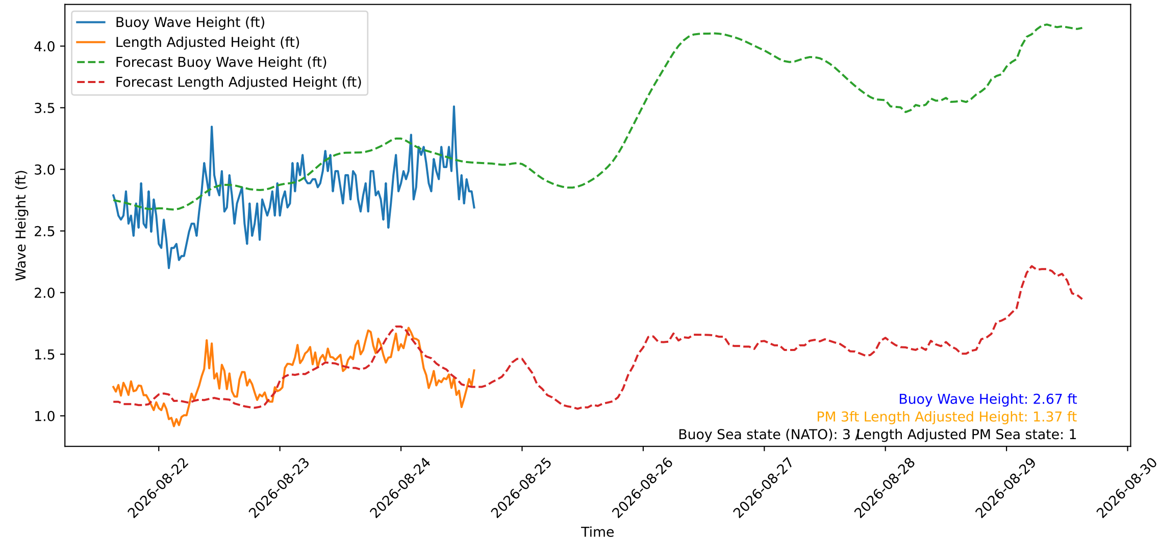
Wave Heights over Time for Oceanside Harbor at 2026-08-24 15:10:29
