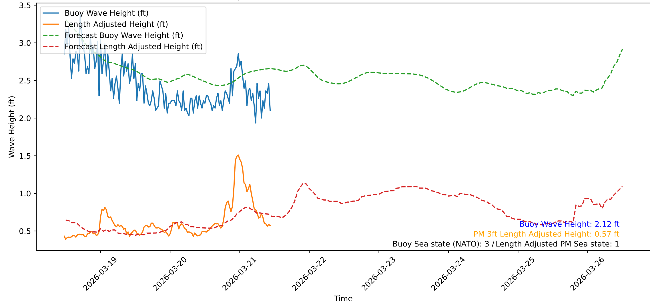
Wave Heights over Time for Green Beach at 2026-03-21 11:31:10
