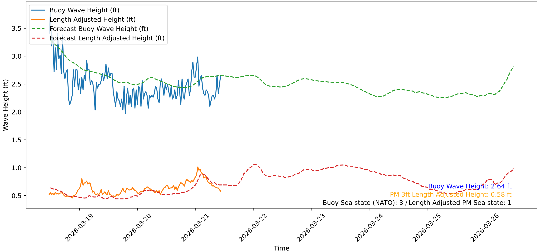
Wave Heights over Time for Oceanside Harbor at 2026-03-21 11:30:31
