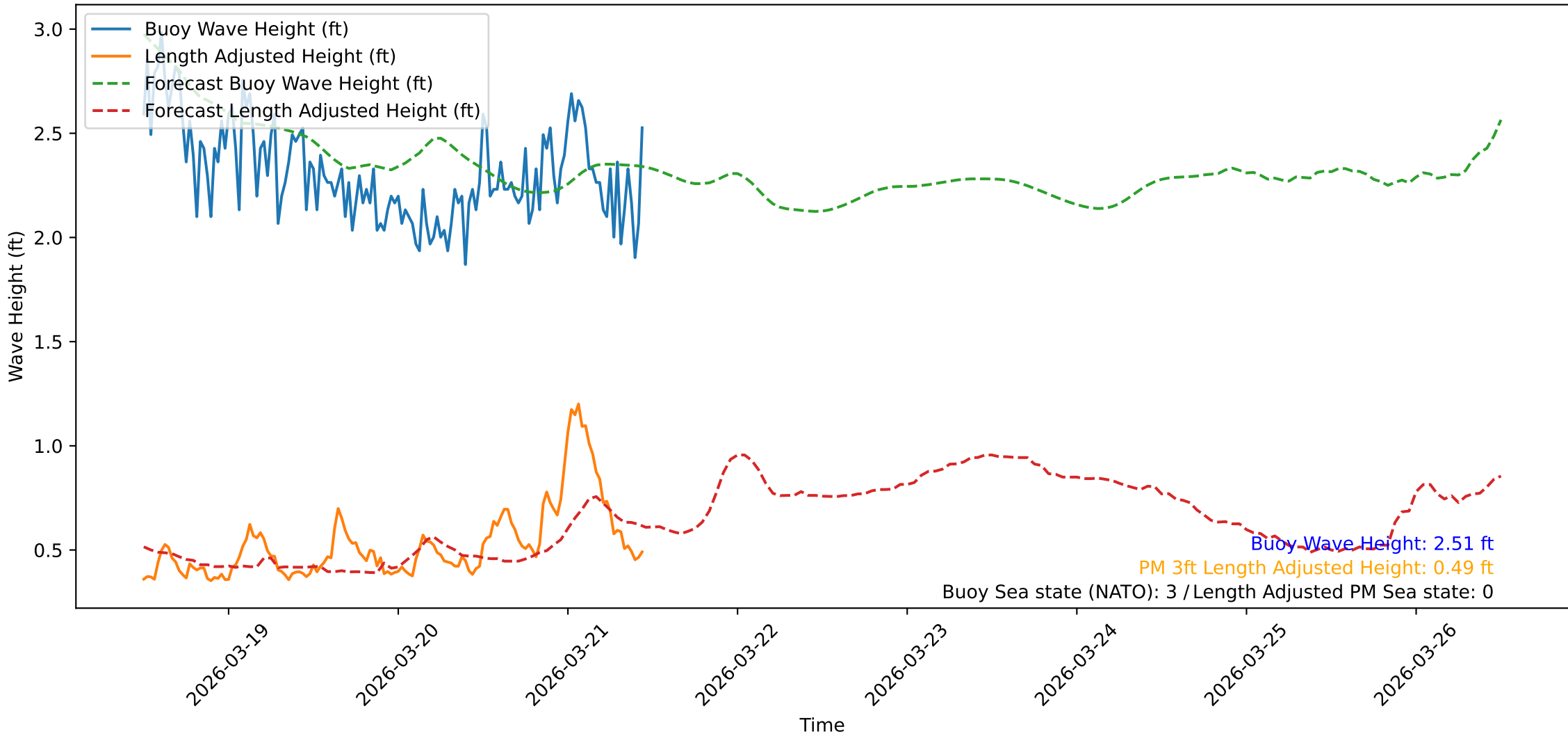
Wave Heights over Time for Red Beach at 2026-03-21 11:30:47
