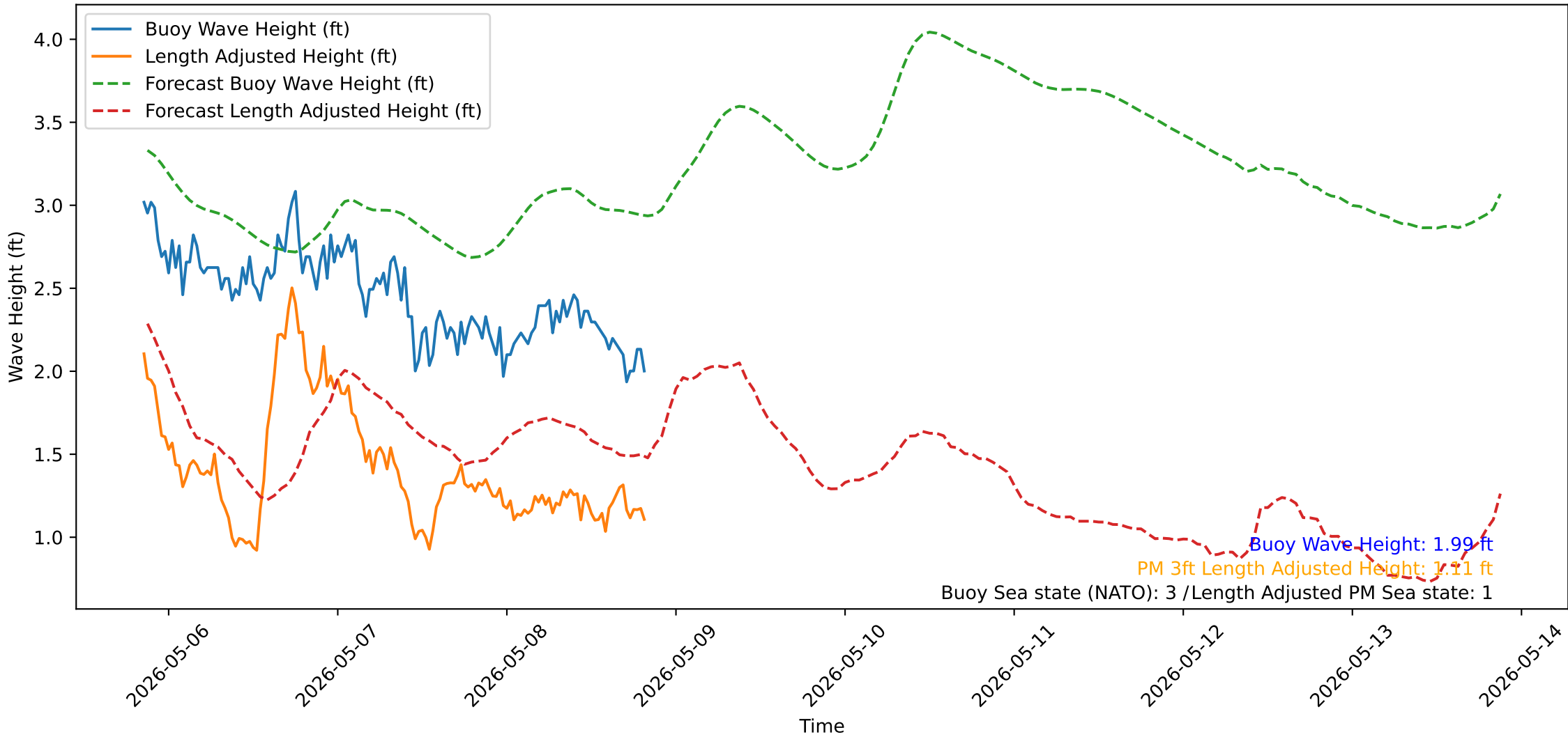
Wave Heights over Time for Oceanside Harbor at 2026-05-08 20:30:32
