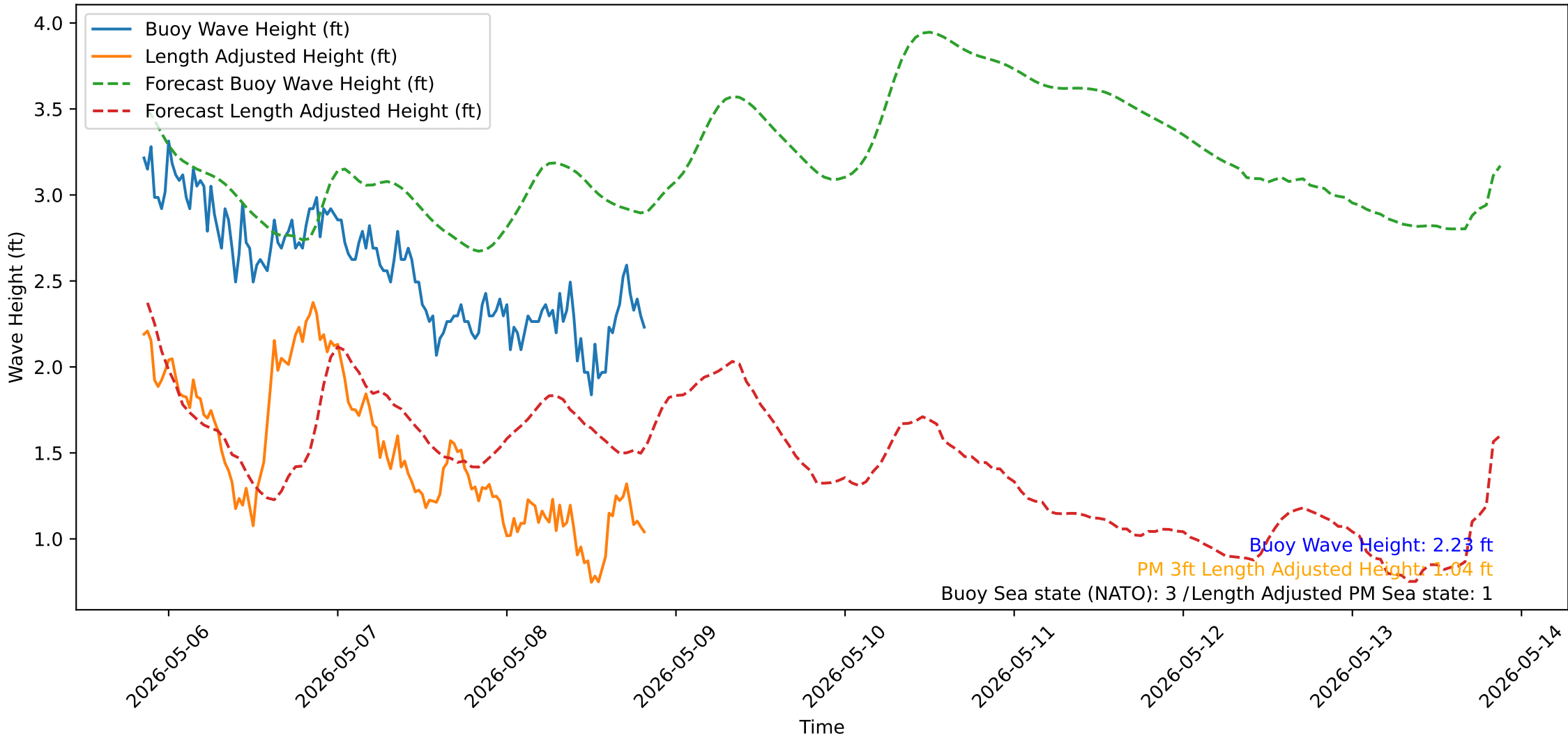
Wave Heights over Time for Green Beach at 2026-05-08 20:31:14
