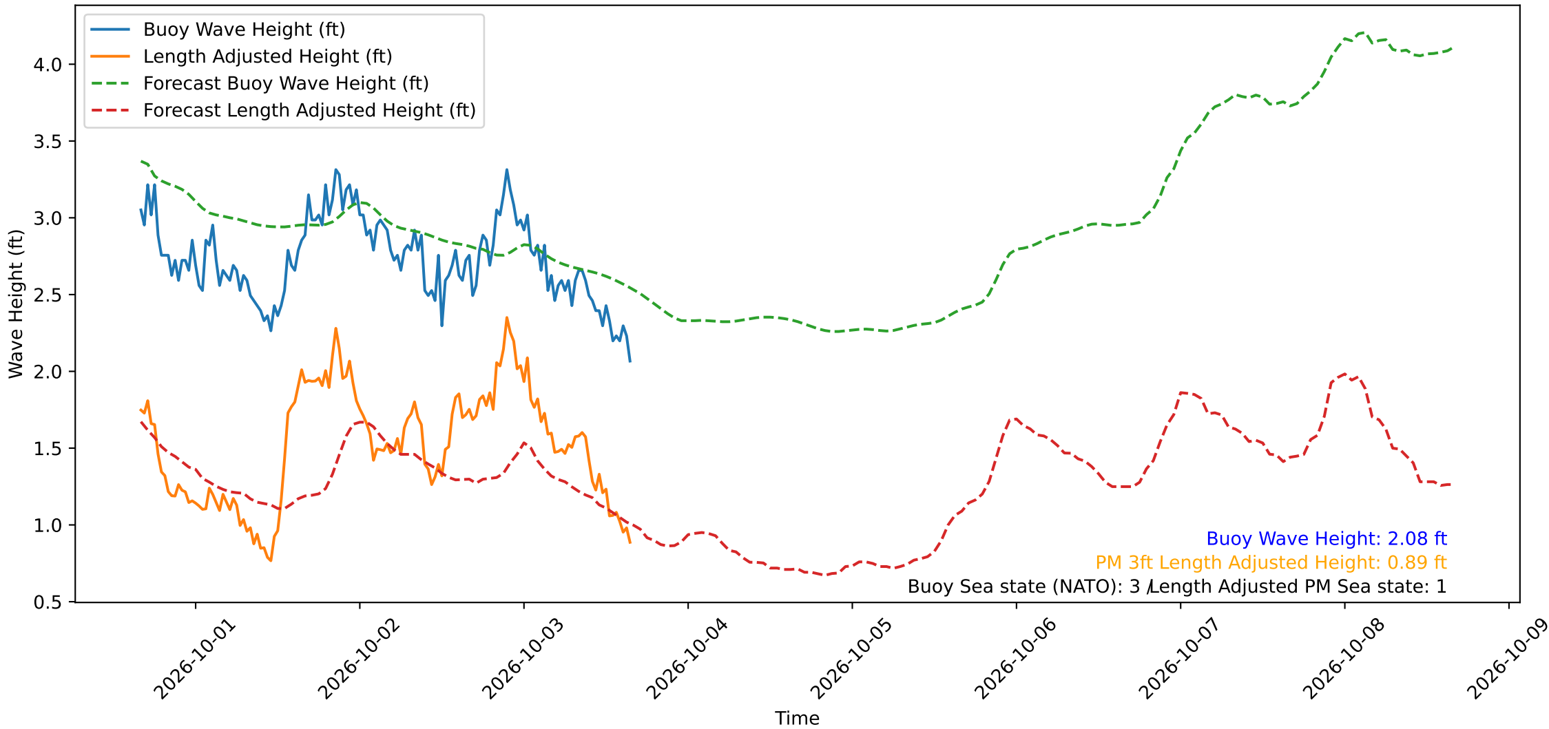
Wave Heights over Time for Oceanside Harbor at 2026-10-03 16:00:29
