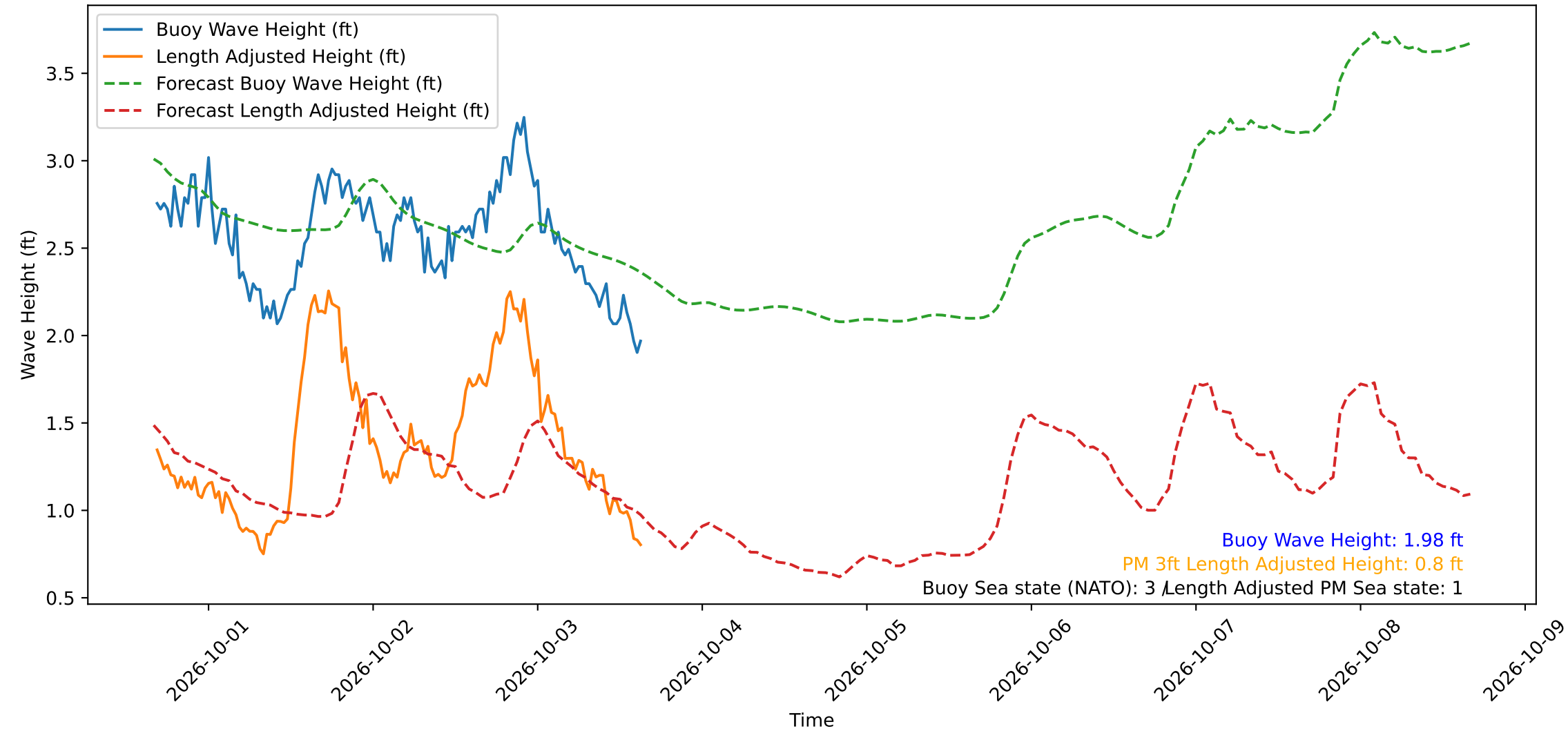
Wave Heights over Time for Red Beach at 2026-10-03 16:00:49
