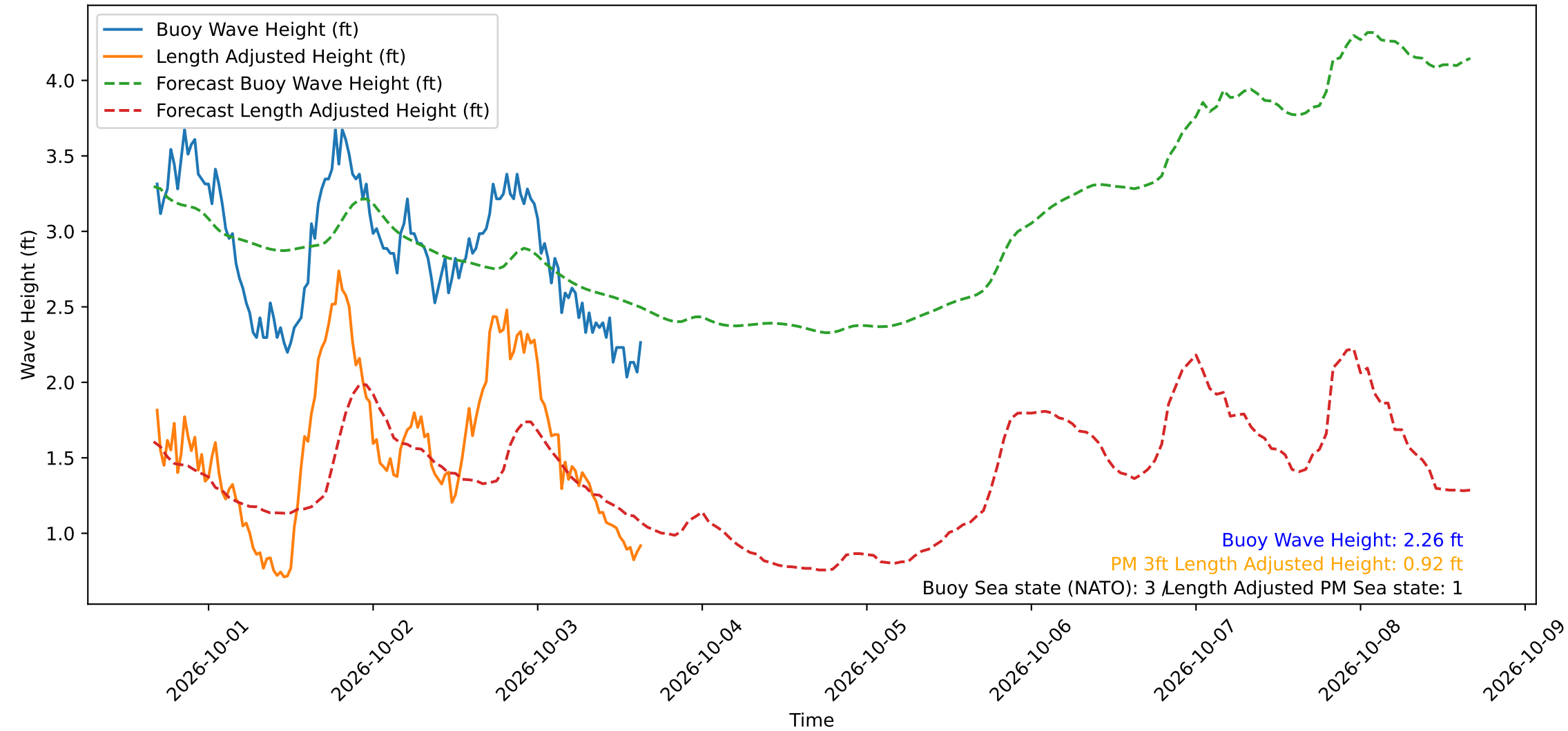
Wave Heights over Time for Green Beach at 2026-10-03 16:01:12
