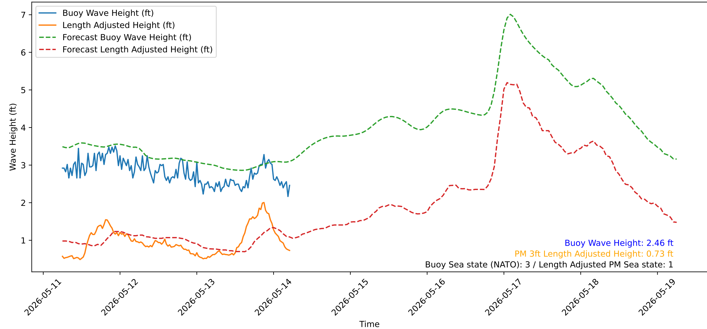
Wave Heights over Time for Green Beach at 2026-05-14 05:51:14
