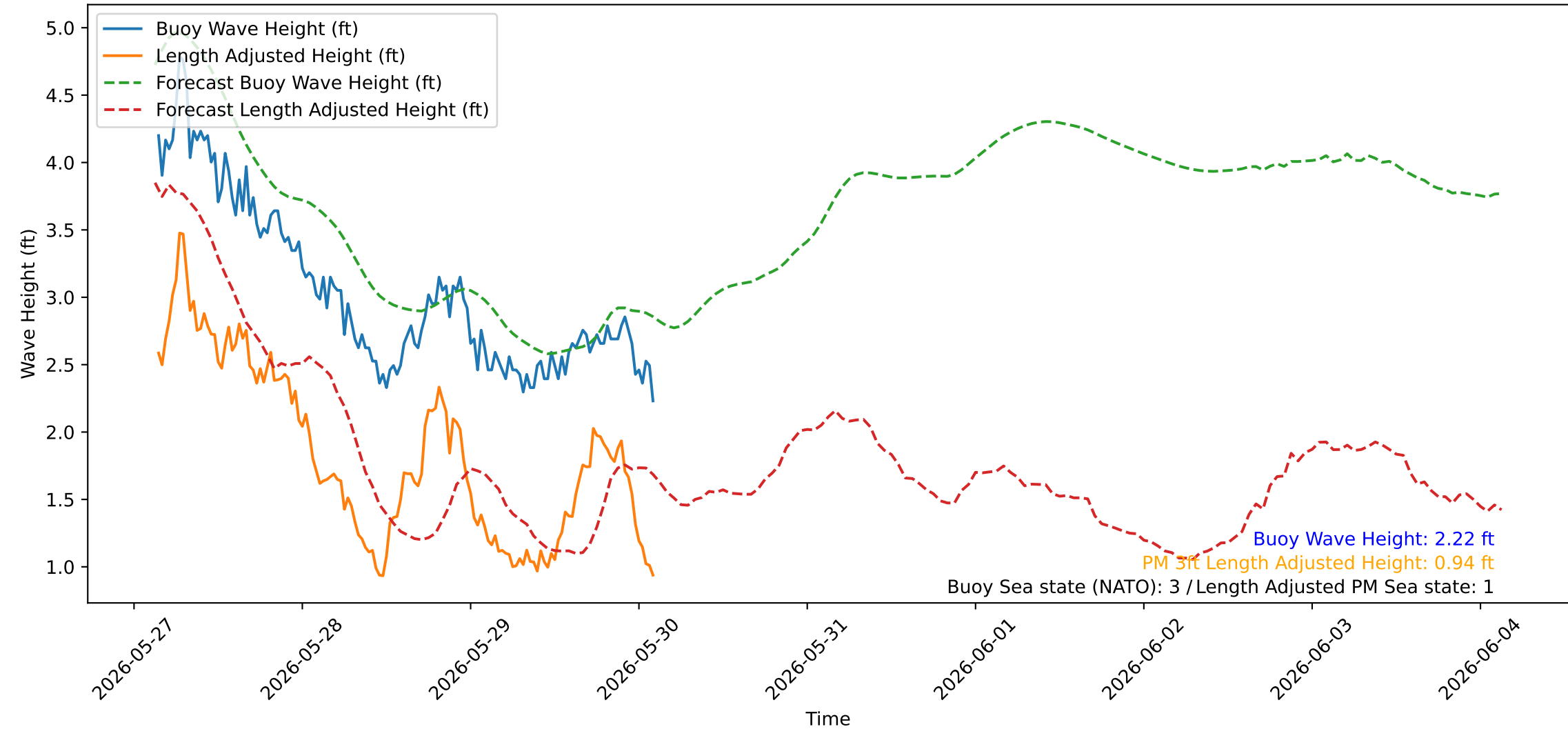
Wave Heights over Time for Red Beach at 2026-05-30 03:00:42
