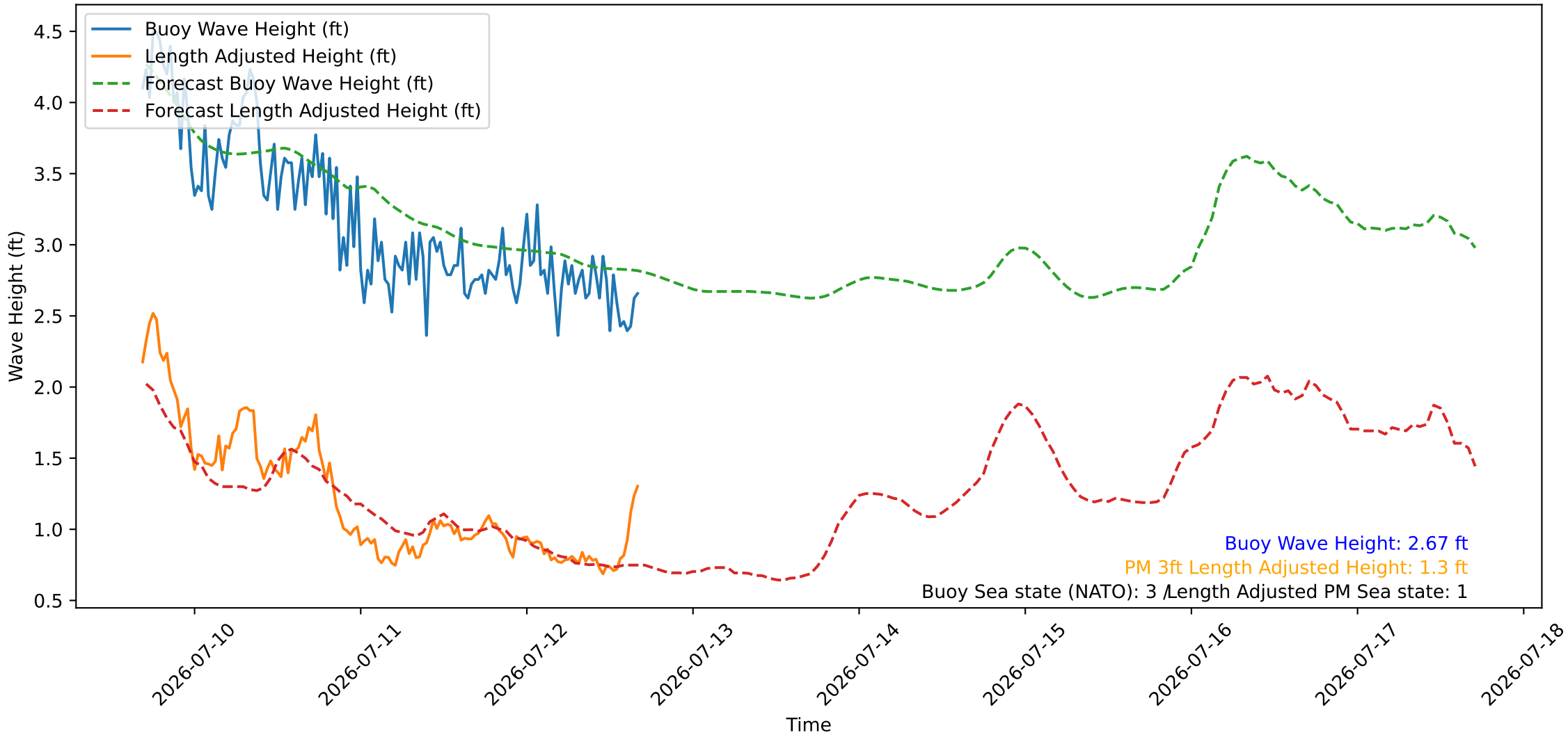
Wave Heights over Time for Oceanside Harbor at 2026-07-12 16:30:26
