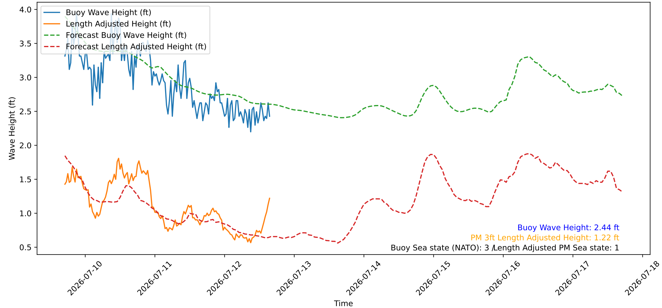
Wave Heights over Time for Red Beach at 2026-07-12 16:30:46
