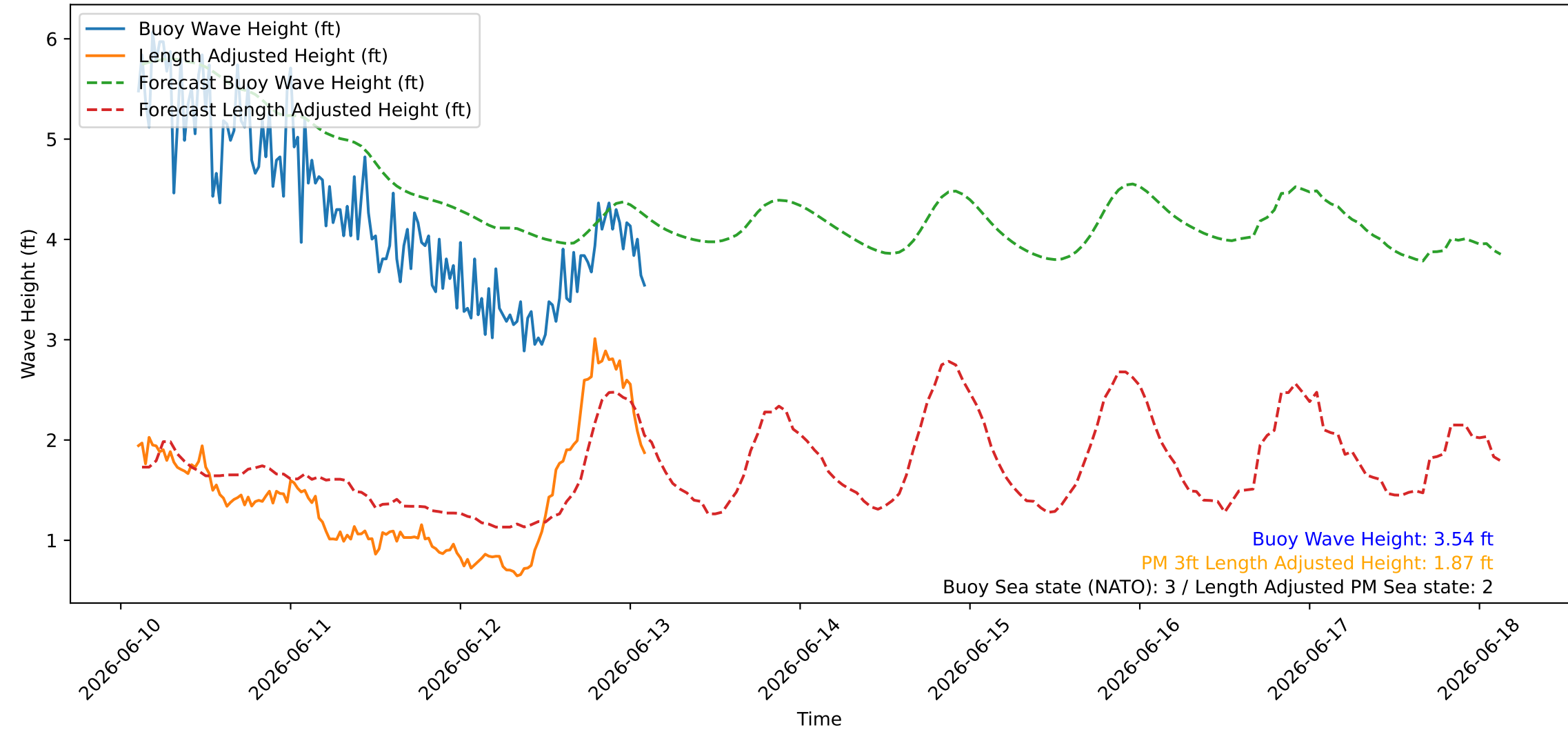
Wave Heights over Time for Green Beach at 2026-06-13 02:41:09
