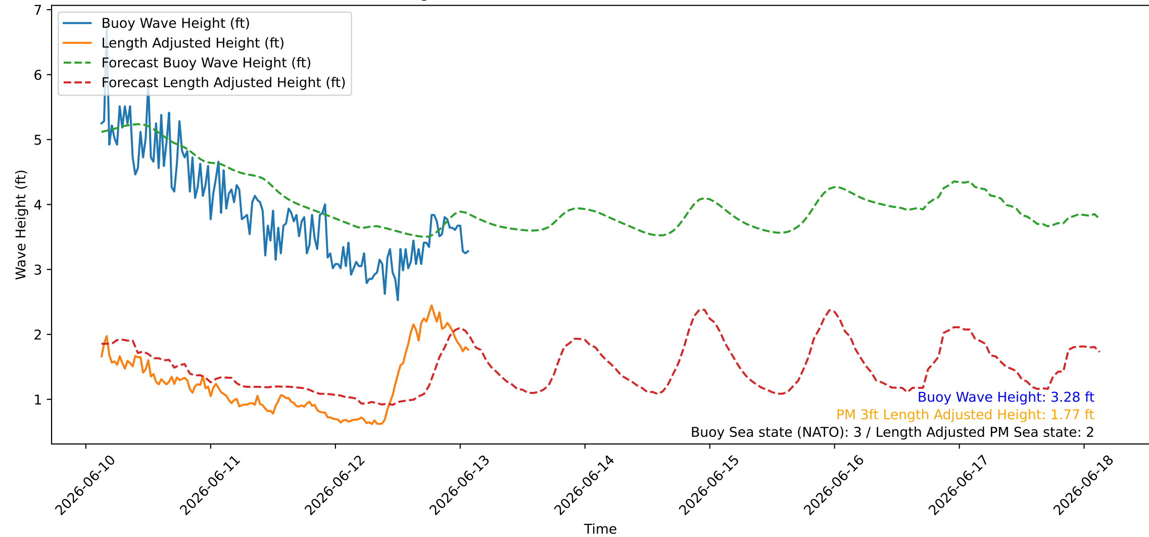
Wave Heights over Time for Red Beach at 2026-06-13 02:40:46
