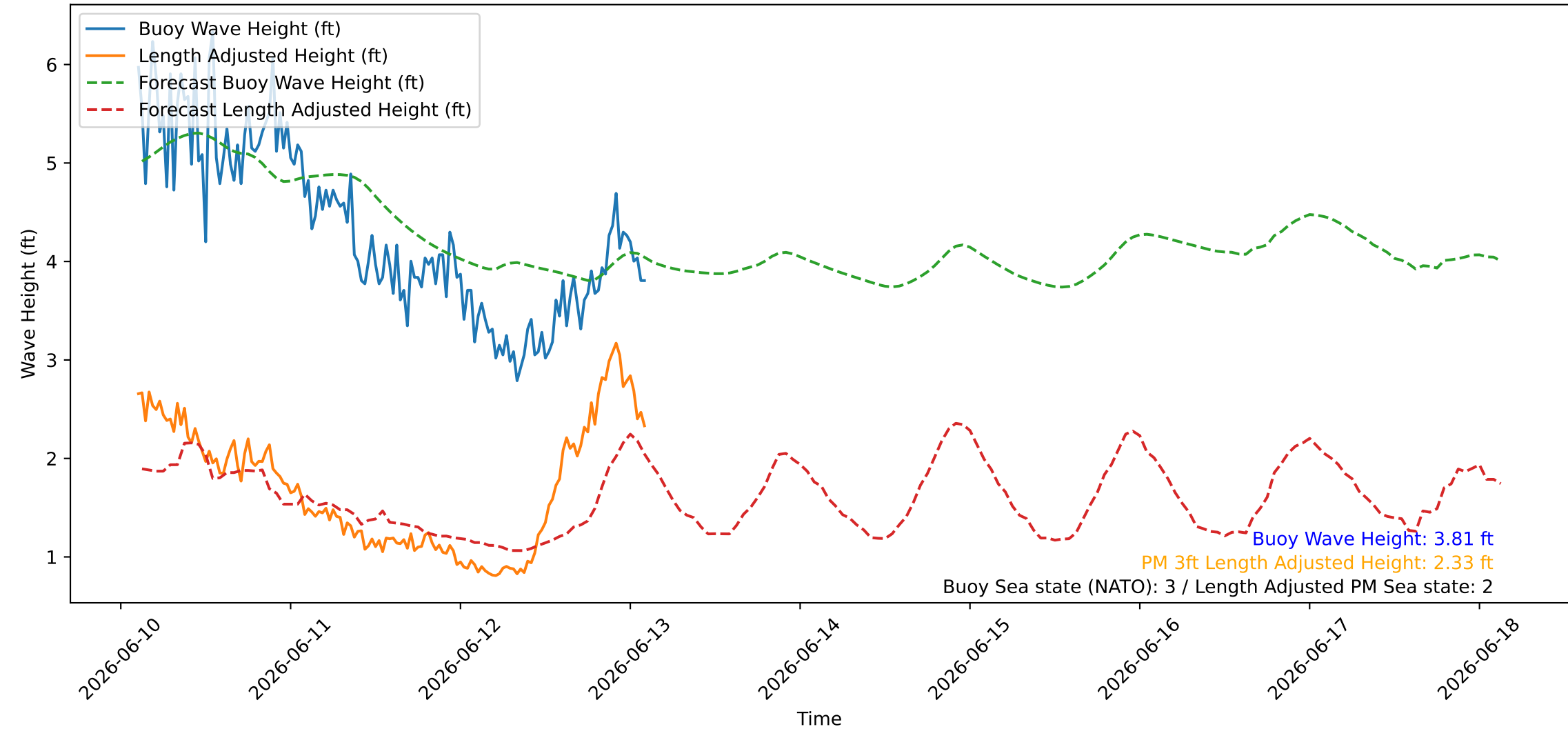
Wave Heights over Time for Oceanside Harbor at 2026-06-13 02:40:26
