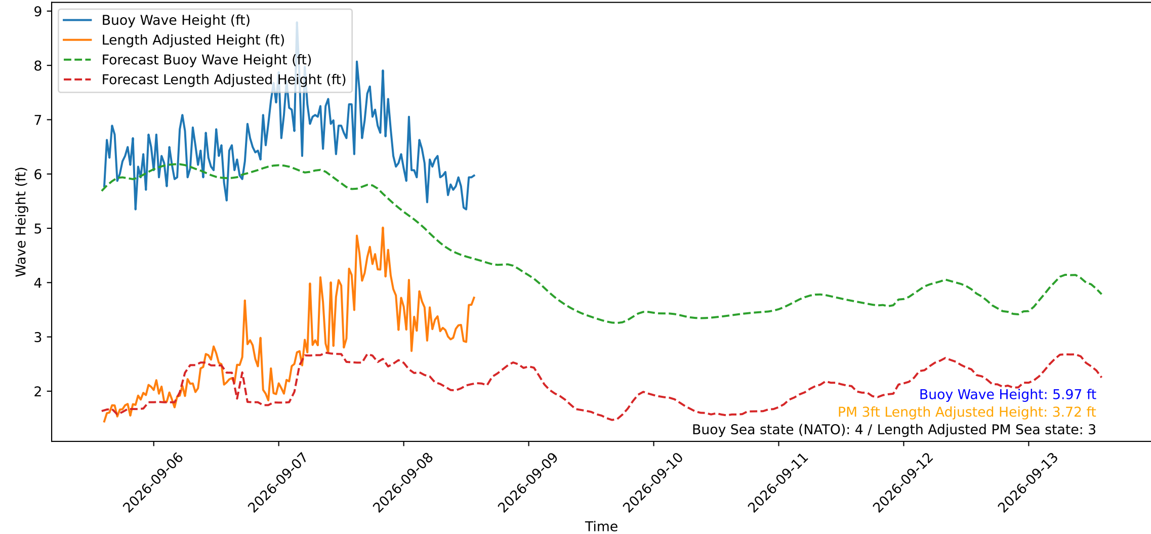
Wave Heights over Time for Green Beach at 2026-09-08 14:11:12
