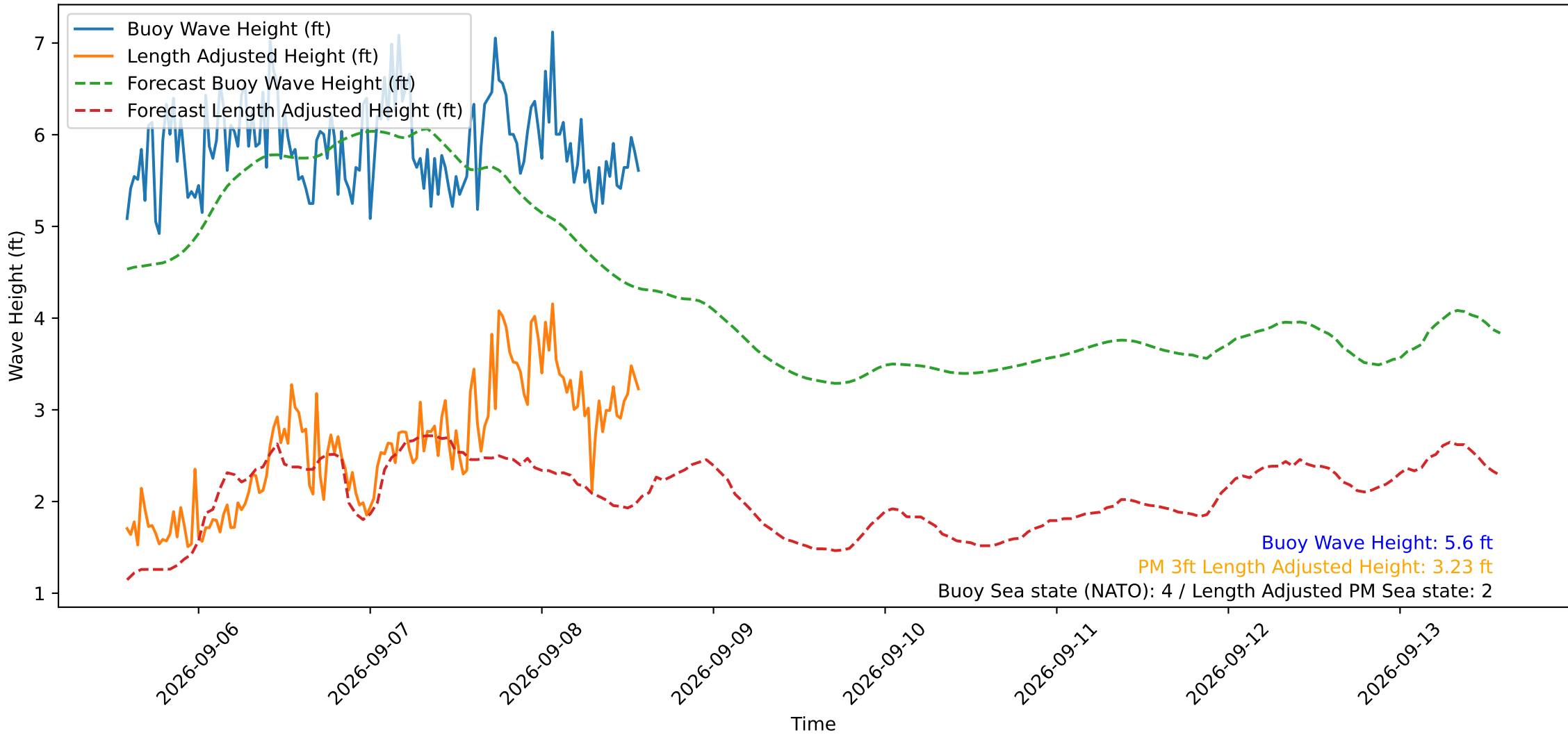
Wave Heights over Time for Oceanside Harbor at 2026-09-08 14:10:30
