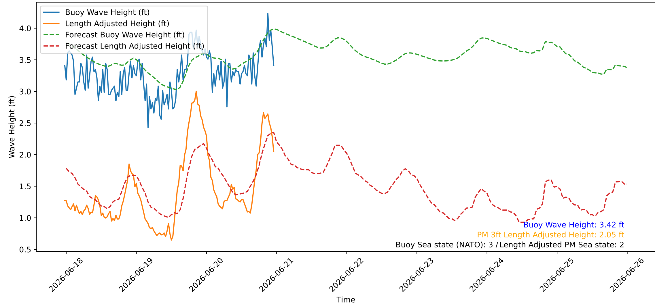
Wave Heights over Time for Green Beach at 2026-06-20 23:41:08
