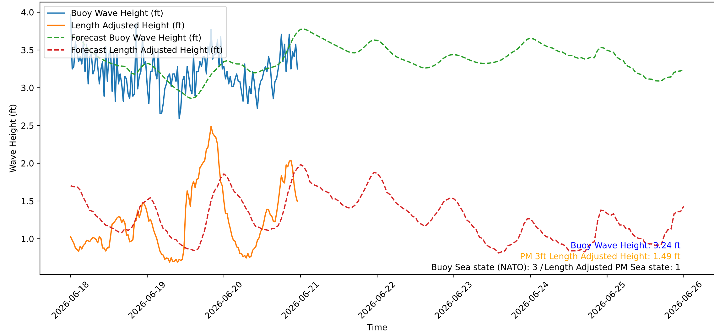
Wave Heights over Time for Red Beach at 2026-06-20 23:40:45
