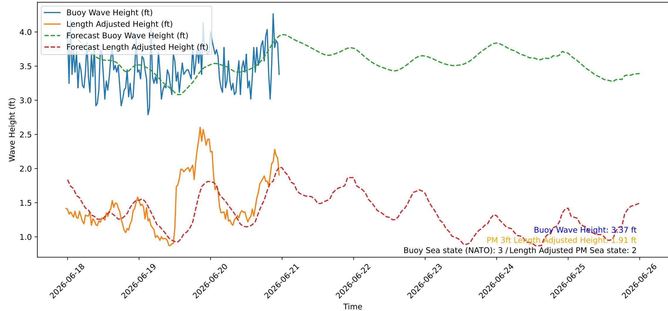
Wave Heights over Time for Oceanside Harbor at 2026-06-20 23:40:26
