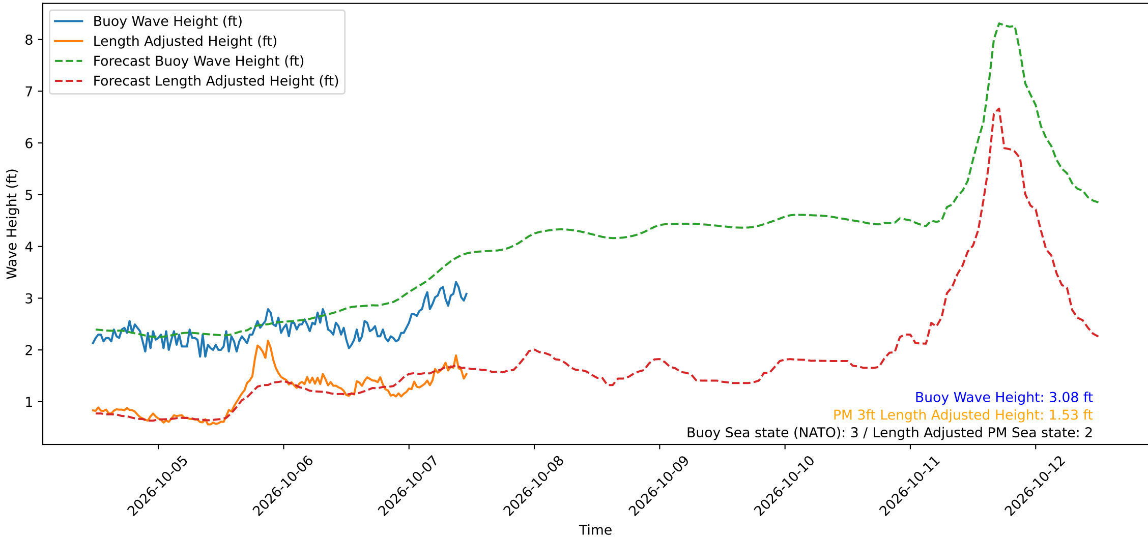
Wave Heights over Time for Oceanside Harbor at 2026-10-07 11:30:29
