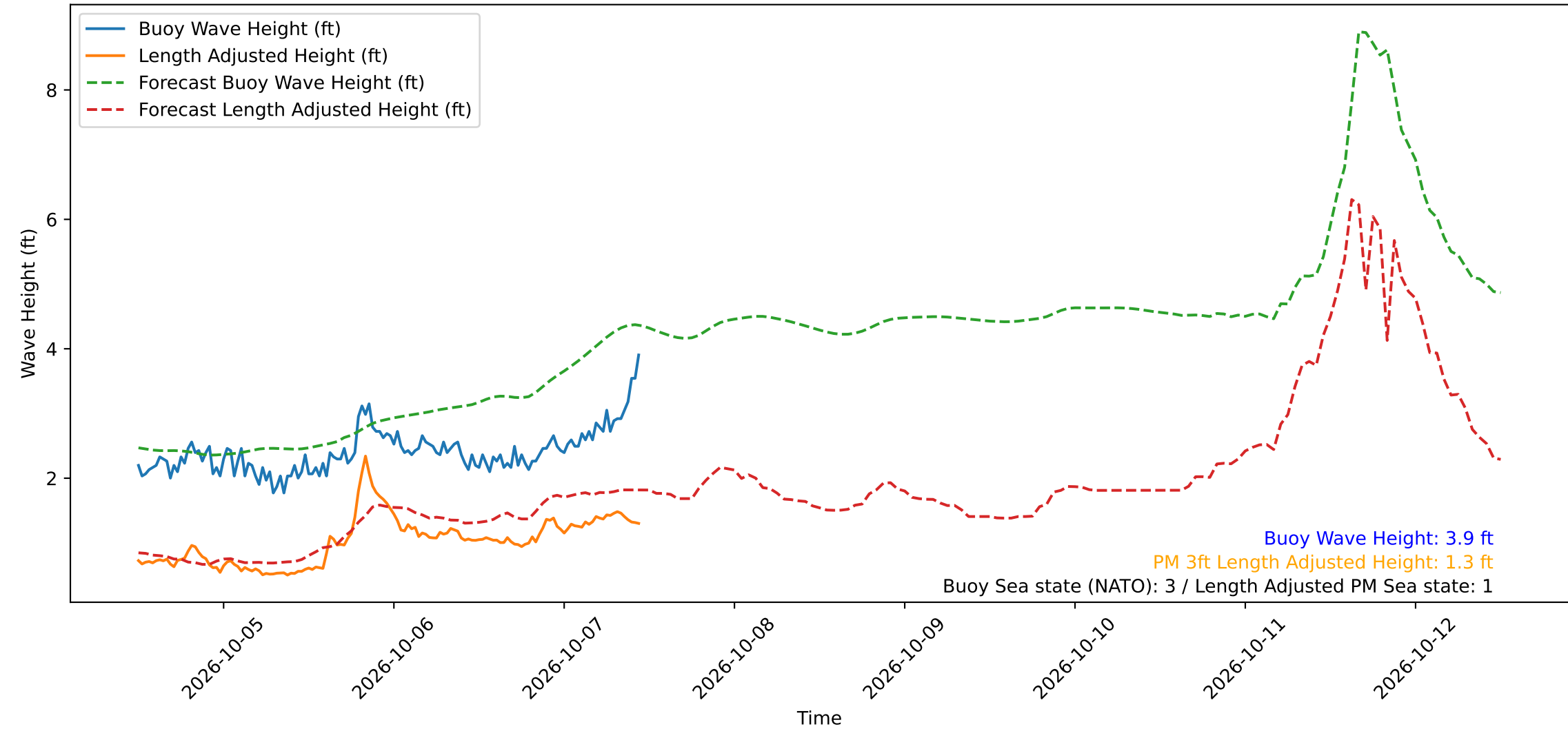
Wave Heights over Time for Green Beach at 2026-10-07 11:31:12
