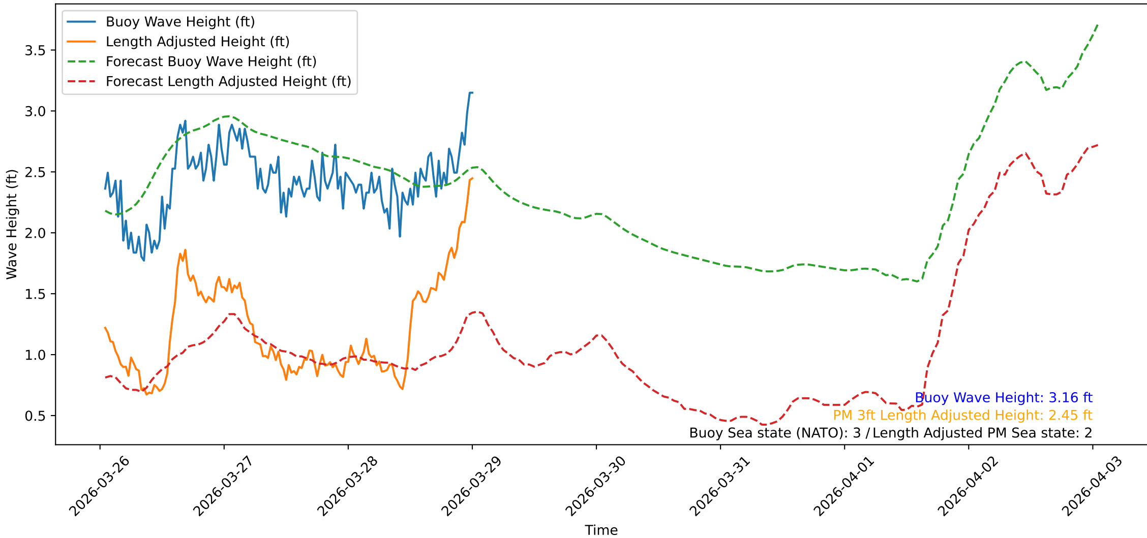
Wave Heights over Time for Oceanside Harbor at 2026-03-29 01:00:31
