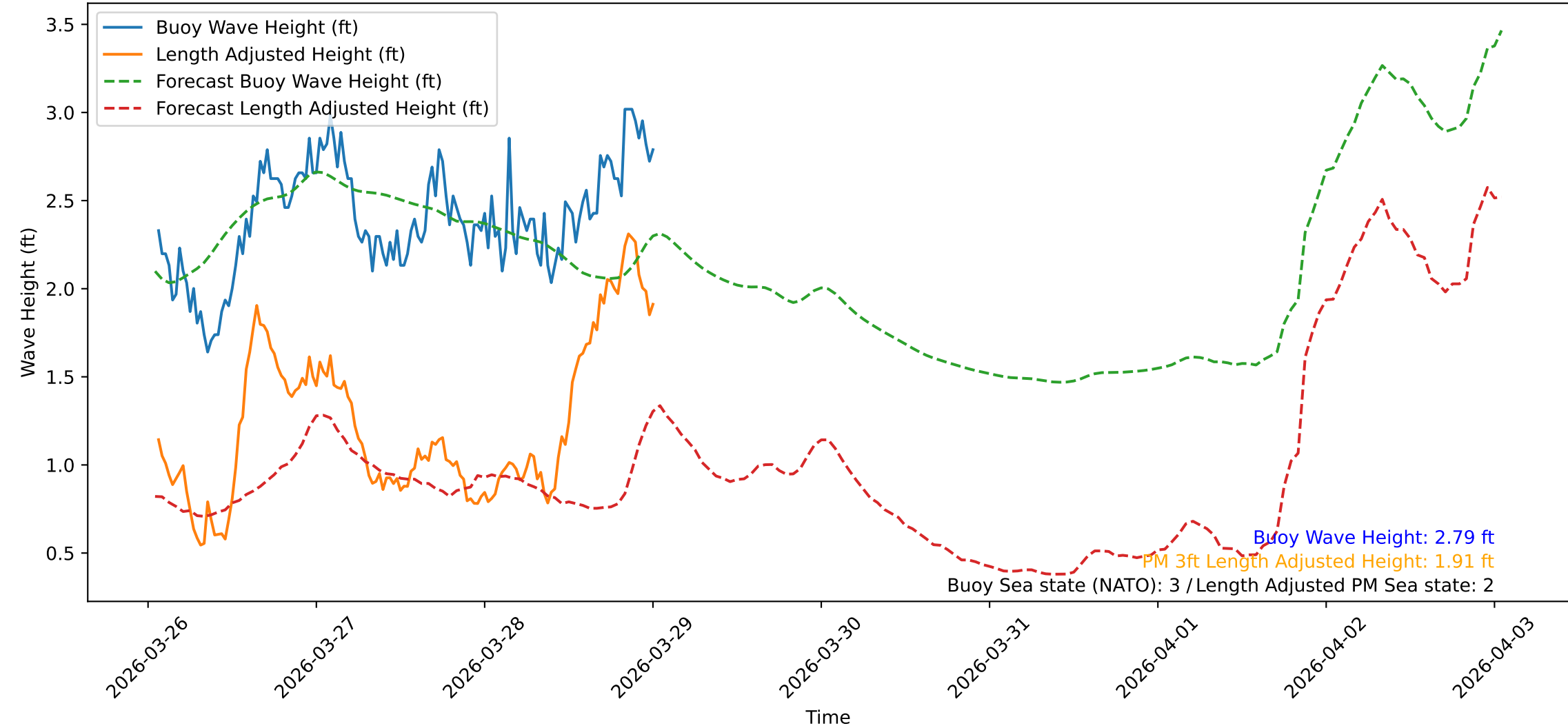
Wave Heights over Time for Red Beach at 2026-03-29 01:00:47
